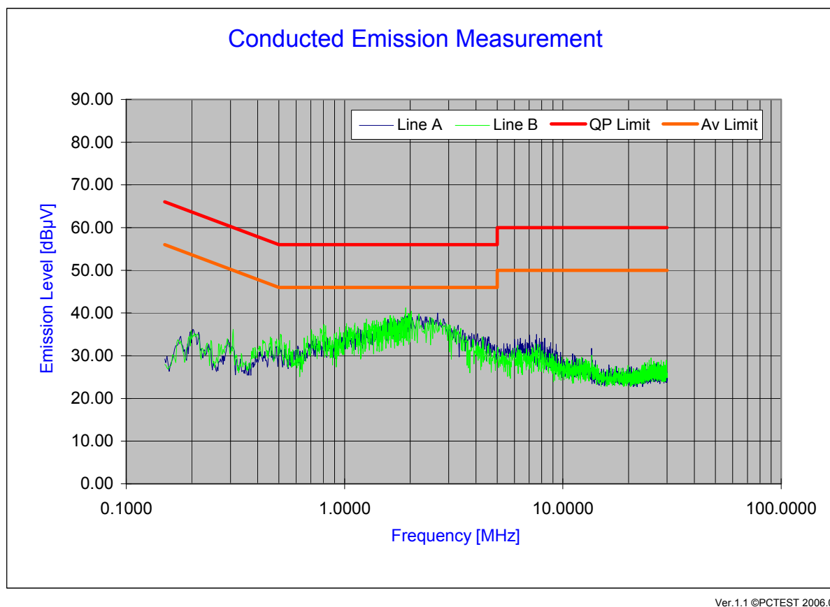
Plot 6-18. Line Conducted Plot with Bluetooth LE
