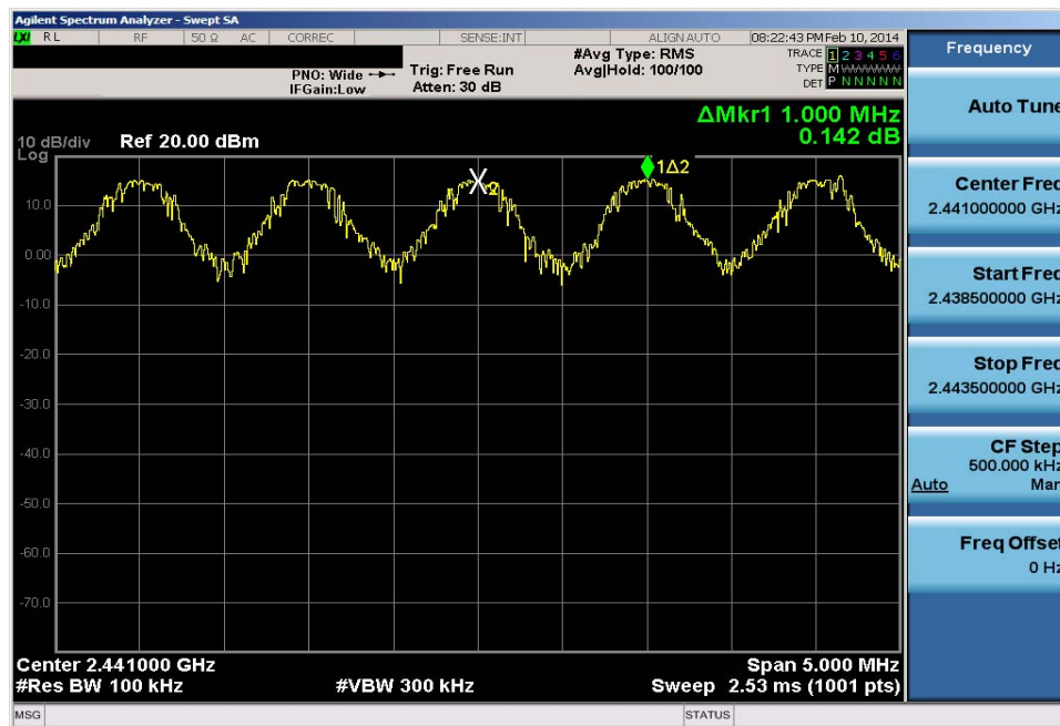
Plot 6-32. Channel Spacing Plot (Bluetooth)
