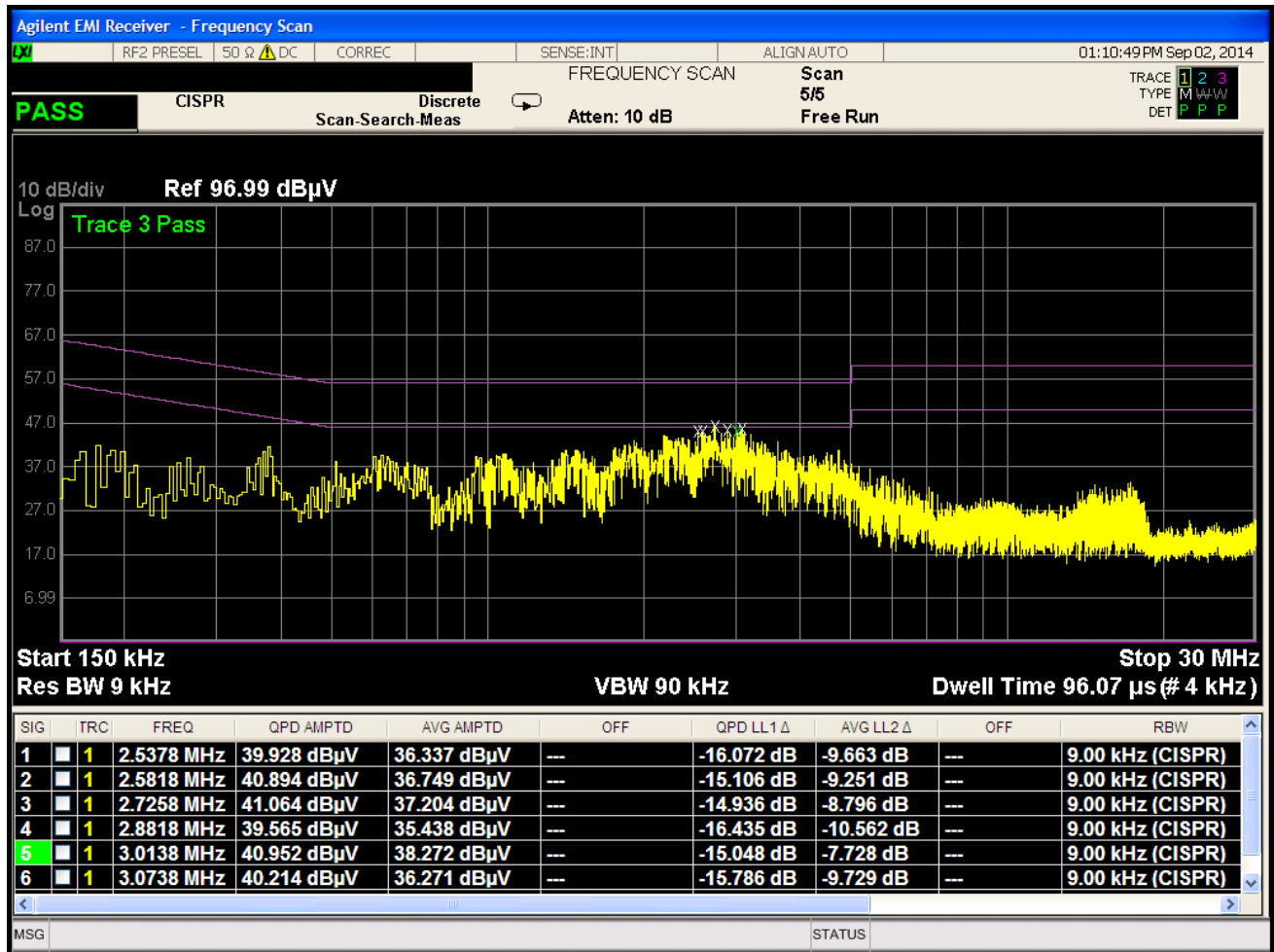
Plot 6-21. Line Conducted Plot and Data with Bluetooth LE (N)
