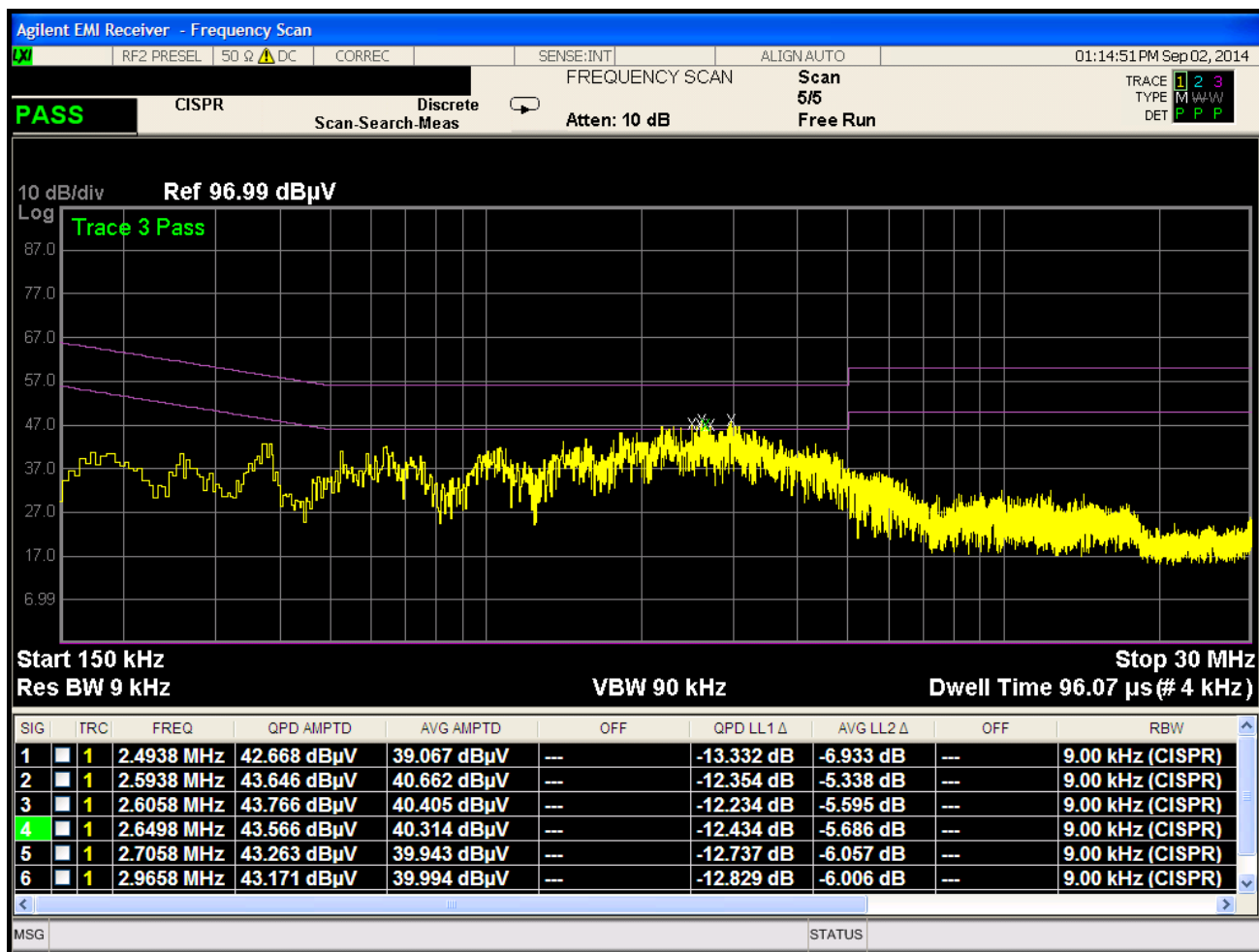
Plot 6-20. Line Conducted Plot and Data with Bluetooth LE (L1)
