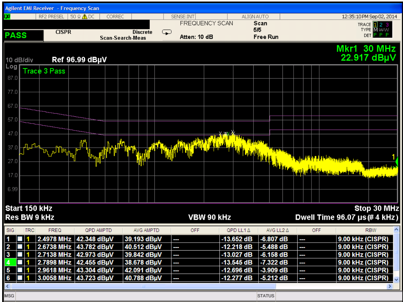
Plot 6-44. Line-Conducted Test Plot and Data (L1)
