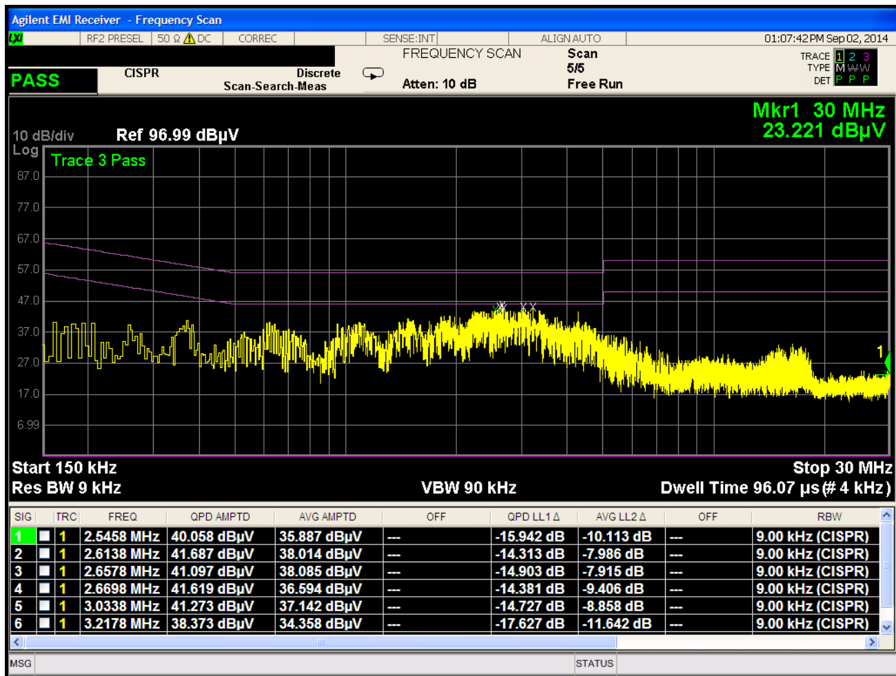
Plot 6-45. Line-Conducted Test Plot and Data (N)
