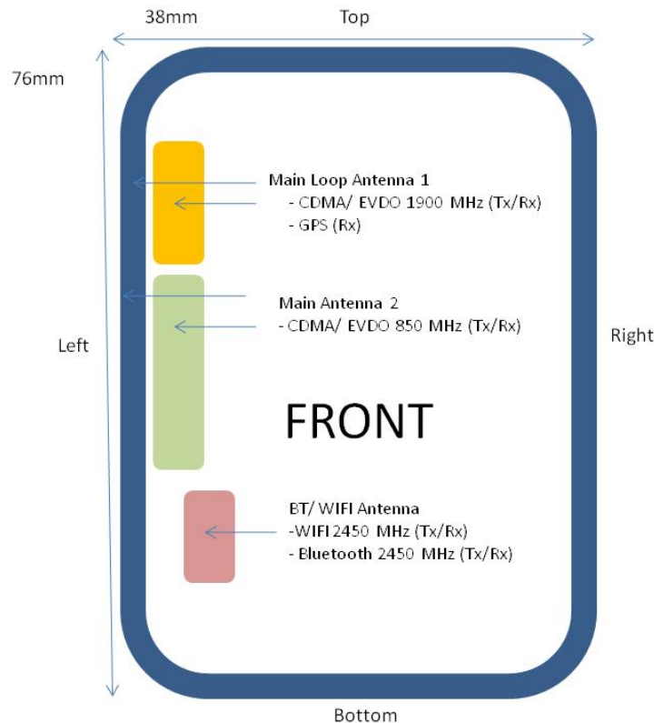
Figure 1-1 DUT Antenna Locations
