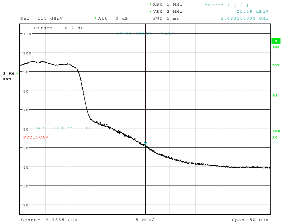
Plot 6-33. Radiated Restricted Upper Band Edge Measurement (Average)
