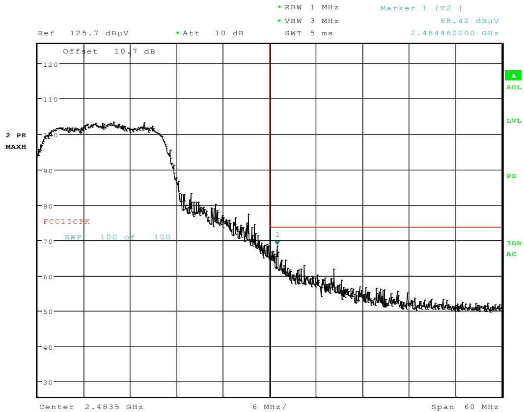
Plot 6-34. Radiated Restricted Upper Band Edge Measurement (Peak)
