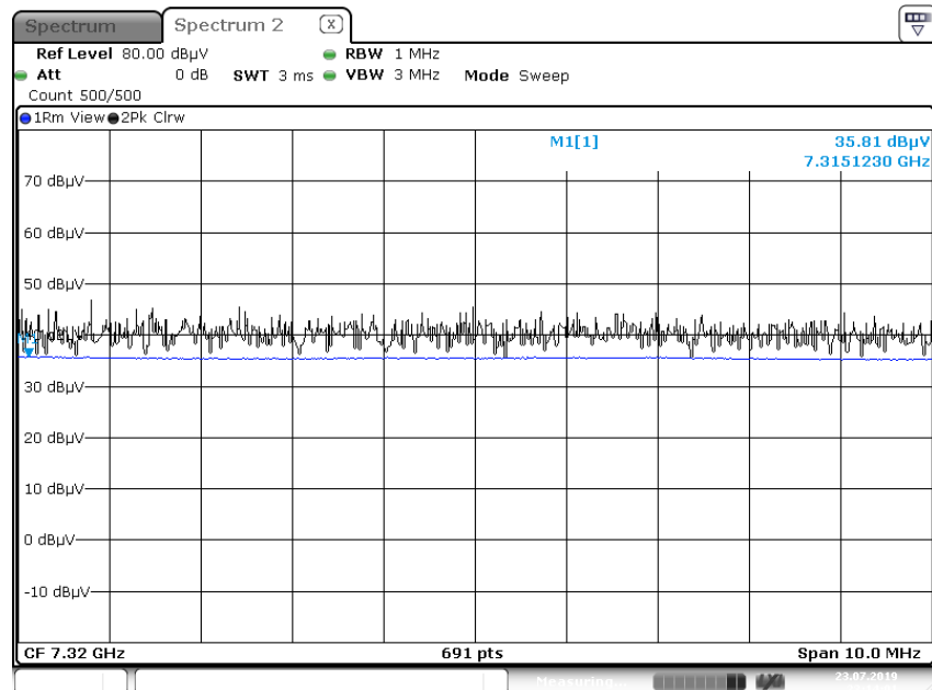
Radiated Spurious Emissions plot – Average Reading
