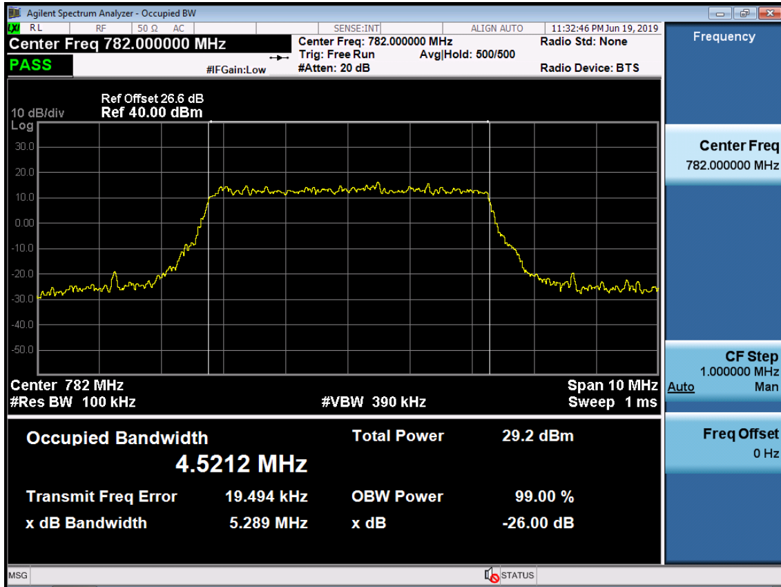
BAND 13. Occupied Bandwidth Plot (Ch.23230 16-QAM RB 25) 5 MHz
