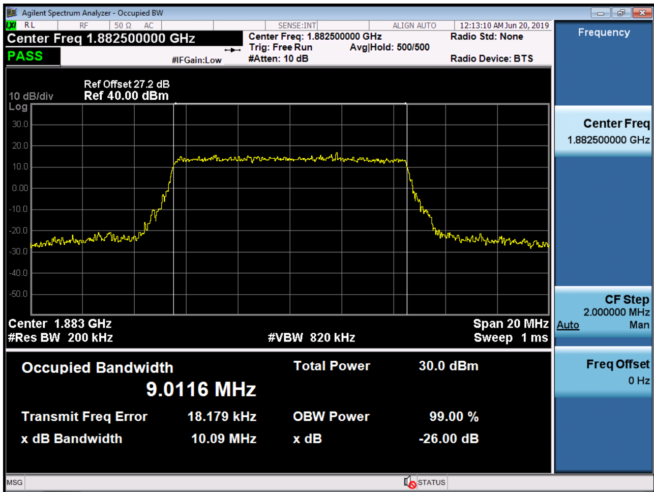
BAND 2. Occupied Bandwidth Plot (10M BW Ch.26365 QPSK RB 50_0)
