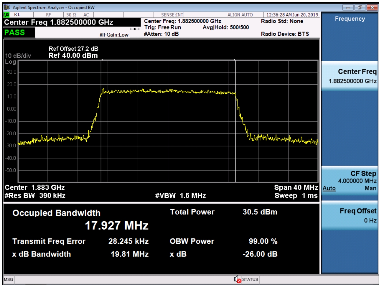
BAND 2. Occupied Bandwidth Plot (20M BW Ch.26365 QPSK RB 100_0)
