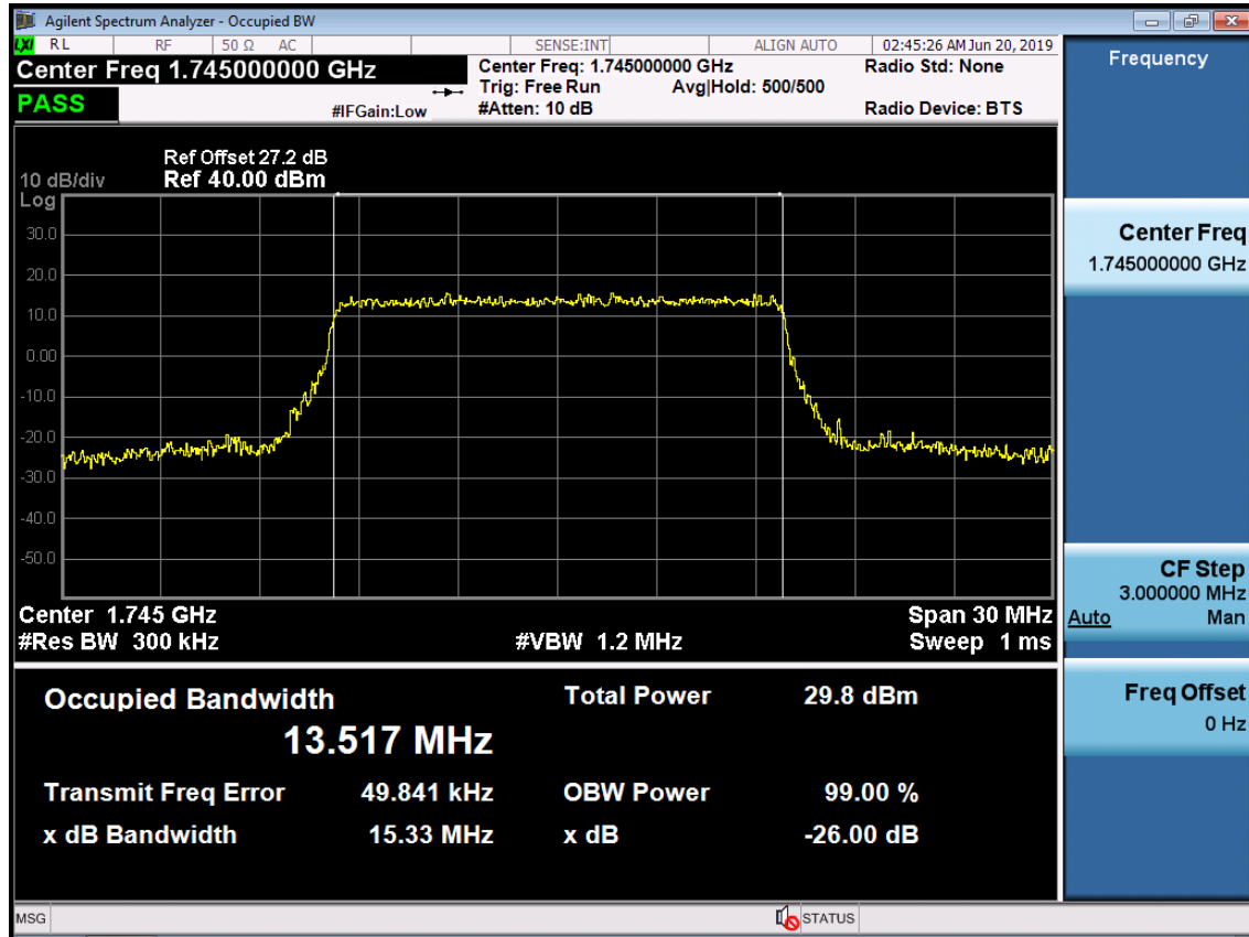
BAND 66. Occupied Bandwidth Plot (15M BW Ch.132322 QPSK RB 75)
