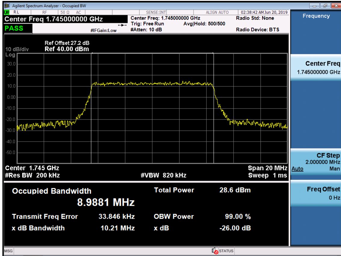
BAND 66. Occupied Bandwidth Plot (10M BW Ch.132322 16QAM RB 50)
