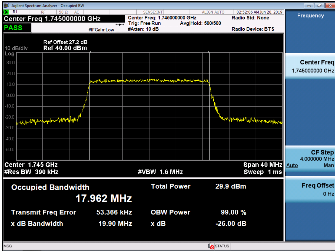
BAND 66, Occupied Bandwidth Plot (20M BW Ch.132322 QPSK RB 100)
