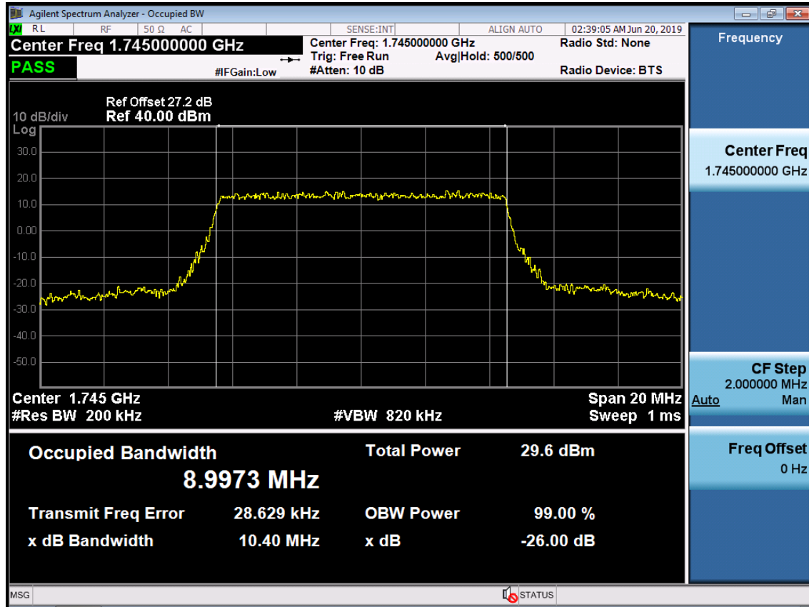
BAND 66. Occupied Bandwidth Plot (10M BW Ch.132322 QPSK RB 50)
