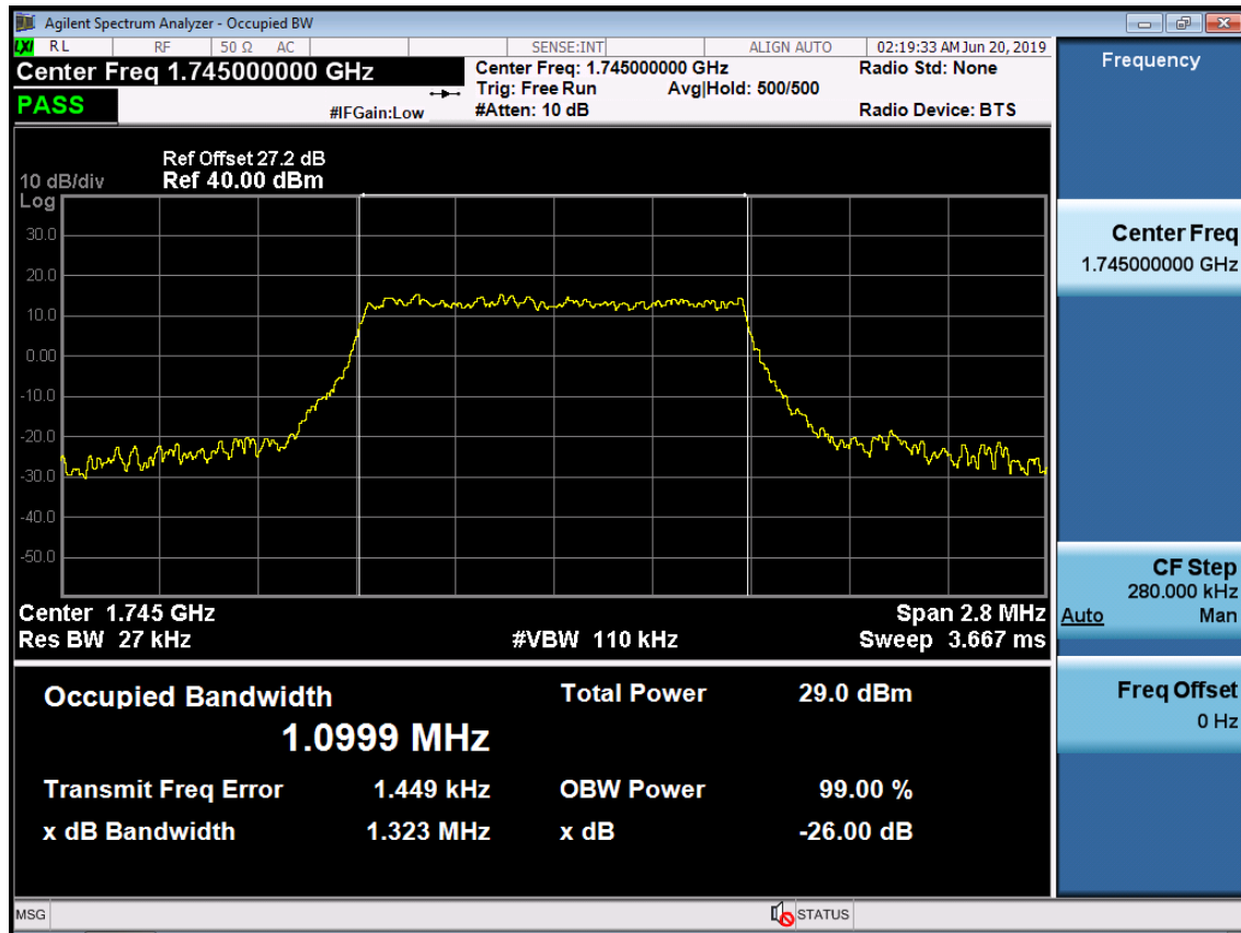
BAND 66. Occupied Bandwidth Plot (1.4M BW Ch.132322 16QAM RB 6)
