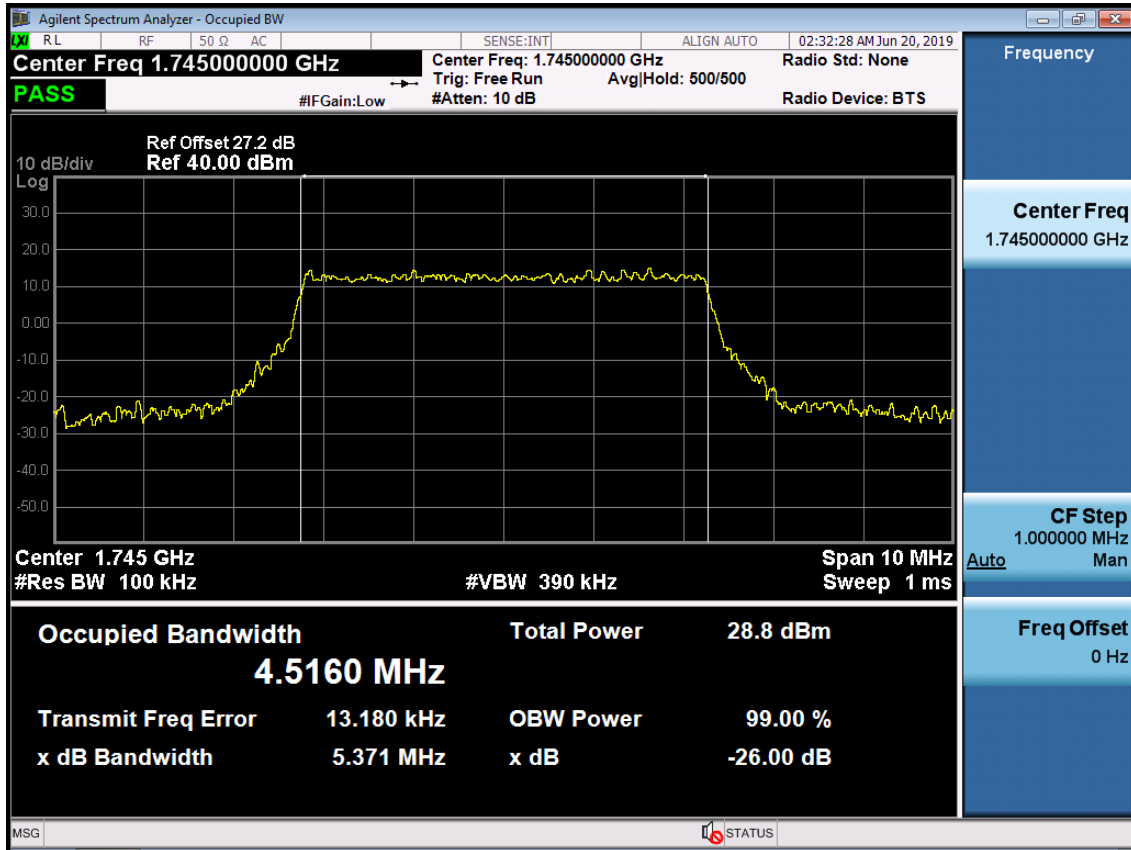
BAND 66. Occupied Bandwidth Plot (5M BW Ch.132322 16QAM RB 25)
