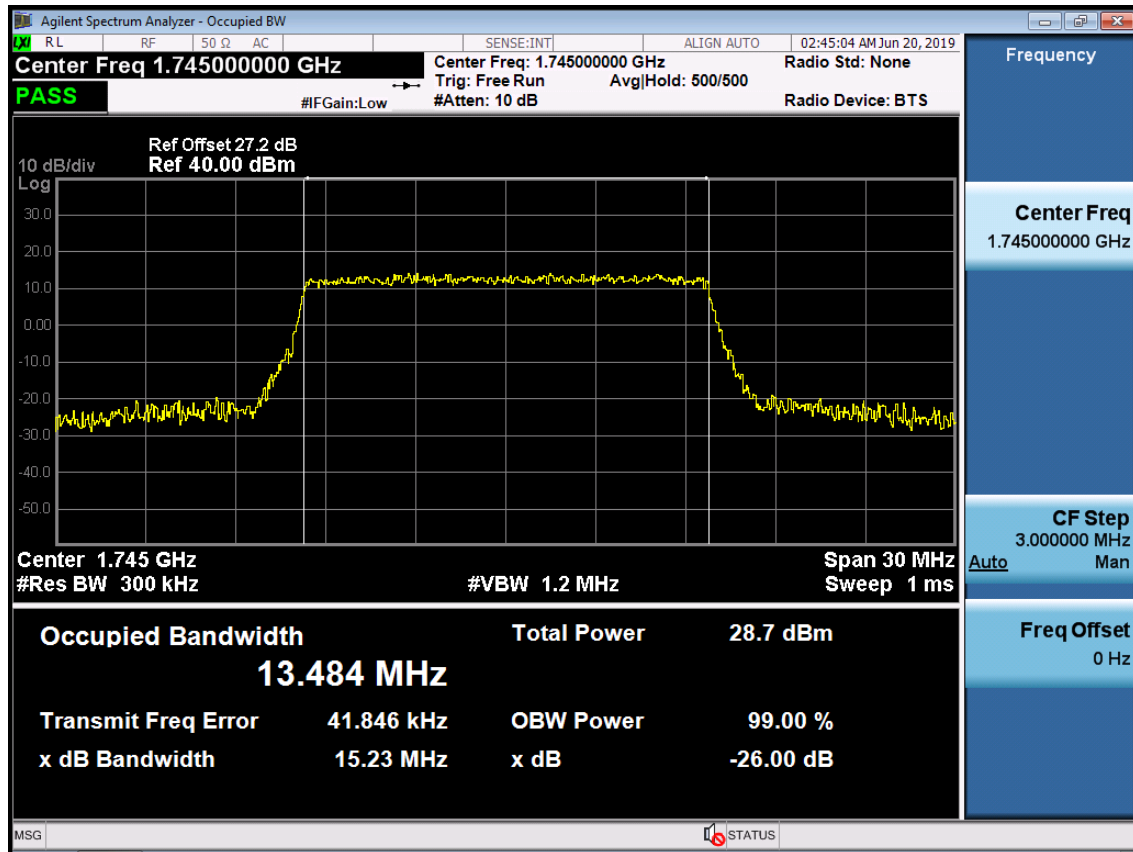
BAND 66. Occupied Bandwidth Plot (15M BW Ch.132322 16QAM RB 75)
