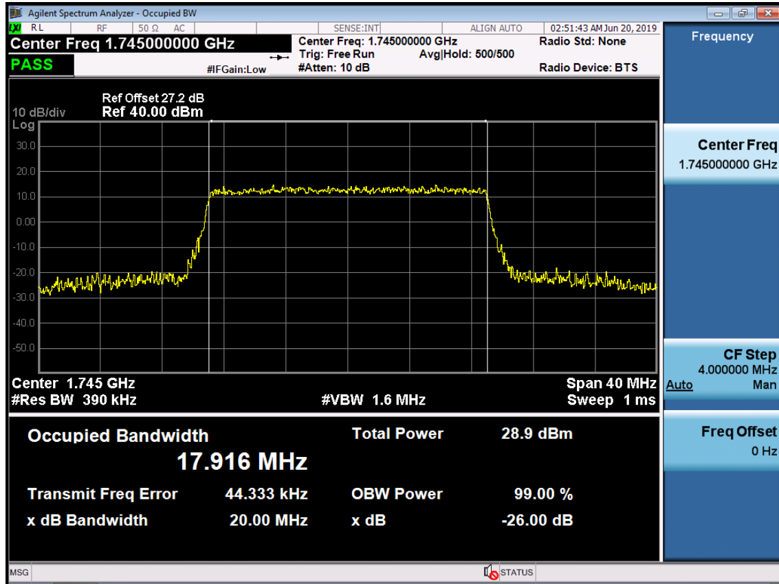
BAND 66. Occupied Bandwidth Plot (20M BW Ch.132322 16QAM RB 100)
