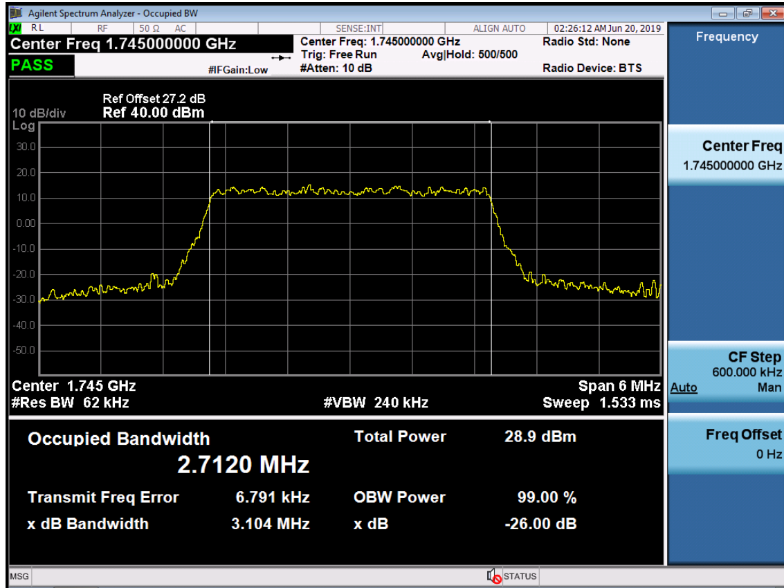
BAND 66. Occupied Bandwidth Plot (3M BW Ch.132322 16QAM RB 15)
