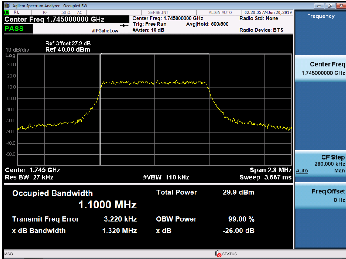
BAND 66. Occupied Bandwidth Plot (1.4M BW Ch.132322 QPSK RB 6)
