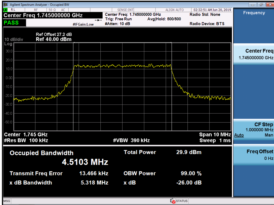
BAND 66. Occupied Bandwidth Plot (5M BW Ch.132322 QPSK RB 25)
