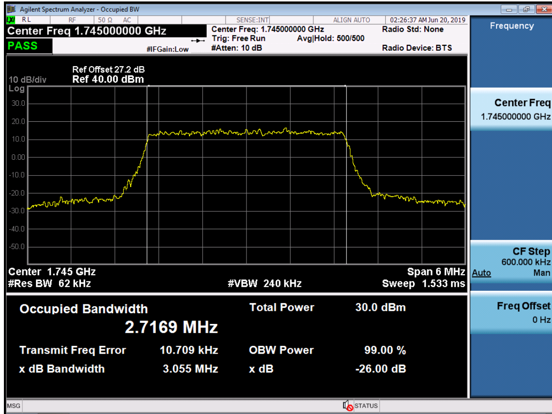
BAND 66. Occupied Bandwidth Plot (3M BW Ch.132322 QPSK RB 15)
