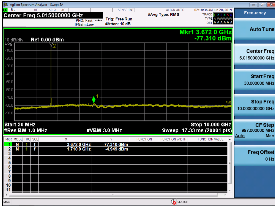
BAND 66. Conducted Spurious Plot_1 (131979ch_1.4MHz_QPSK_RB 1_0)
