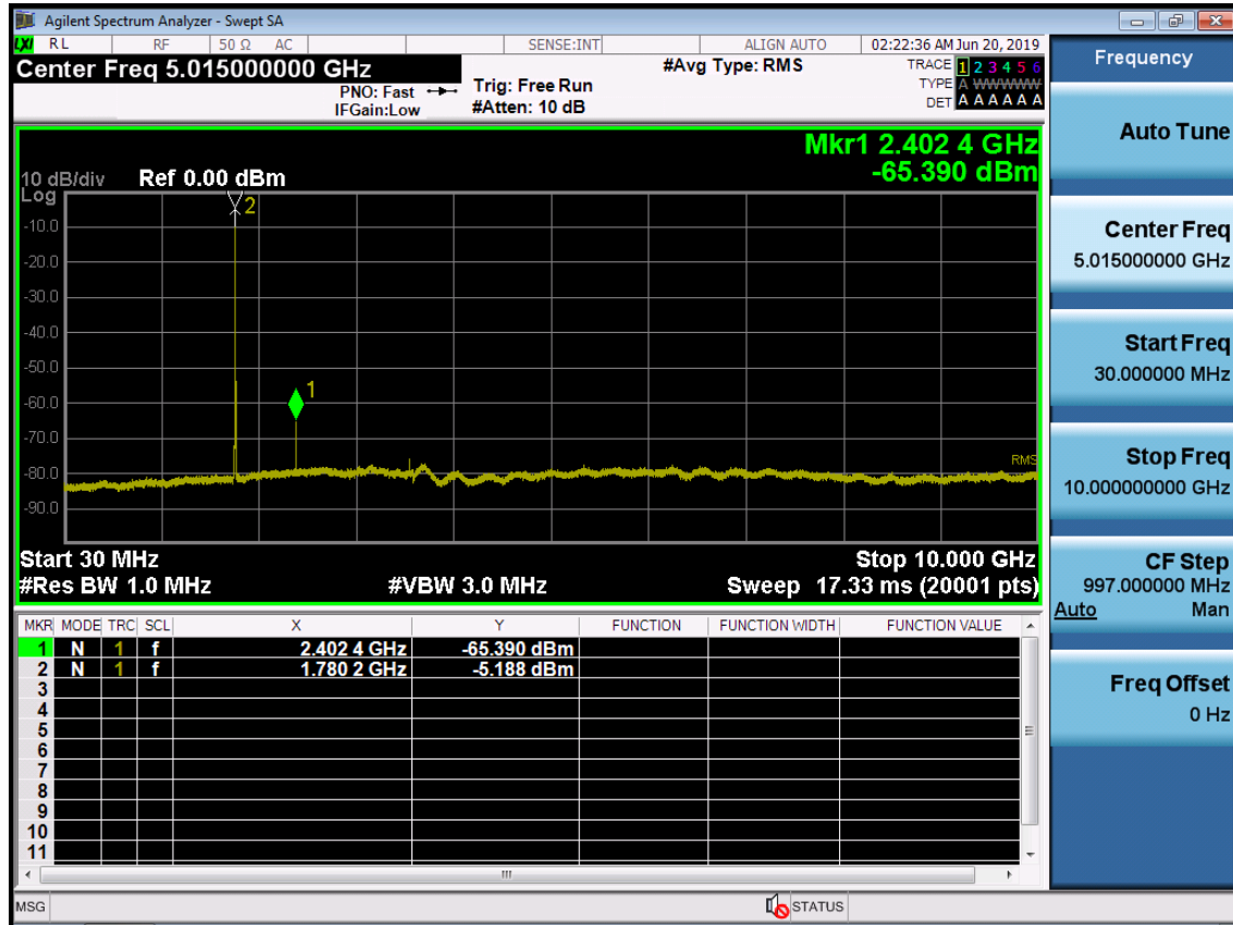
BAND 66. Conducted Spurious Plot_1 (132665ch_1.4MHz_QPSK_ RB 1_0)
