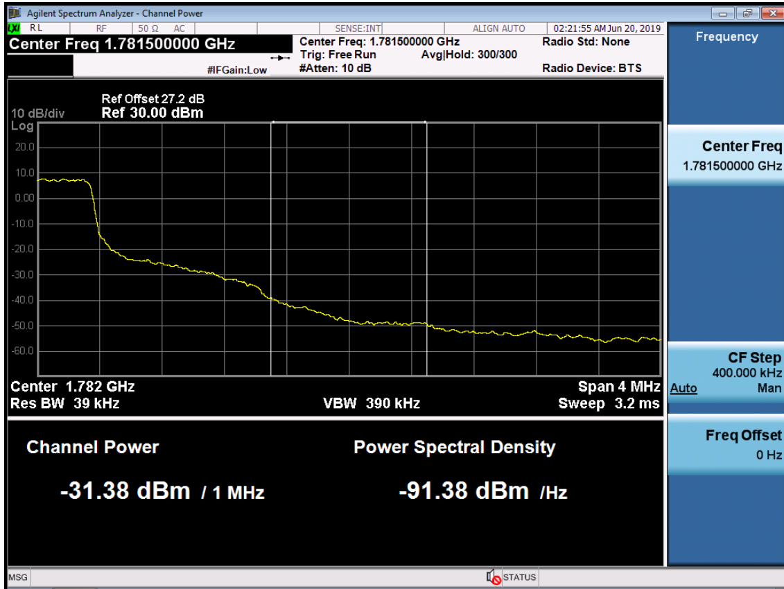
BAND 66. Upper Extended Band Edge Plot (1.4M BW Ch. 132665 QPSK_RB6_0) -3
