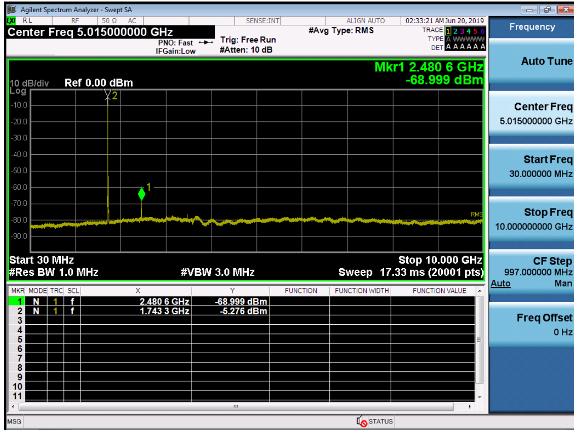
BAND 66. Conducted Spurious Plot_1 (132322ch_5MHz_QPSK_RB 1_0)
