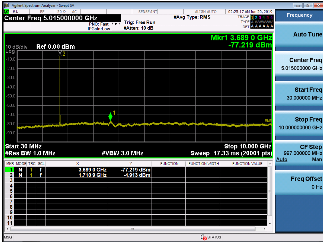
BAND 66. Conducted Spurious Plot_1 (131987ch_3MHz_QPSK_RB 1_0)
