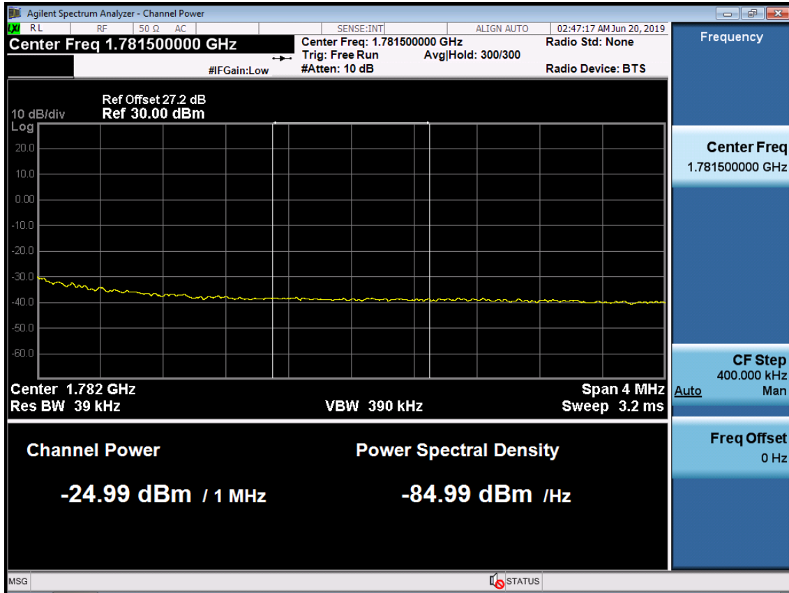
BAND 66. Upper Extended Band Edge Plot (15M BW Ch.132597 QPSK_RB75) -3
