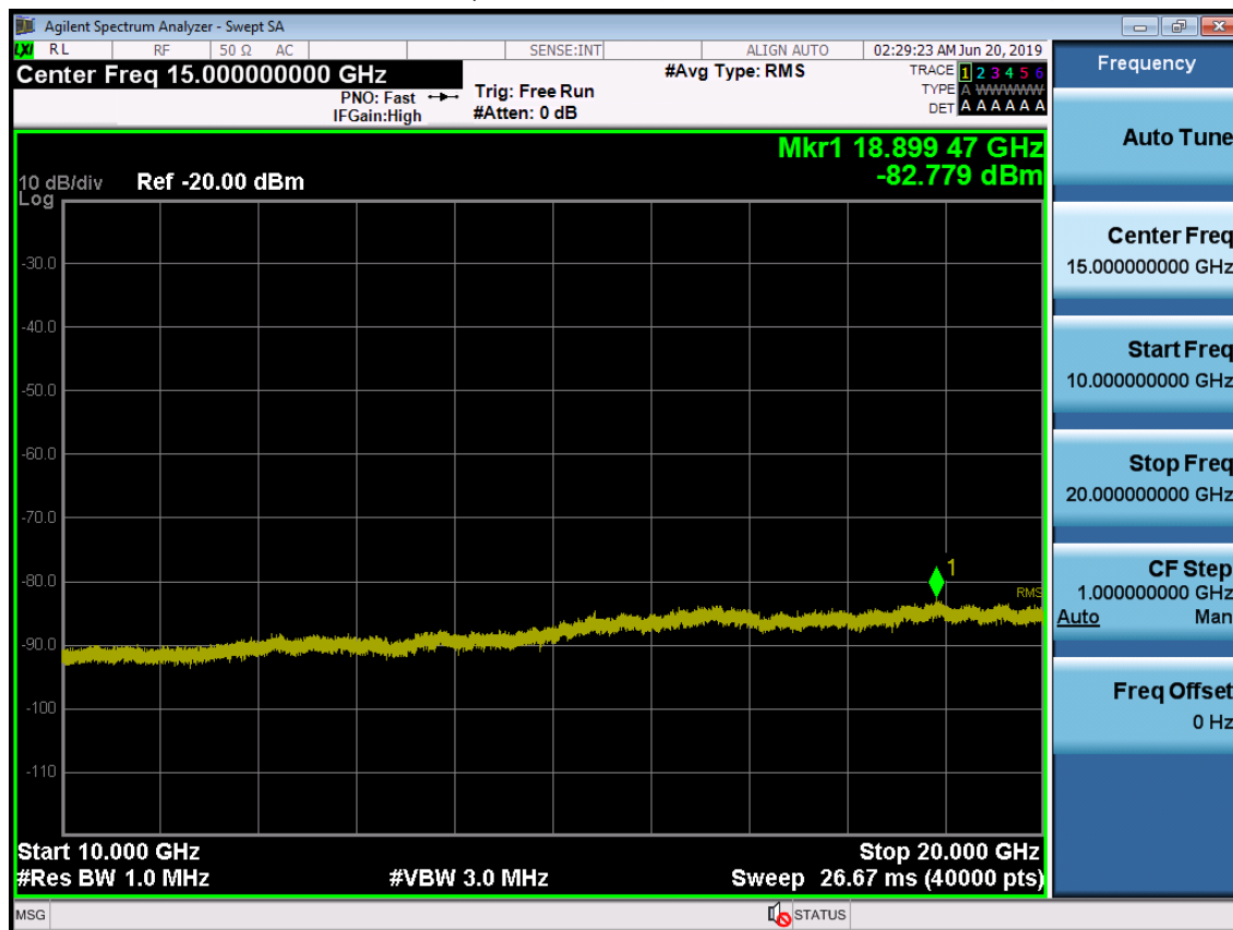
BAND 66. Conducted Spurious Plot_2 (132657ch_3MHz_QPSK_RB 1_0)
