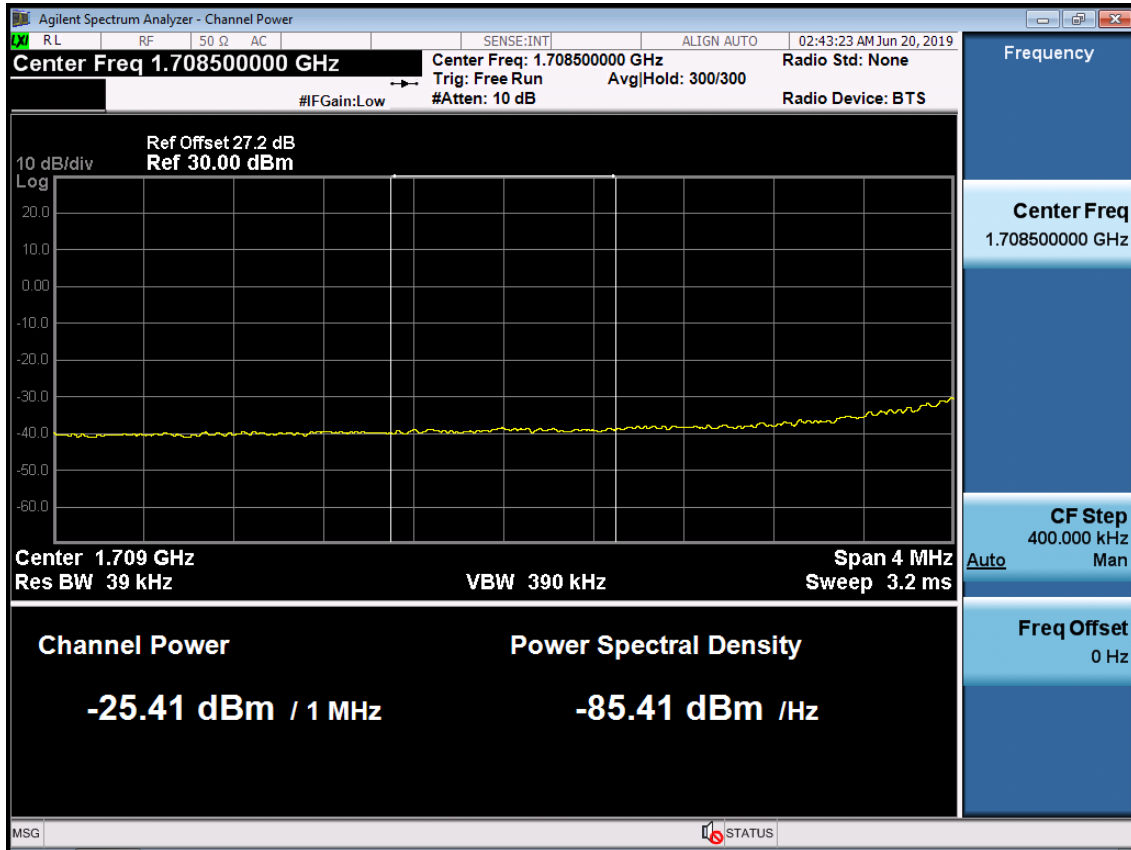
BAND 66. Lower Extended Band Edge Plot (15M BW Ch.132047 QPSK_RB75_0) -3
