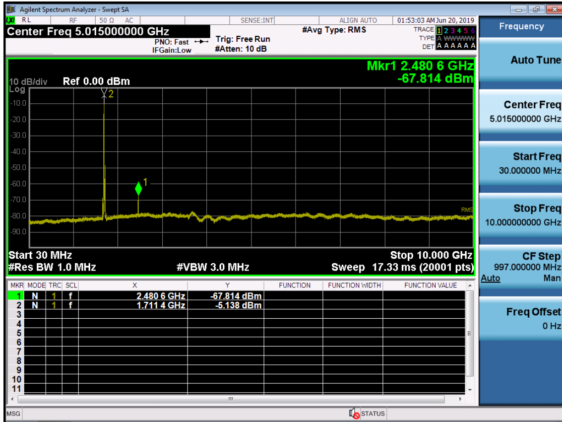
BAND 66. Conducted Spurious Plot_1 (132047ch_15MHz_QPSK_ RB 1_0)
