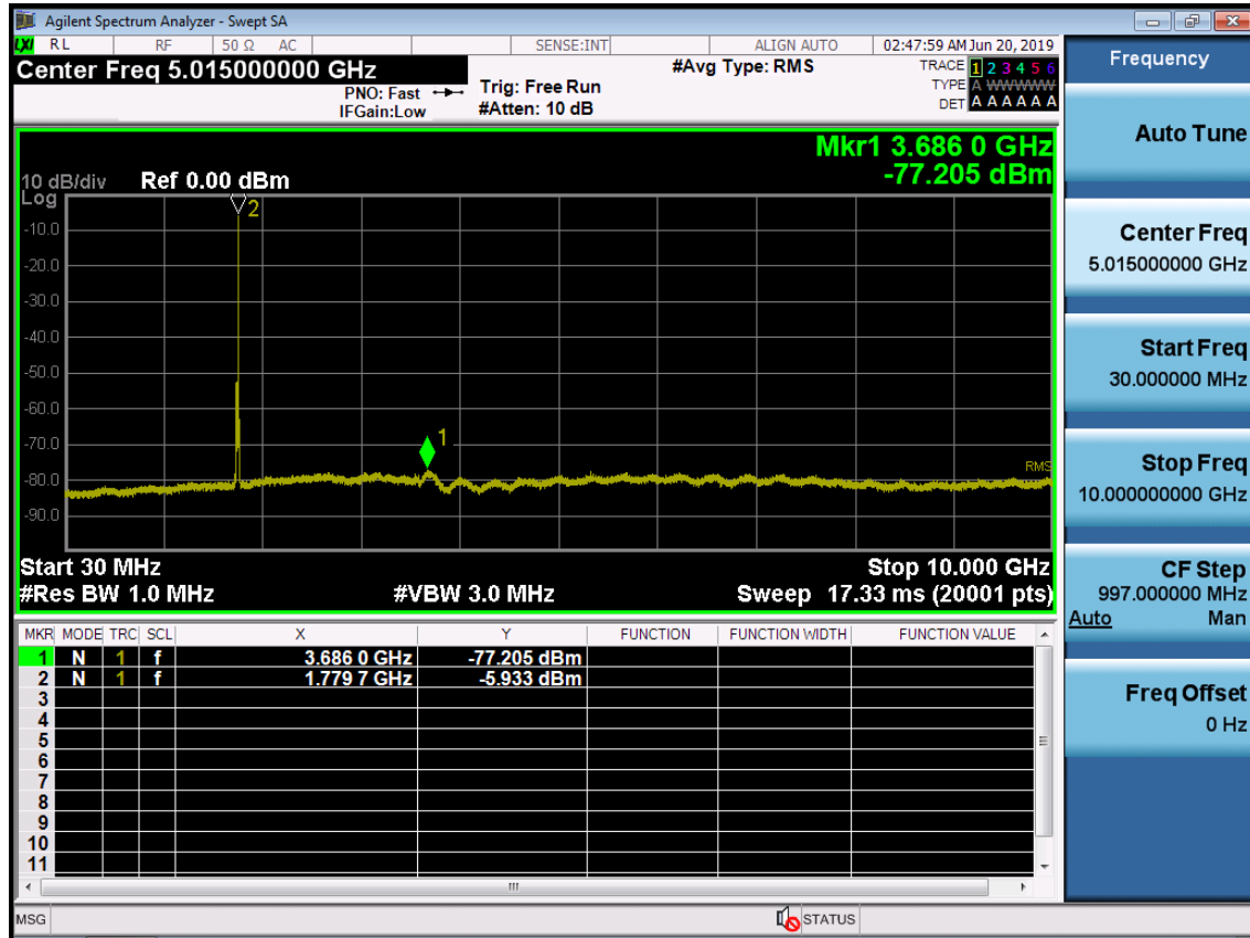
BAND 66. Conducted Spurious Plot_1 (132597ch_15MHz_QPSK_ RB 1_0)
