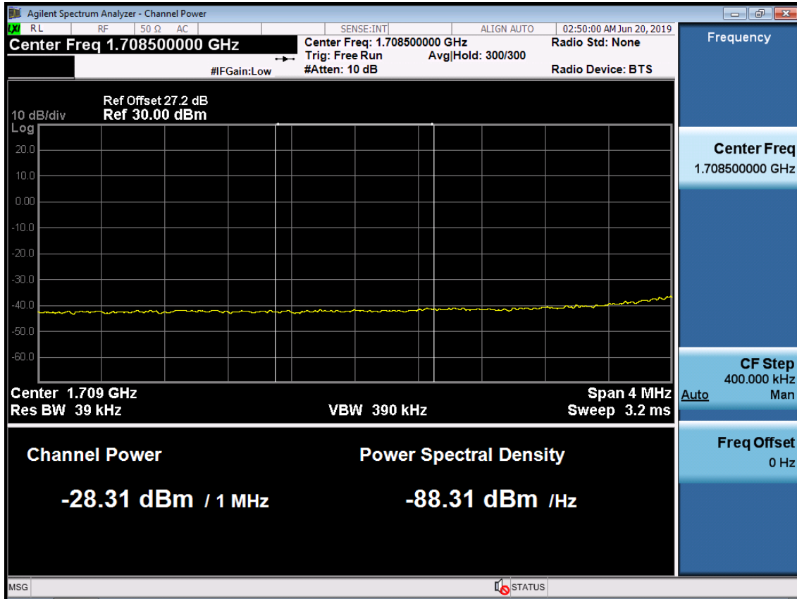
BAND 66. Lower Extended Band Edge Plot (20M BW Ch.132072 QPSK_RB100_0) -3
