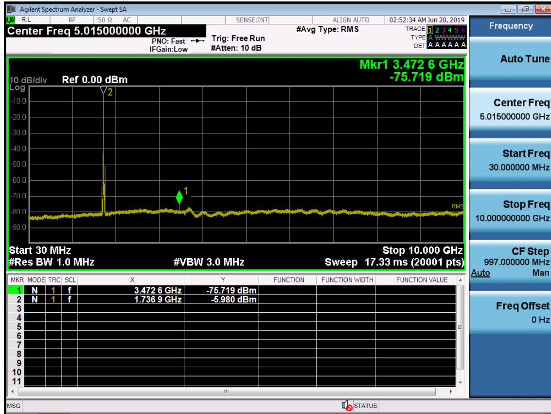
BAND 66. Conducted Spurious Plot_1 (132322ch_20MHz_QPSK_ RB 1_0)
