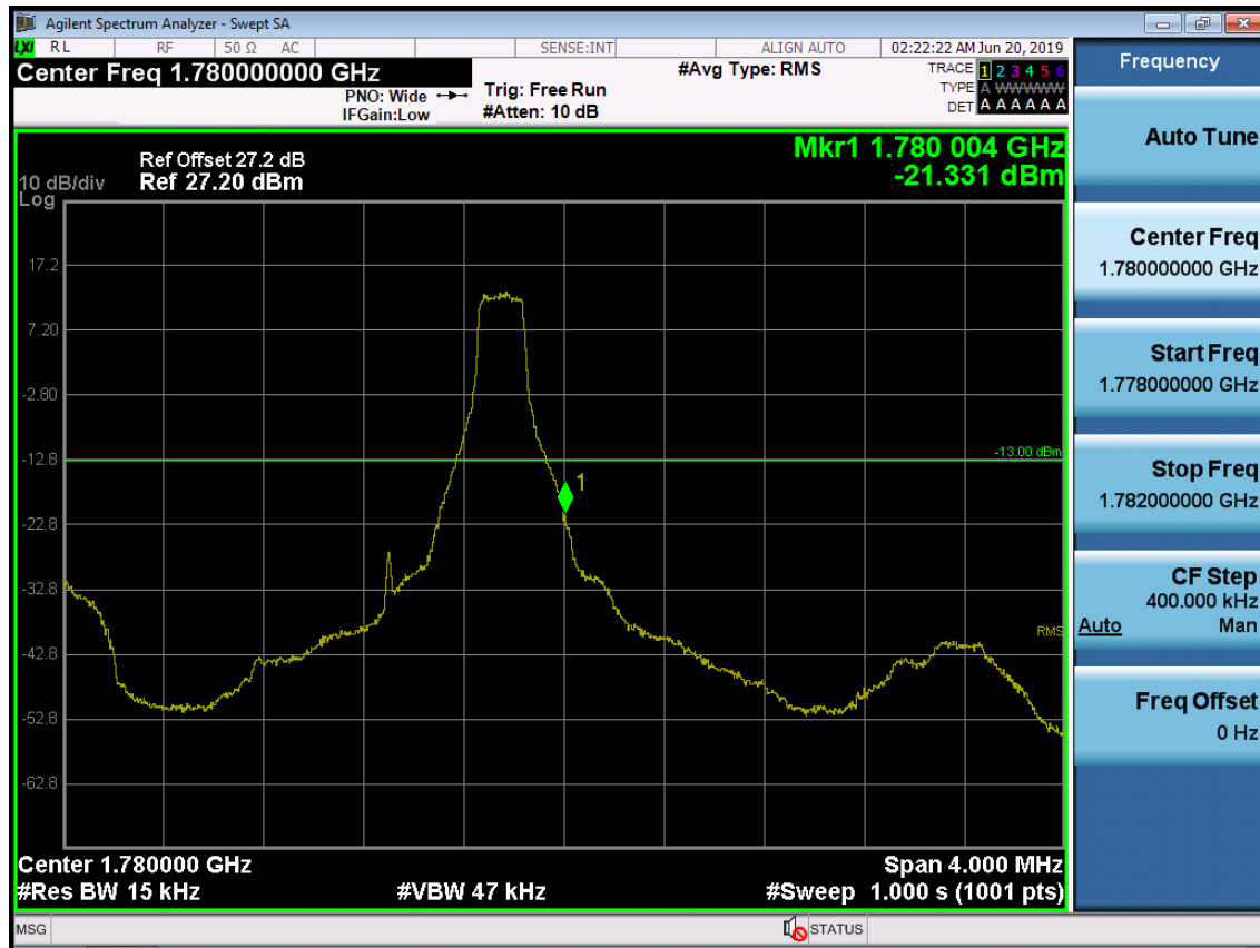
BAND 66. Upper Band Edge Plot (1.4M BW Ch.132665 QPSK_RB1_Offset5) -1
