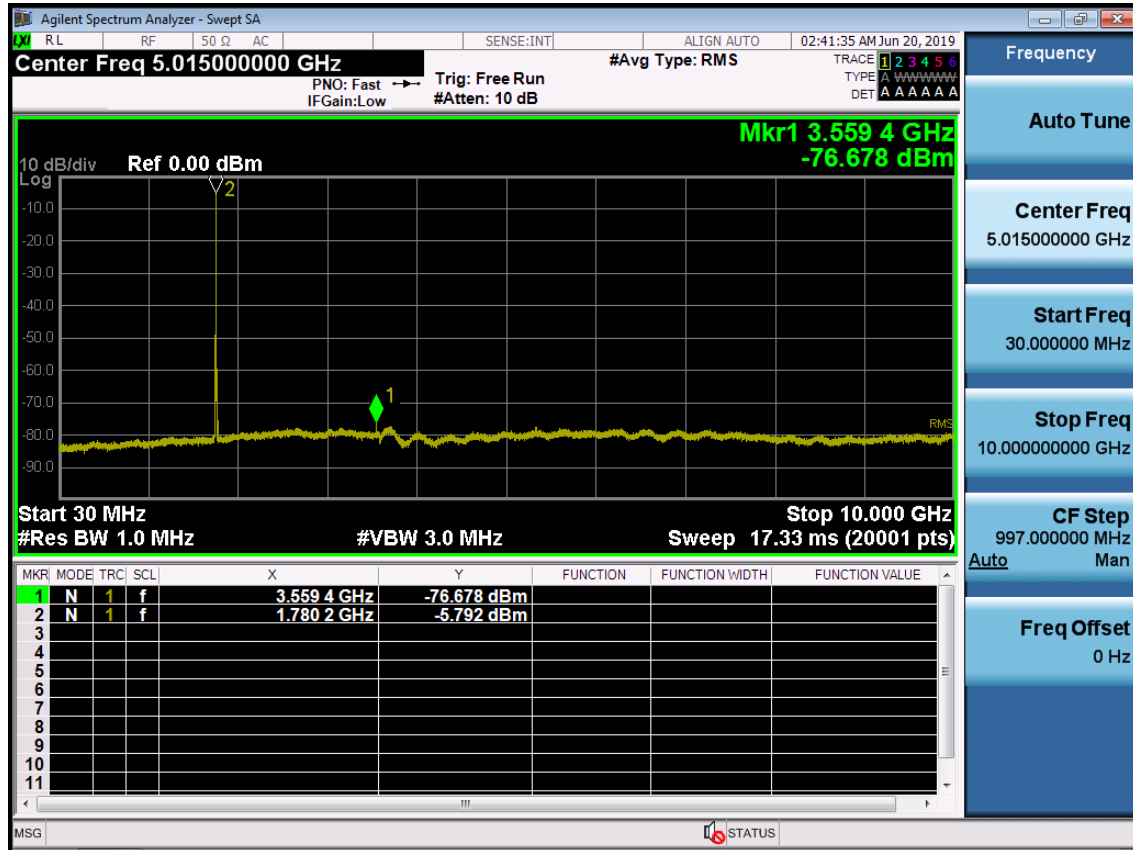
BAND 66. Conducted Spurious Plot_1 (132622ch_10MHz_QPSK_ RB 1_0)
