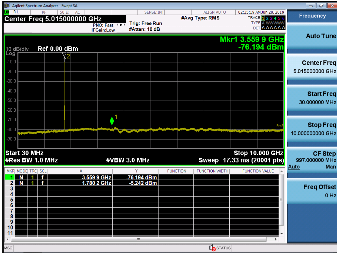
BAND 66. Conducted Spurious Plot_1 (132647ch_5MHz_QPSK_RB 1_0)
