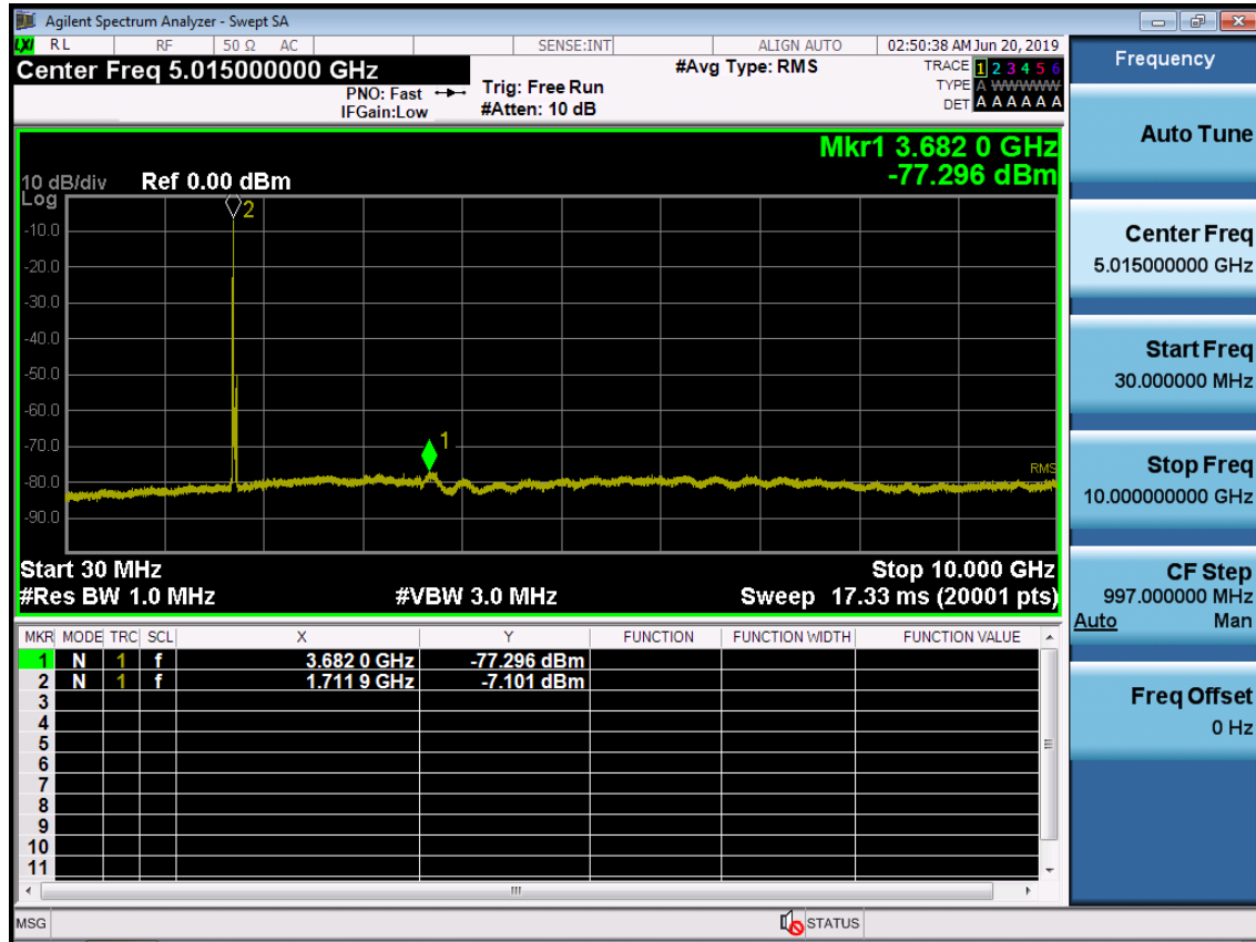
BAND 66. Conducted Spurious Plot_1 (132072ch_20MHz_QPSK_ RB 1_0)
