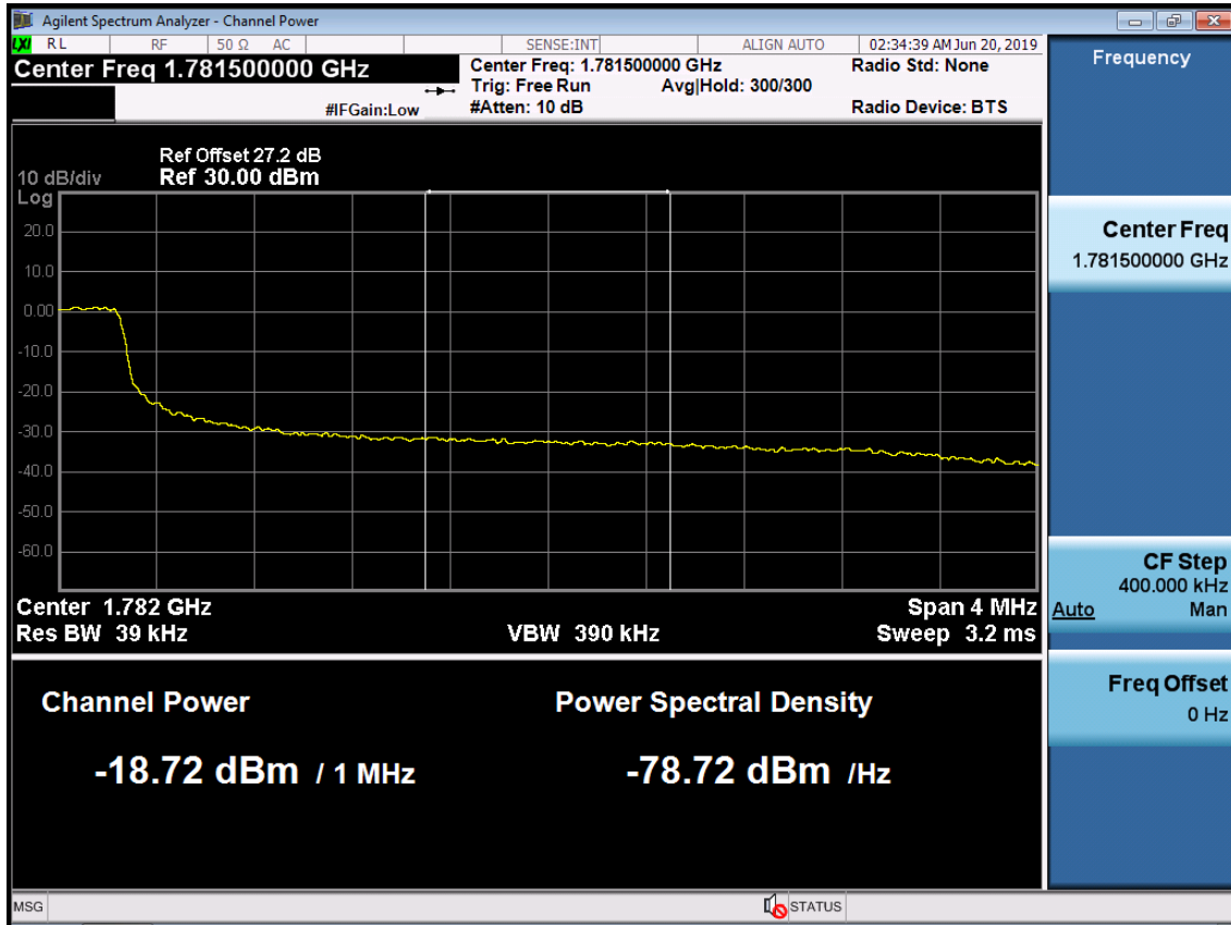
BAND 66. Upper Extended Band Edge Plot (5M BW Ch.132647 QPSK_RB25) -3
