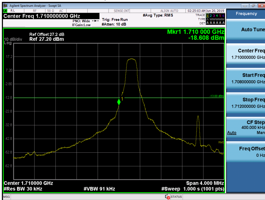
BAND 66. Lower Band Edge Plot (3M BW Ch.131987 QPSK RB 1, Offset 0) -1
