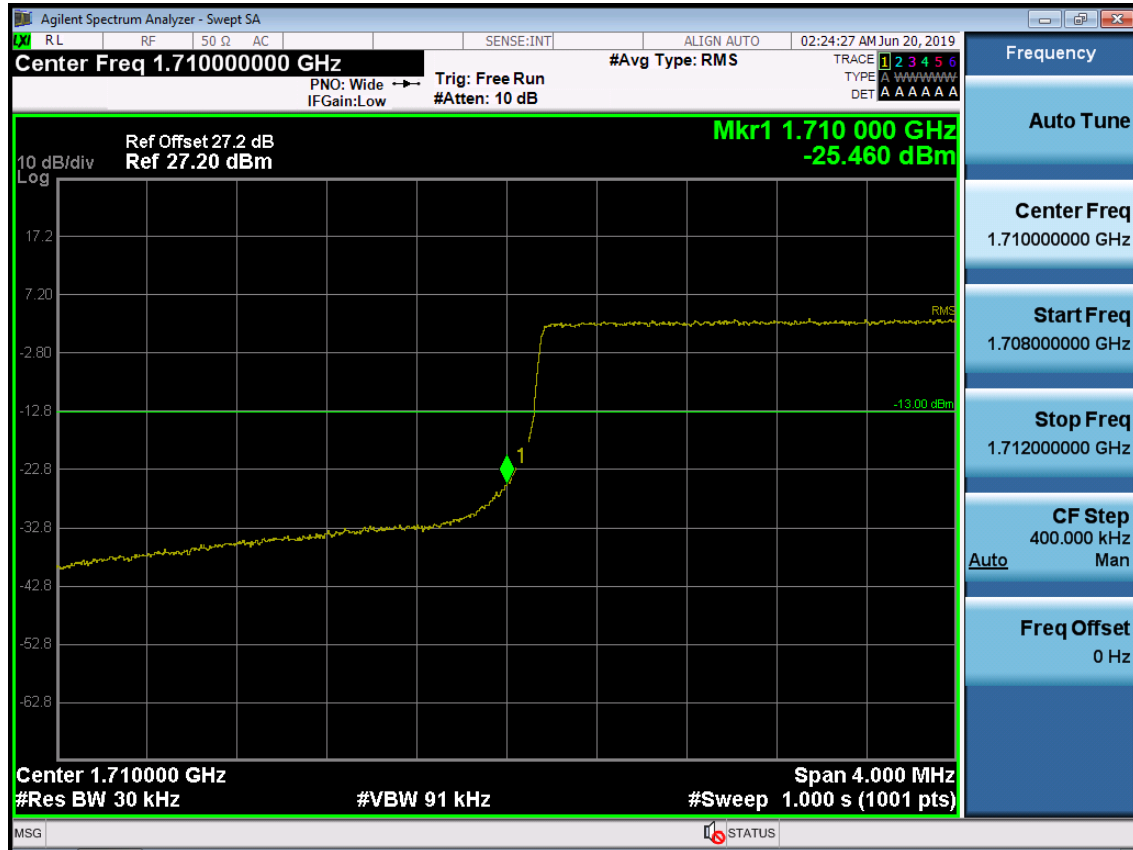
BAND 66. Lower Band Edge Plot (3M BW Ch.131987 QPSK RB 15) -2
