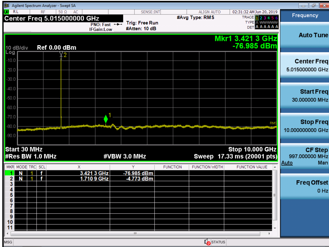
BAND 66. Conducted Spurious Plot_1 (131997ch_5MHz_QPSK_RB 1_0)
