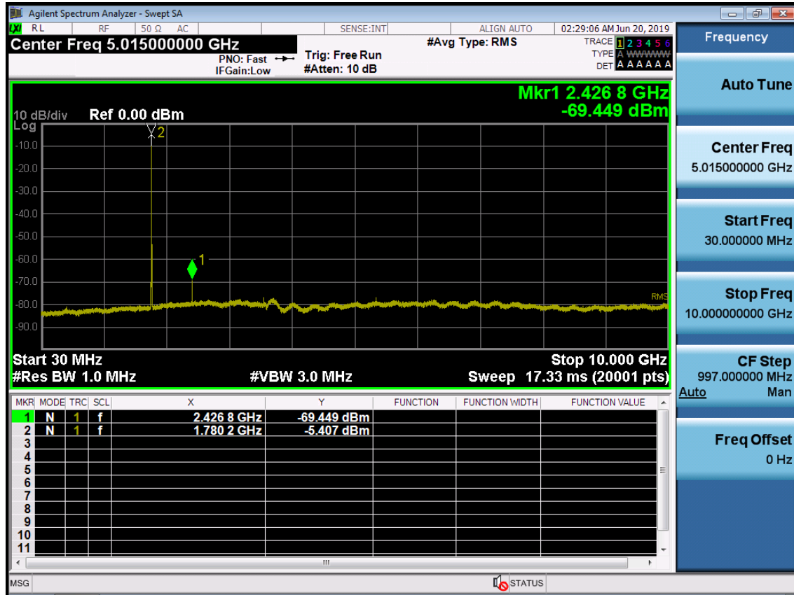
BAND 66. Conducted Spurious Plot_1 (132657ch_3MHz_QPSK_RB 1_0)
