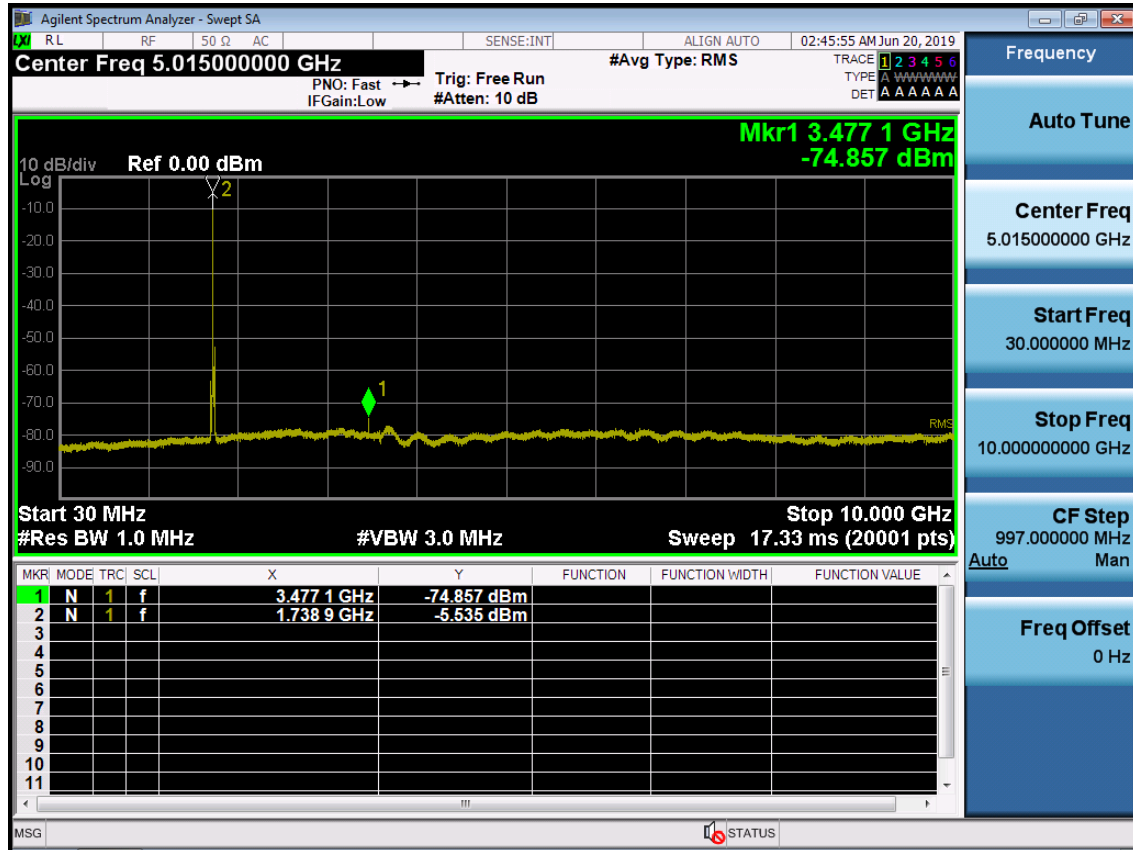
BAND 66. Conducted Spurious Plot_1 (132322ch_15MHz_QPSK_ RB 1_0)
