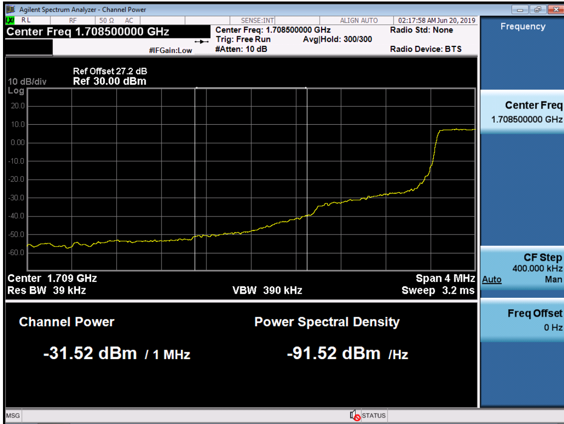
BAND 66. Lower Extended Band Edge Plot (1.4M BW Ch.131979 QPSK_RB6_0) -3
