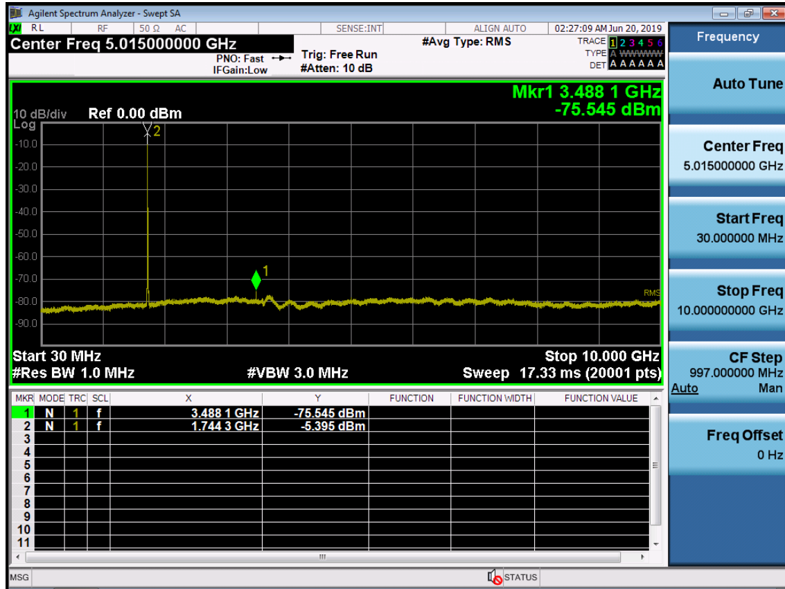
BAND 66. Conducted Spurious Plot_1 (132322ch_3MHz_QPSK_RB 1_0)
