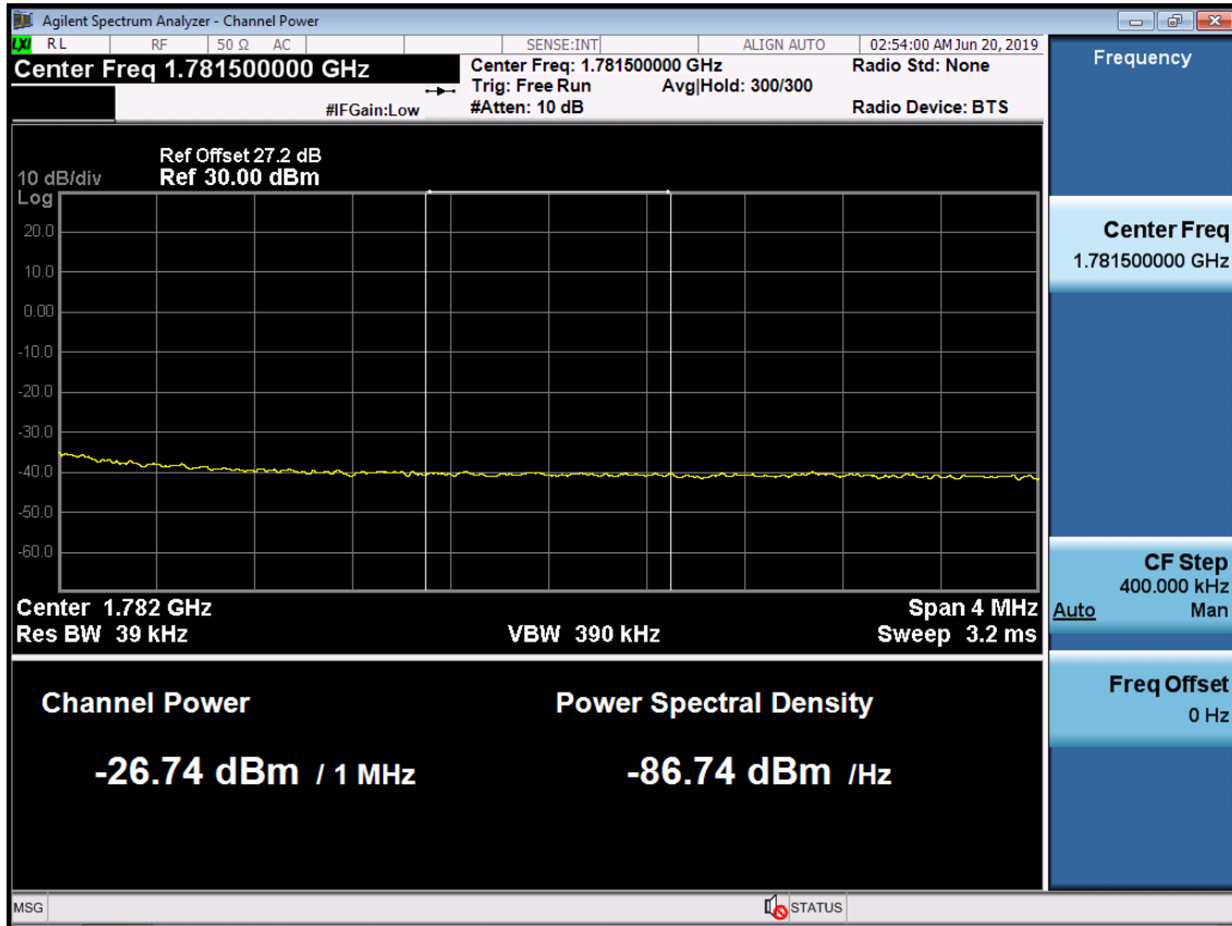
BAND 66. Upper Extended Band Edge Plot (20M BW Ch.132572 QPSK_RB100) -3
