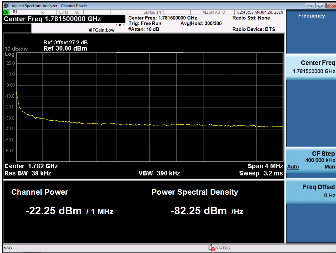
BAND 66. Upper Extended Band Edge Plot (10M BW Ch.132622 QPSK_RB50) -3
