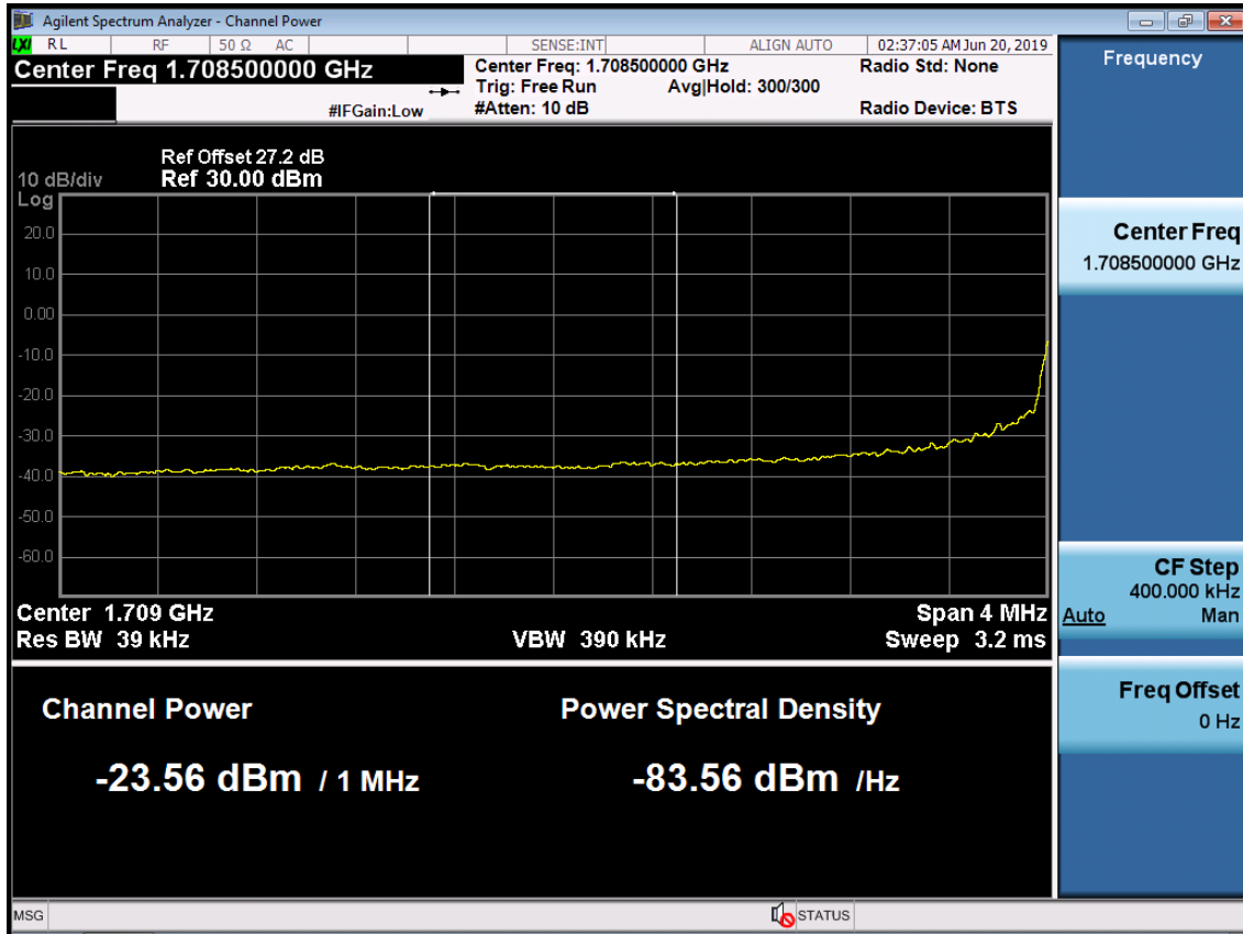
BAND 66. Lower Extended Band Edge Plot (10M BW Ch.132022 QPSK_RB50_0) -3
