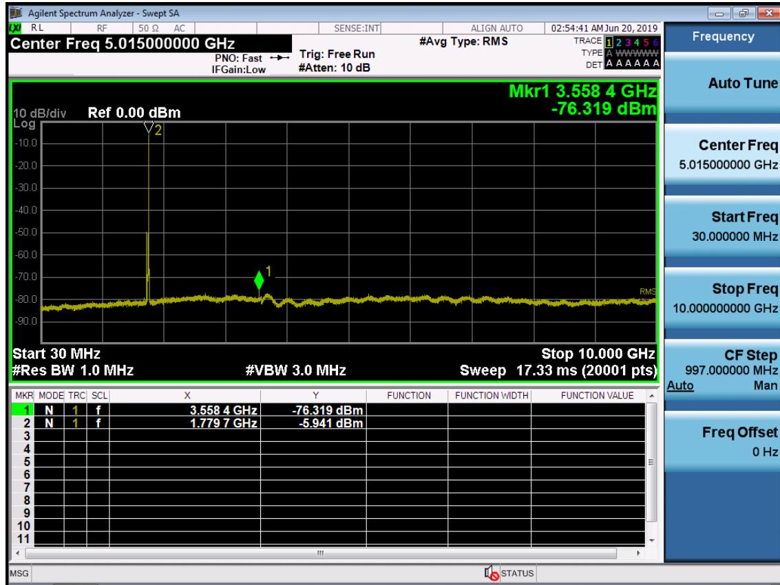
BAND 66. Conducted Spurious Plot_1 (132572ch_20MHz_QPSK_ RB 1_0)
