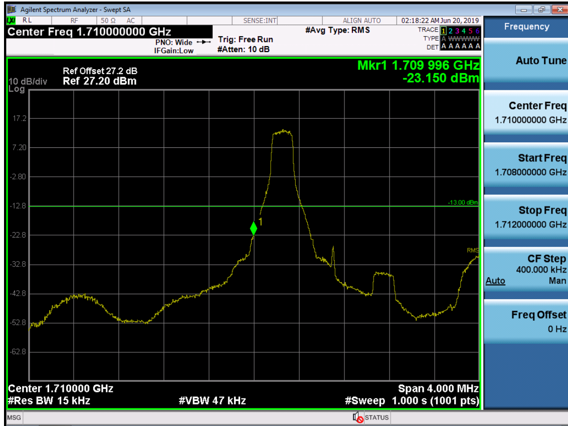
BAND 66. Lower Band Edge Plot (1.4M BW Ch.131979 QPSK RB 1, Offset 0) -1
