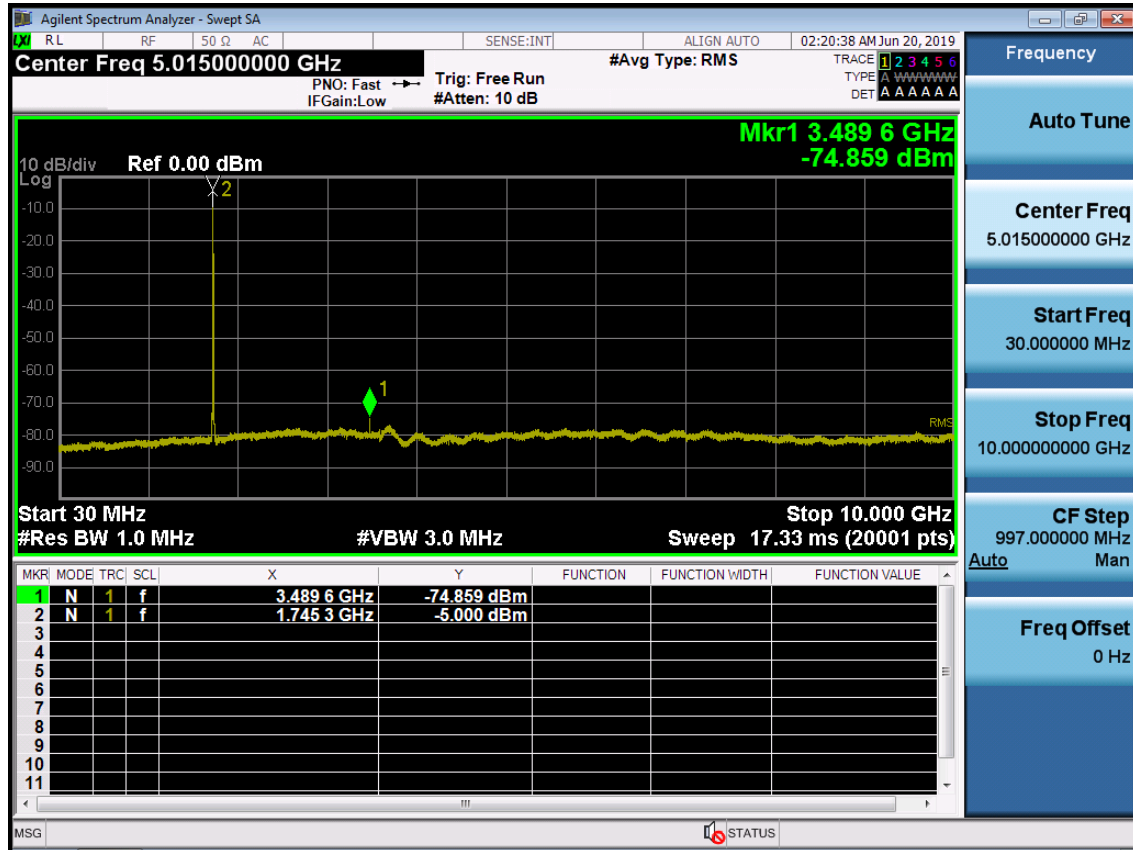
BAND 66. Conducted Spurious Plot_1 (132322ch_1.4MHz_QPSK_ RB 1_0)
