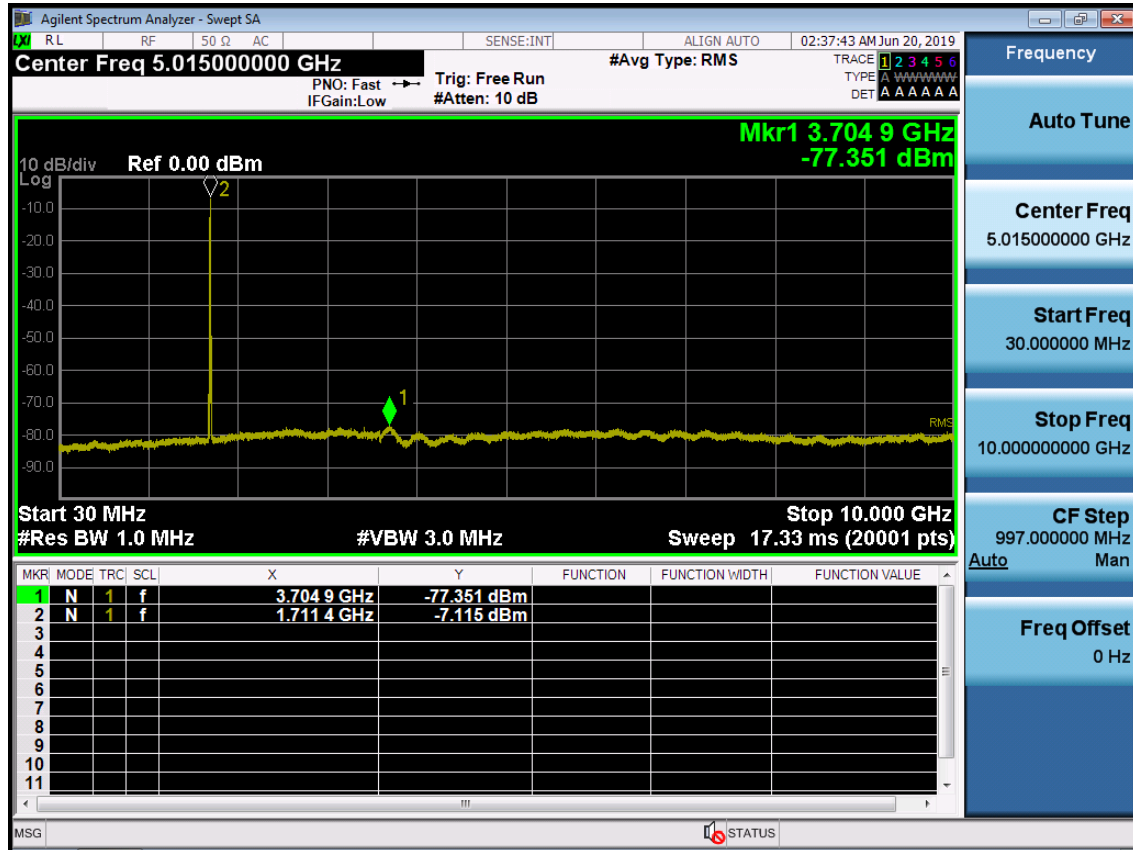
BAND 66. Conducted Spurious Plot_1 (132022ch_10MHz_QPSK_ RB 1_0)
