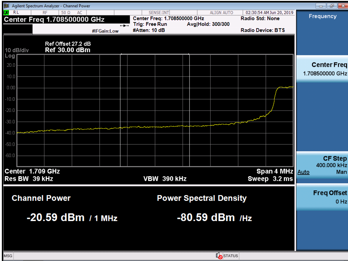
BAND 66. Lower Extended Band Edge Plot (5M BW Ch.131997 QPSK_RB25_0) -3
