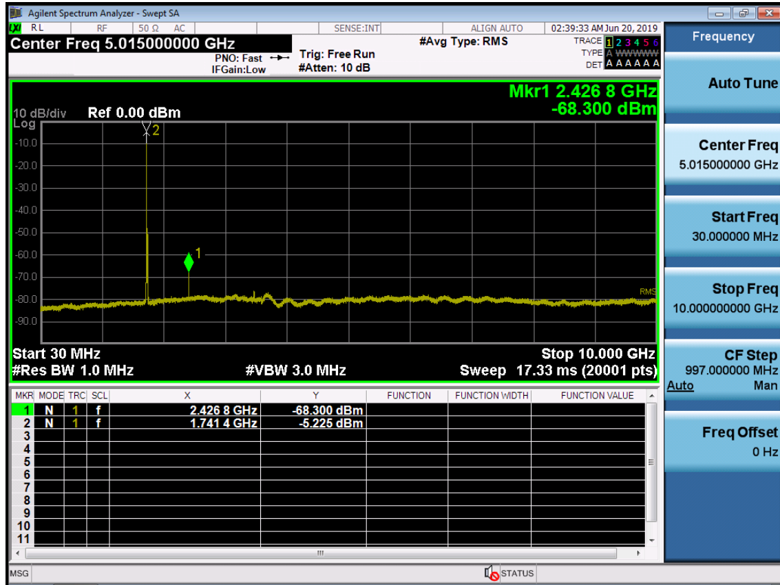
BAND 66. Conducted Spurious Plot_1 (132322ch_10MHz_QPSK_ RB 1_0)
