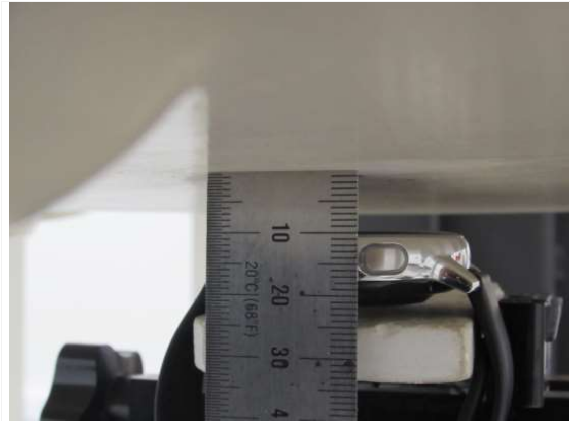
Distance of 10 mm from the EUT
