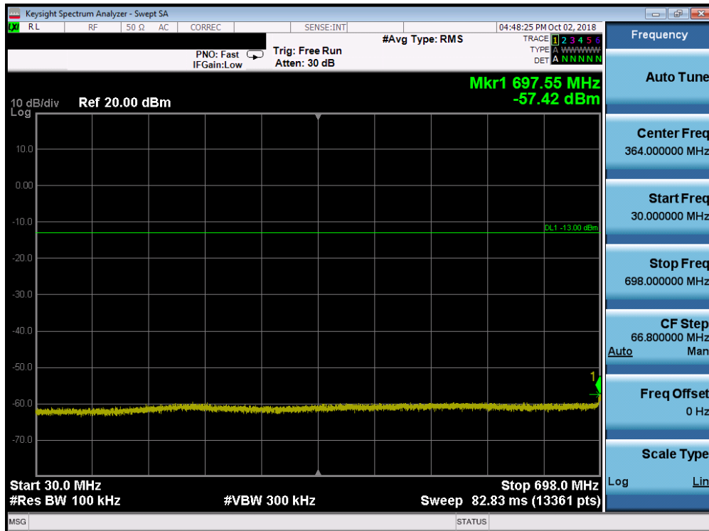
Plot 7-68. Conducted Spurious Plot (Band 12 - 5.0MHz QPSK - RB Size 1, RB Offset 0 - High Channel)
