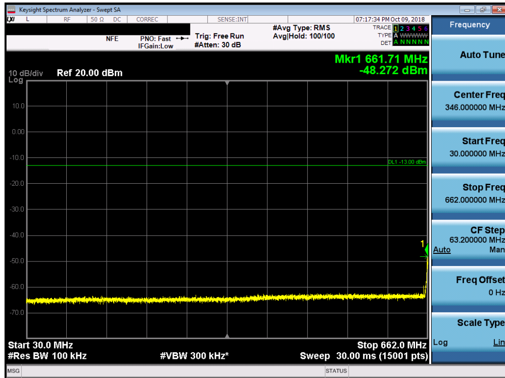
Plot 7-53. Conducted Spurious Plot (Band 71 - 20.0MHz QPSK - RB Size 1, RB Offset 0 - Low Channel)
