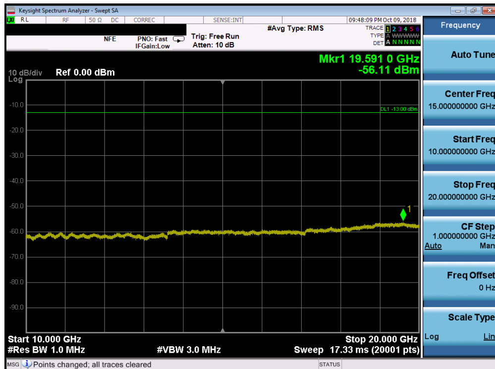
Plot 7-88. Conducted Spurious Plot (Band 66/4 - 20.0MHz QPSK - RB Size 1, RB Offset 0 - Mid Channel)
