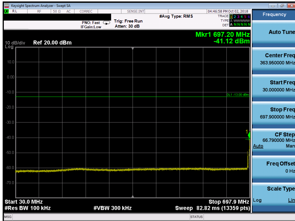
Plot 7-62. Conducted Spurious Plot (Band 12 - 5.0MHz QPSK - RB Size 1, RB Offset 0 - Low Channel)
