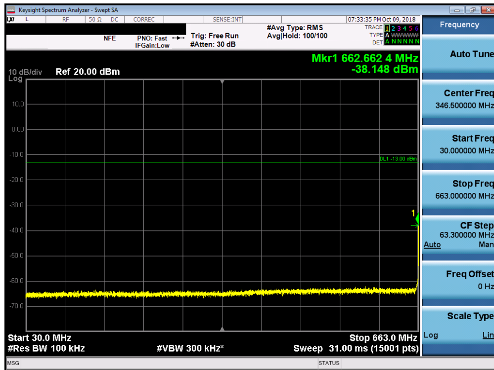
Plot 7-56. Conducted Spurious Plot (Band 71 - 20.0MHz QPSK - RB Size 1, RB Offset 0 - Mid Channel)
