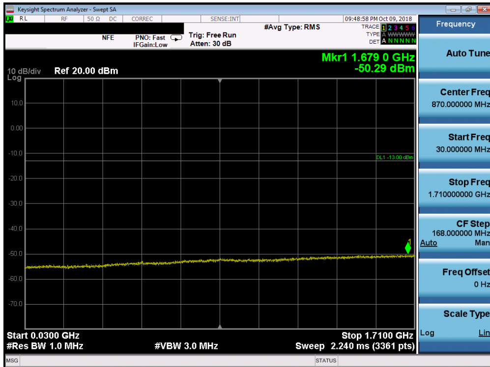
Plot 7-89. Conducted Spurious Plot (Band 66/4 - 20.0MHz QPSK - RB Size 1, RB Offset 0 - High Channel)
