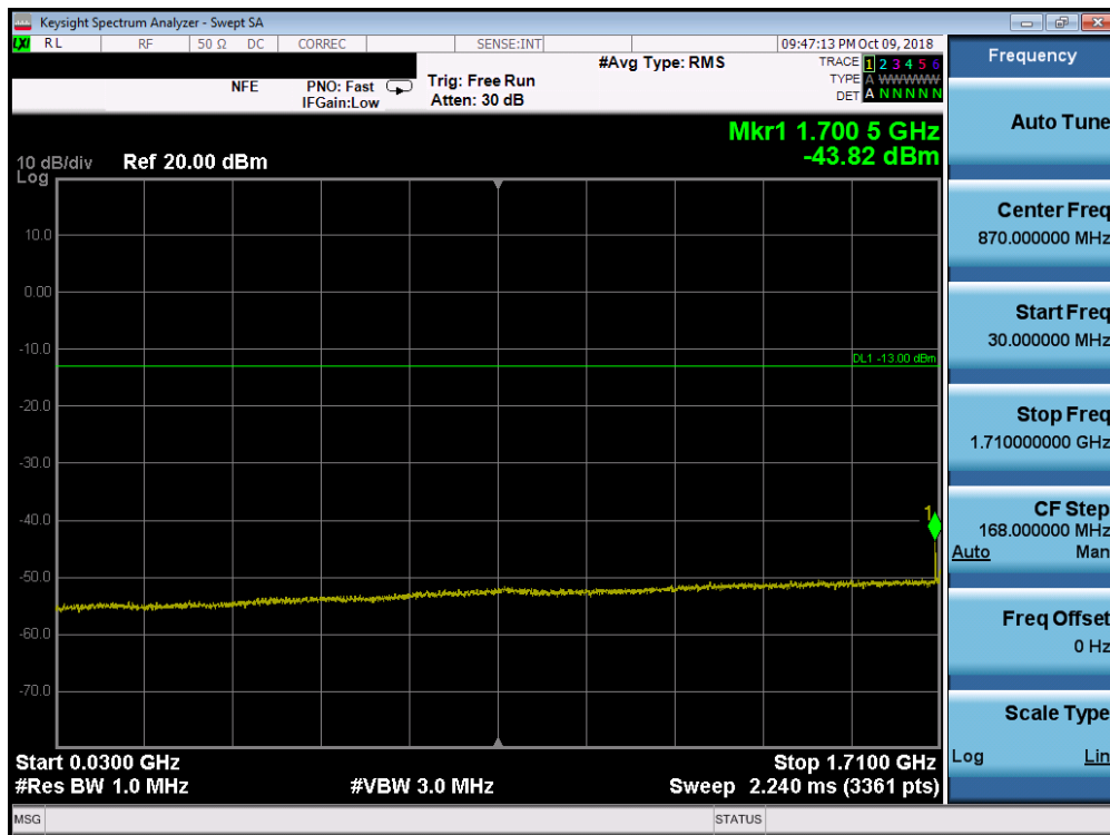
Plot 7-86. Conducted Spurious Plot (Band 66/4 - 20.0MHz QPSK - RB Size 1, RB Offset 0 - Mid Channel)
