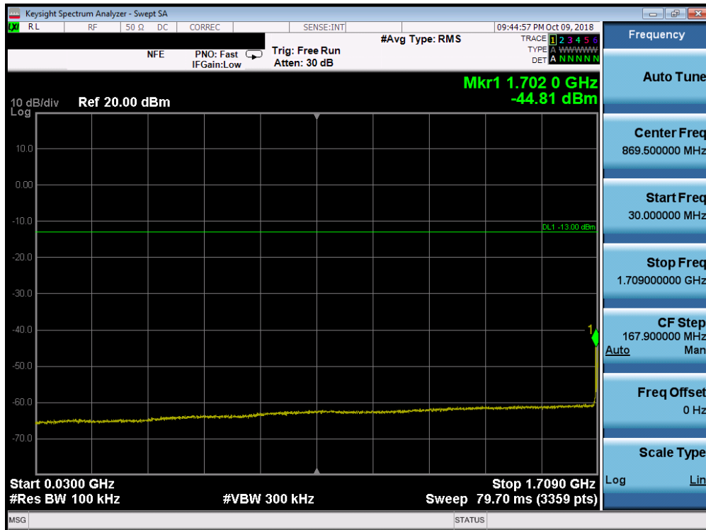
Plot 7-83. Conducted Spurious Plot (Band 66/4 - 20.0MHz QPSK - RB Size 1, RB Offset 0 - Low Channel)
