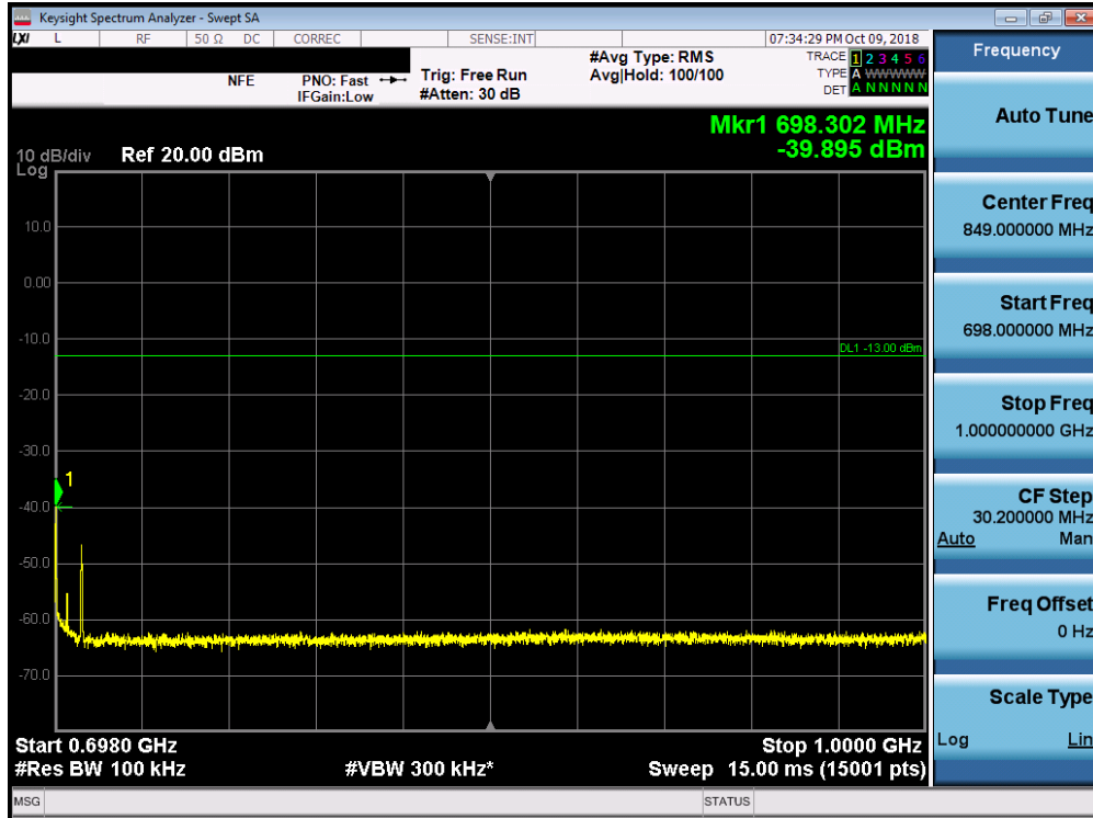
Plot 7-57. Conducted Spurious Plot (Band 71 - 20.0MHz QPSK - RB Size 1, RB Offset 0 - Mid Channel)
