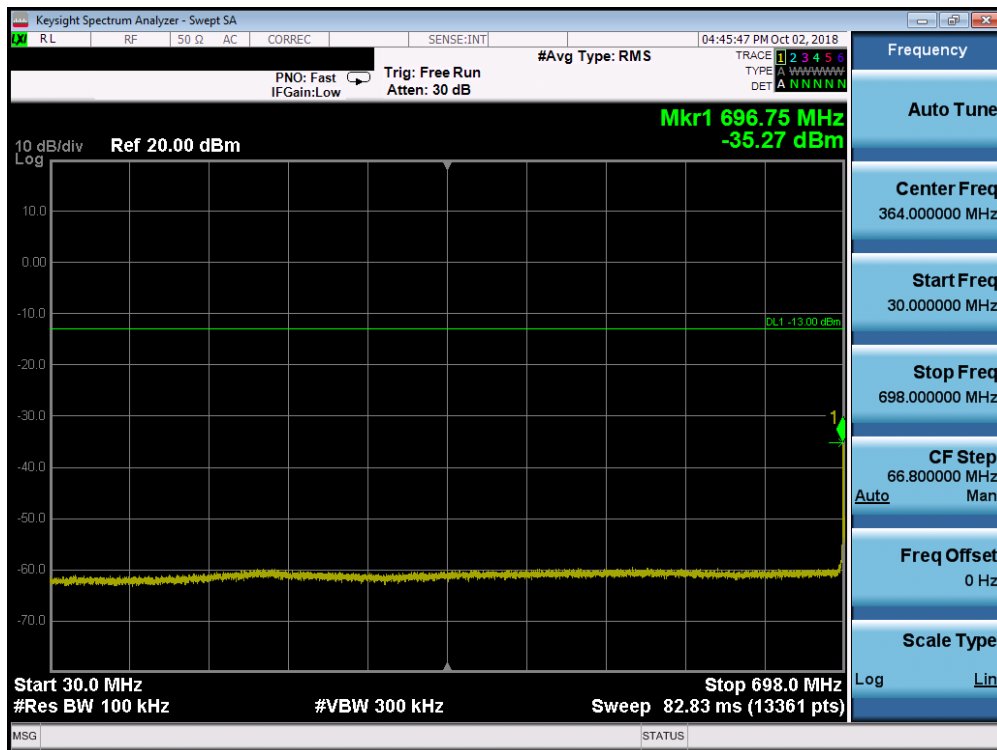
Plot 7-65. Conducted Spurious Plot (Band 12 - 5.0MHz QPSK - RB Size 1, RB Offset 0 - Mid Channel)
