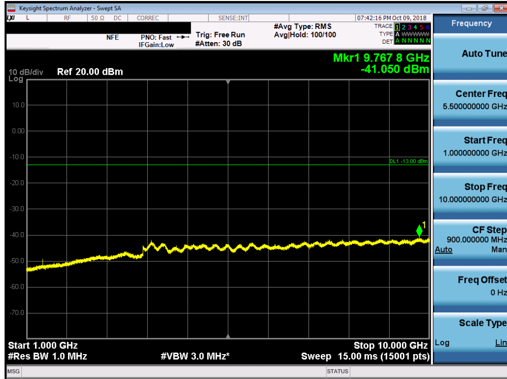
Plot 7-61. Conducted Spurious Plot (Band 71 - 20.0MHz QPSK - RB Size 1, RB Offset 0 - High Channel)
