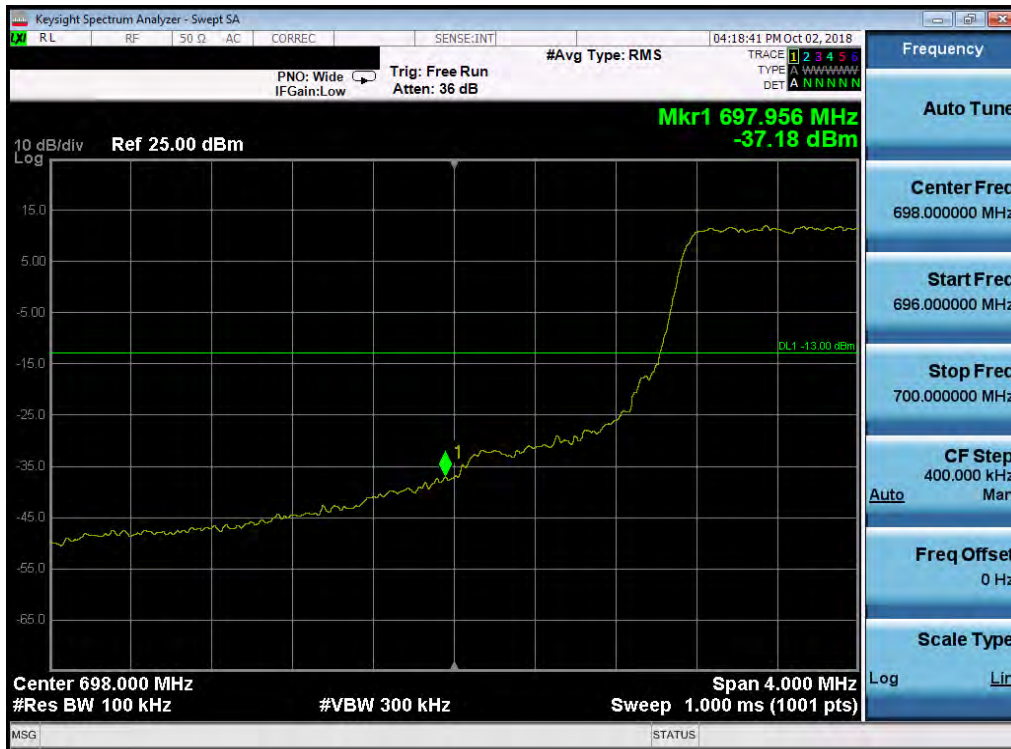
Plot 7-109. Lower Band Edge Plot (Band 12 - 1.4MHz QPSK - Full RB Configuration)
