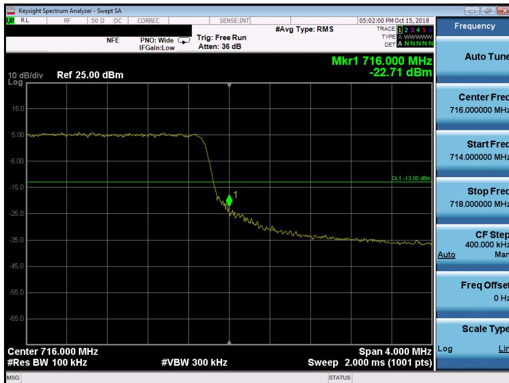
Plot 7-114. Upper Band Edge Plot (Band 12 - 5.0MHz QPSK - Full RB Configuration)
