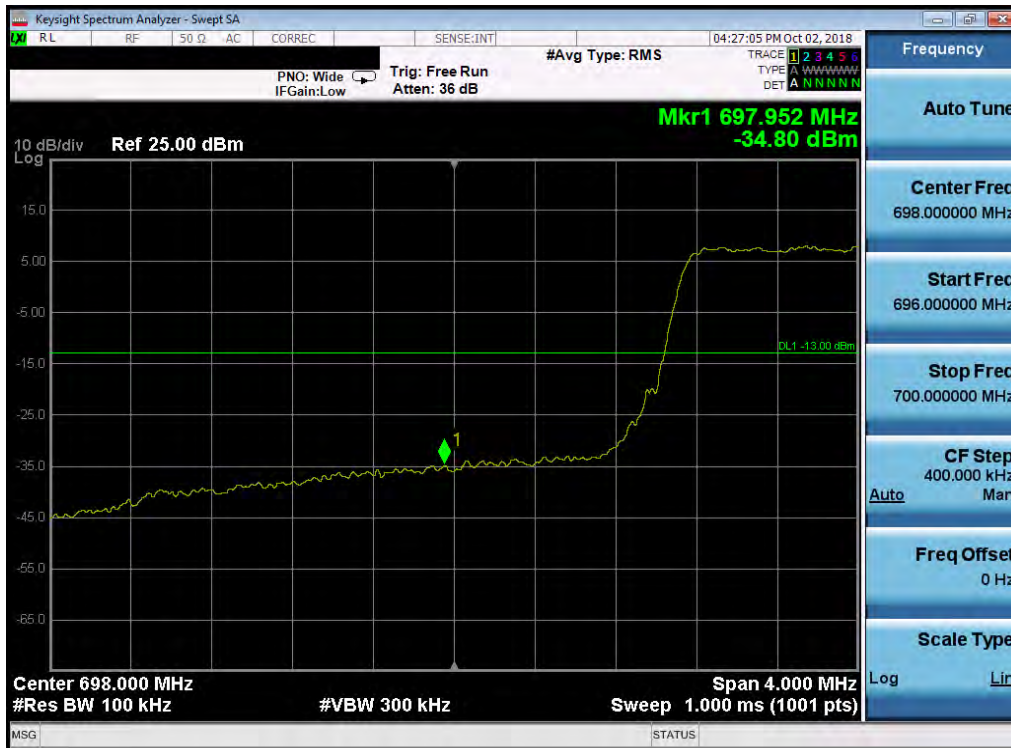
Plot 7-111. Lower Band Edge Plot (Band 12 - 3.0MHz QPSK - Full RB Configuration)
