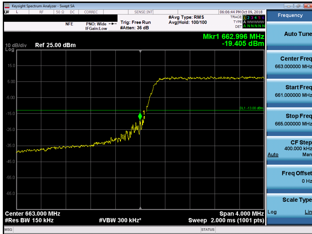
Plot 7-101. Lower Band Edge Plot (Band 71 - 5.0MHz QPSK - Full RB Configuration)
