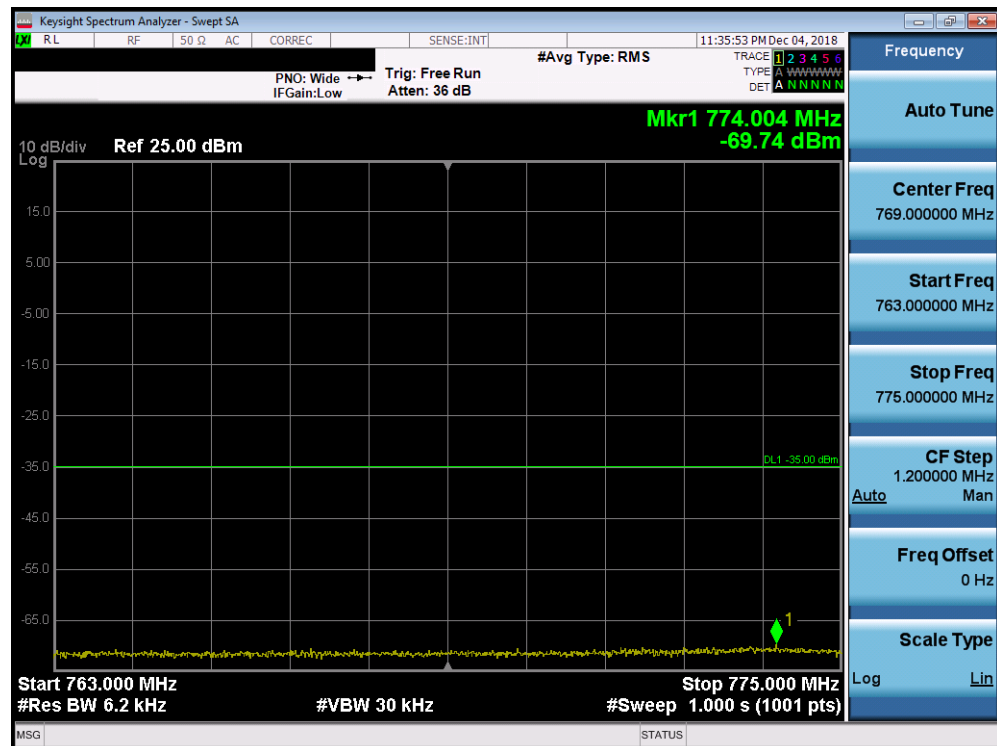
Plot 7-122. Lower Emission Mask Plot (Band 13 - 10.0MHz QPSK - Full RB Configuration)
