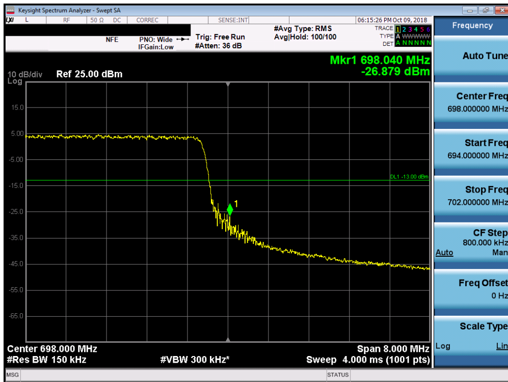
Plot 7-104. Upper Band Edge Plot (Band 71 - 10.0MHz QPSK - Full RB Configuration)
