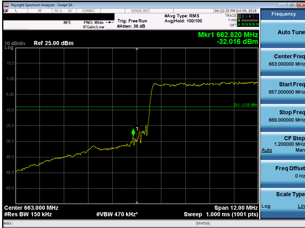
Plot 7-105. Lower Band Edge Plot (Band 71 - 15.0MHz QPSK - Full RB Configuration)
