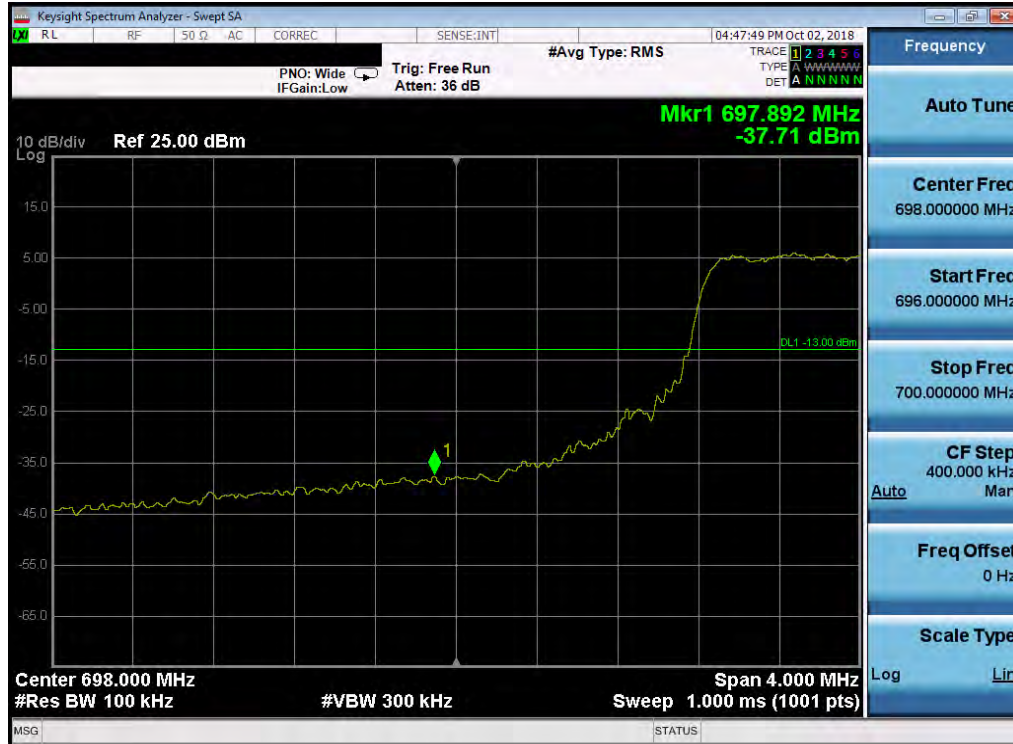
Plot 7-113. Lower Band Edge Plot (Band 12 - 5.0MHz QPSK - Full RB Configuration)
