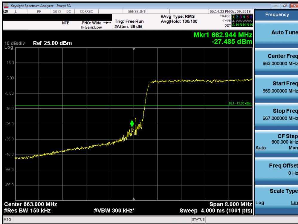
Plot 7-103. Lower Band Edge Plot (Band 71 - 10.0MHz QPSK - Full RB Configuration)
