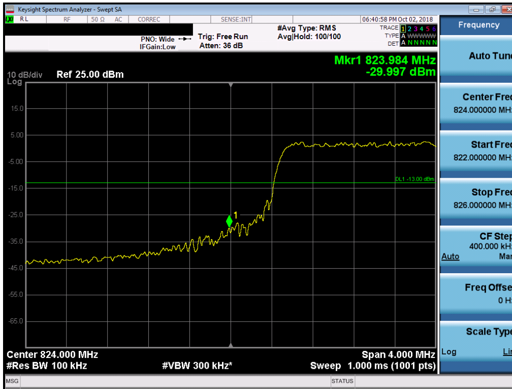
Plot 7-131. Lower Band Edge Plot (Band 5 - 10.0MHz QPSK - Full RB Configuration)
