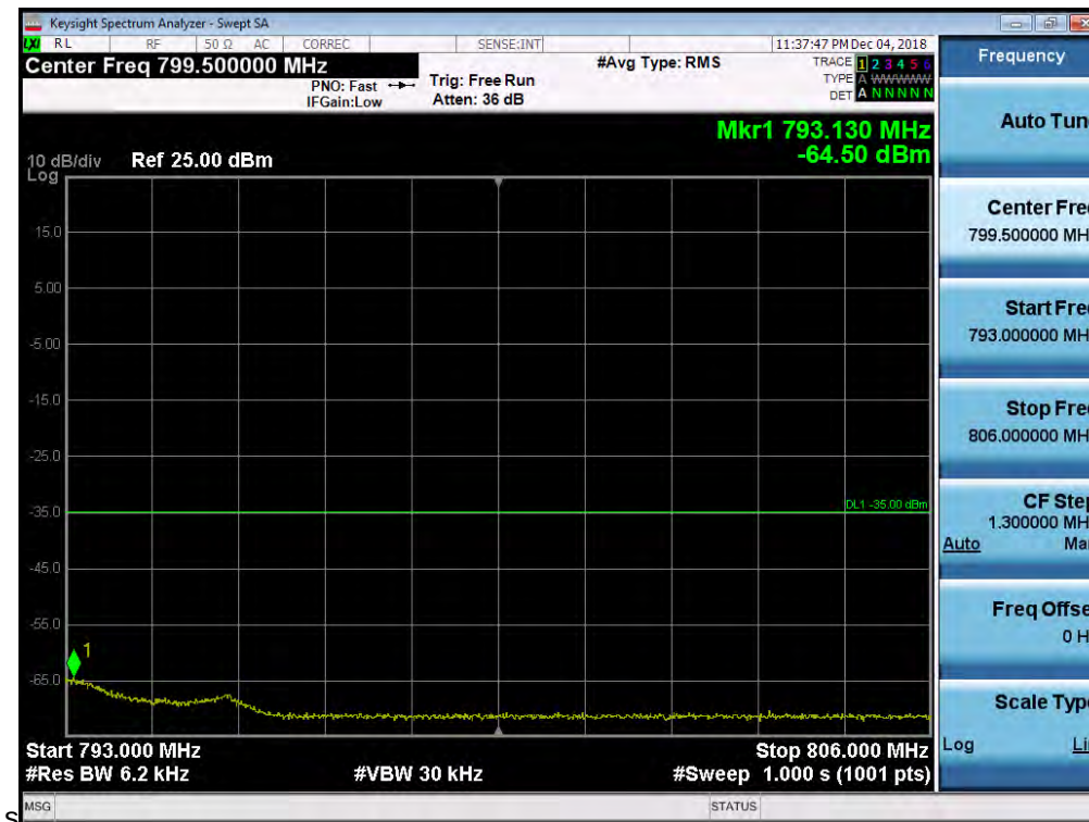
Plot 7-124. Lower Emission Mask Plot (Band 13 - 10.0MHz QPSK - Full RB Configuration)
