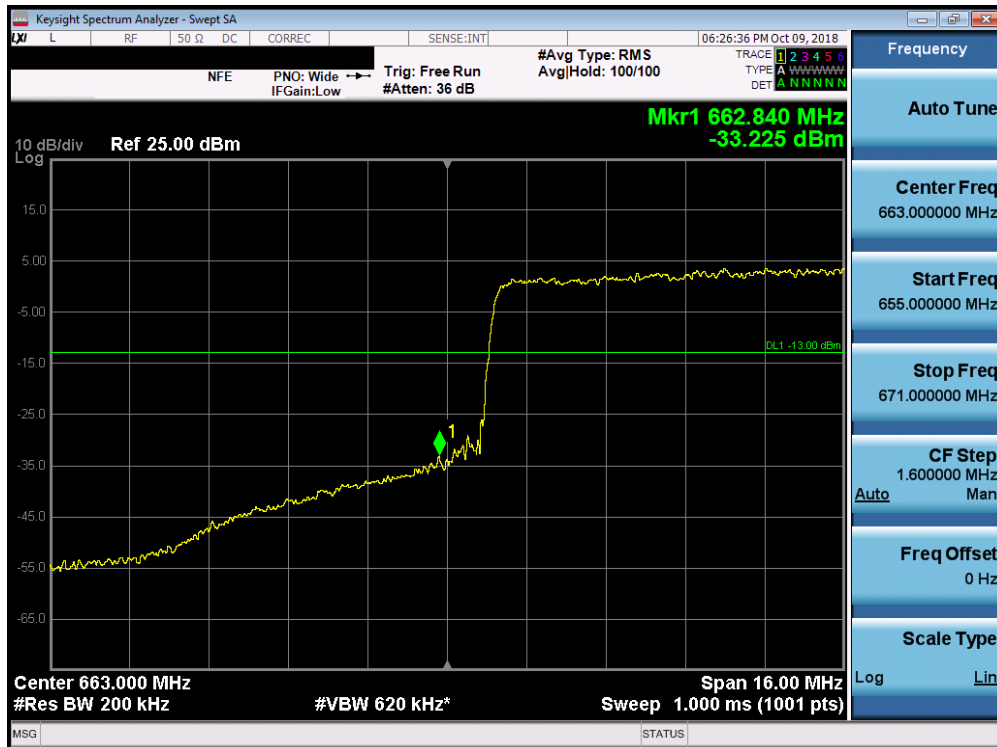
Plot 7-107. Lower Band Edge Plot (Band 71 - 20.0MHz QPSK - Full RB Configuration)
