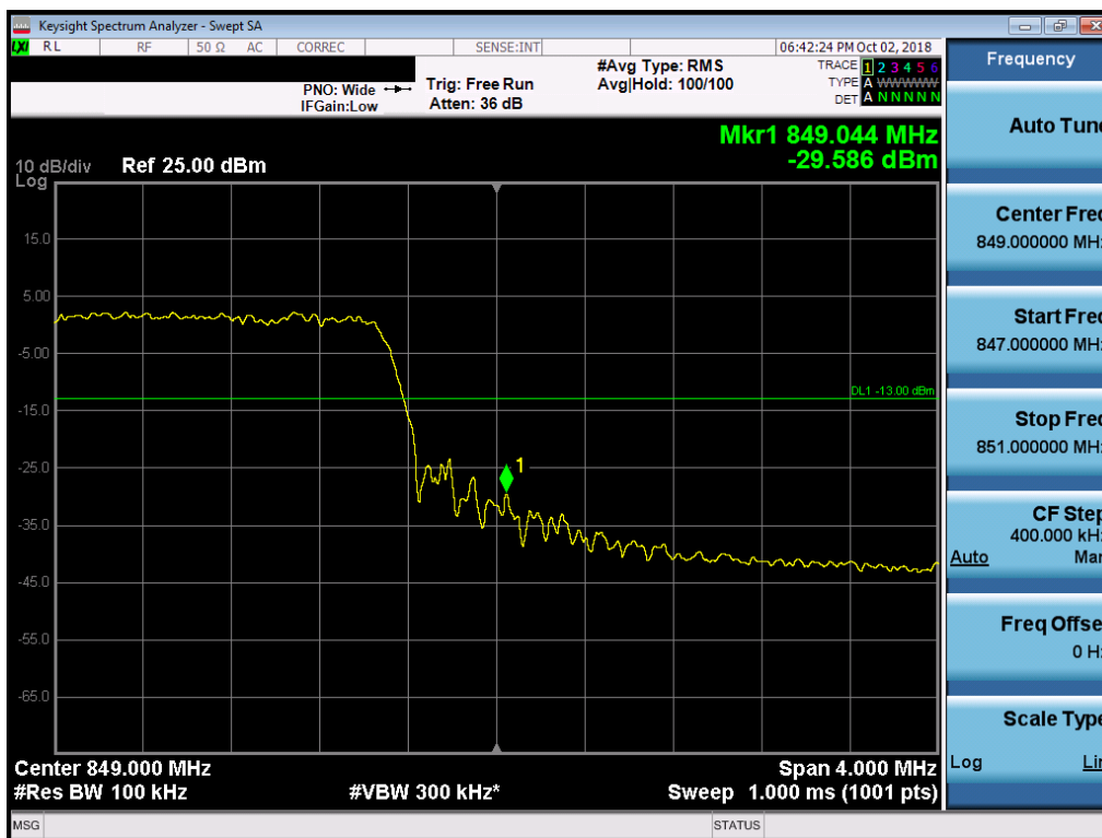
Plot 7-132. Upper Band Edge Plot (Band 5 - 10.0MHz QPSK - Full RB Configuration)
