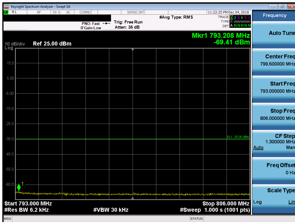
Plot 7-120. Upper Emission Mask Plot (Band 13 - 5.0MHz QPSK - Full RB Configuration)
