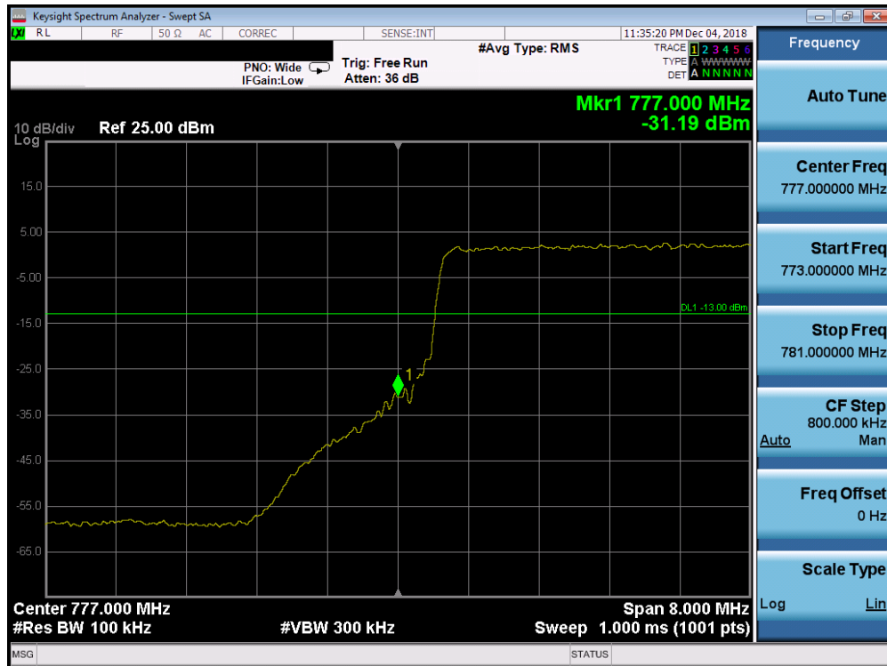
Plot 7-121. Lower Band Edge Plot (Band 13 - 10.0MHz QPSK - Full RB Configuration)
