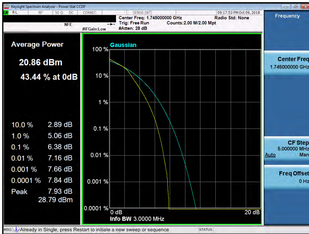
Plot 7-196. PAR Plot (Band 66/4 - 3.0MHz 16-QAM - Full RB Configuration)
