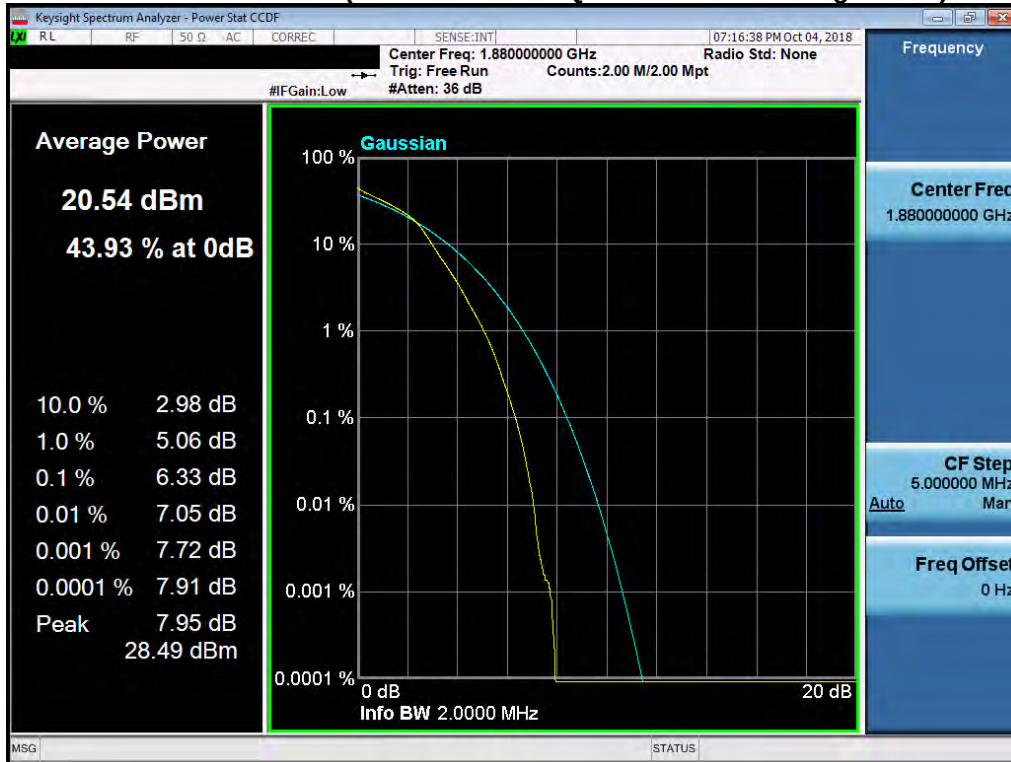
Plot 7-206. PAR Plot (Band 2 - 1.4MHz 16-QAM - Full RB Configuration)
