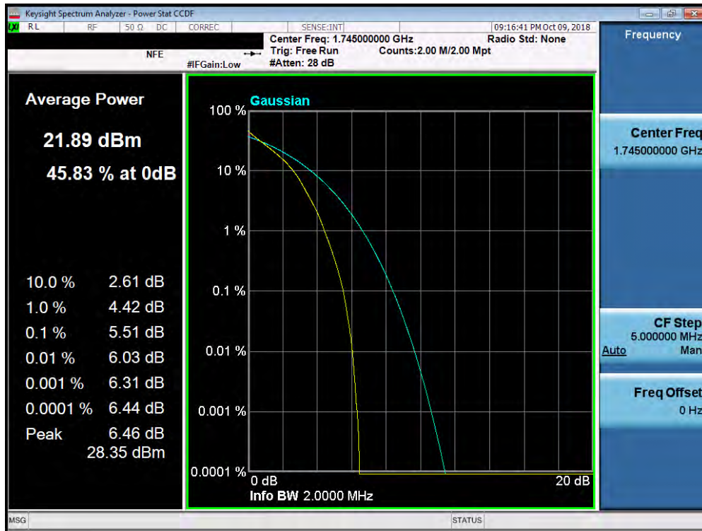
Plot 7-193. PAR Plot (Band 66/4 - 1.4MHz QPSK - Full RB Configuration)
