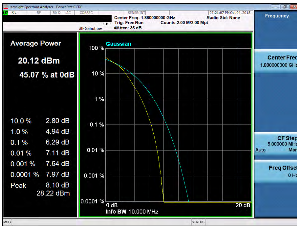
Plot 7-212. PAR Plot (Band 2 - 10.0MHz 16-QAM - Full RB Configuration)
