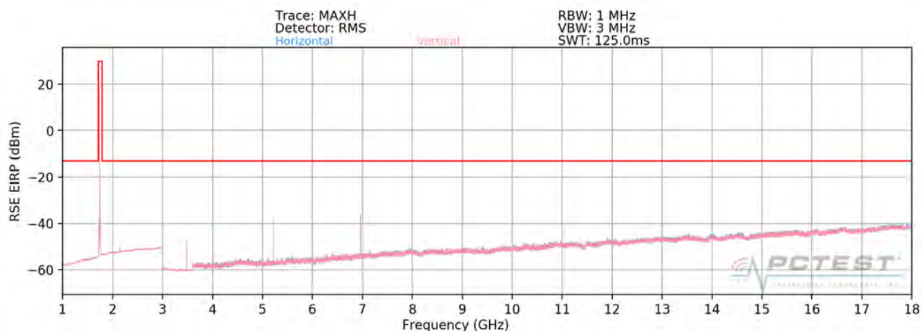
Plot 7-221. Radiated Spurious Plot above 1GHz (Band 66/4)
