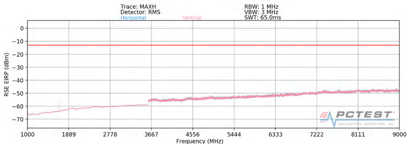
Plot 7-220. Radiated Spurious Plot above 1GHz (Band 5)
