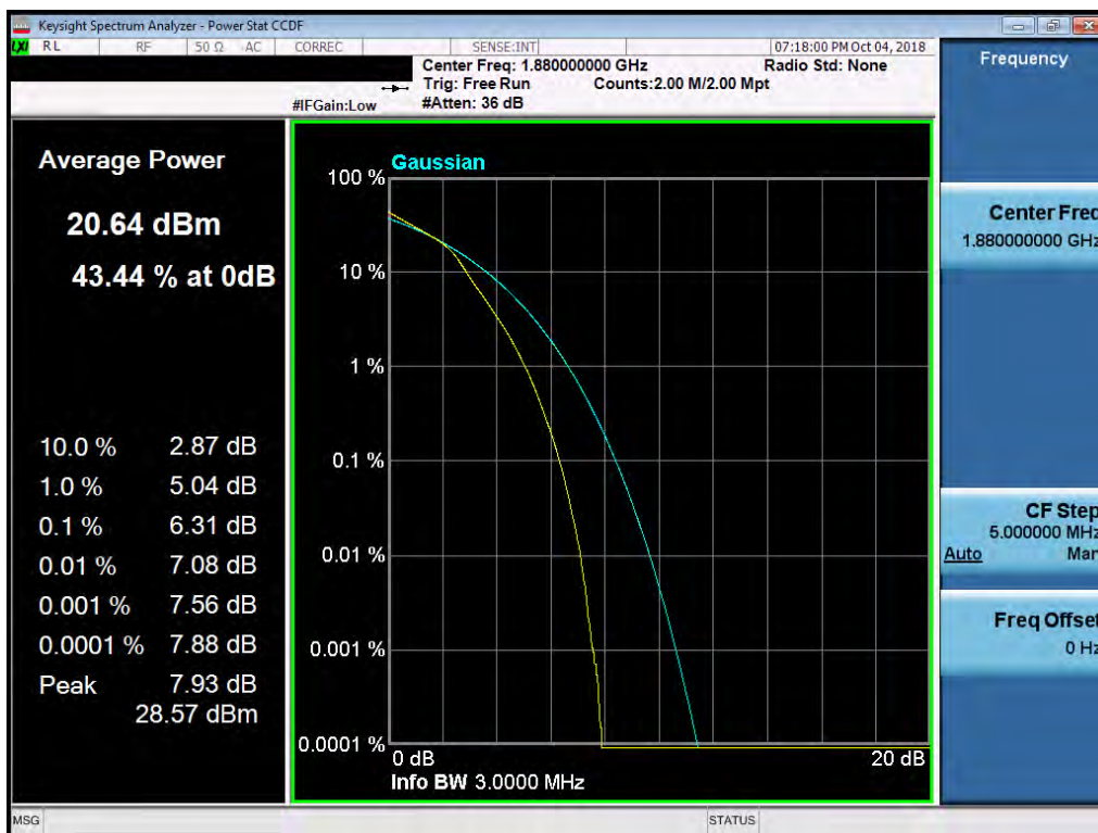
Plot 7-208. PAR Plot (Band 2 - 3.0MHz 16-QAM - Full RB Configuration)
