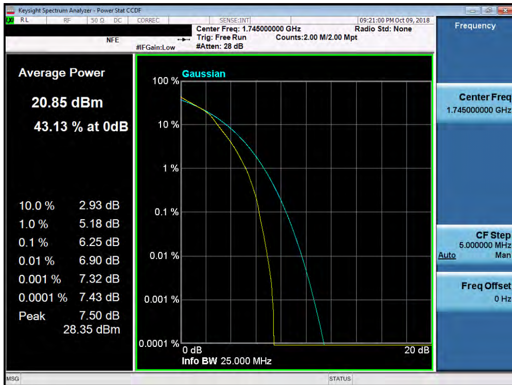
Plot 7-202. PAR Plot (Band 66/4 - 15.0MHz 16-QAM - Full RB Configuration)
