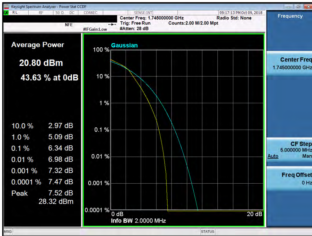
Plot 7-194. PAR Plot (Band 66/4 - 1.4MHz 16-QAM - Full RB Configuration)
