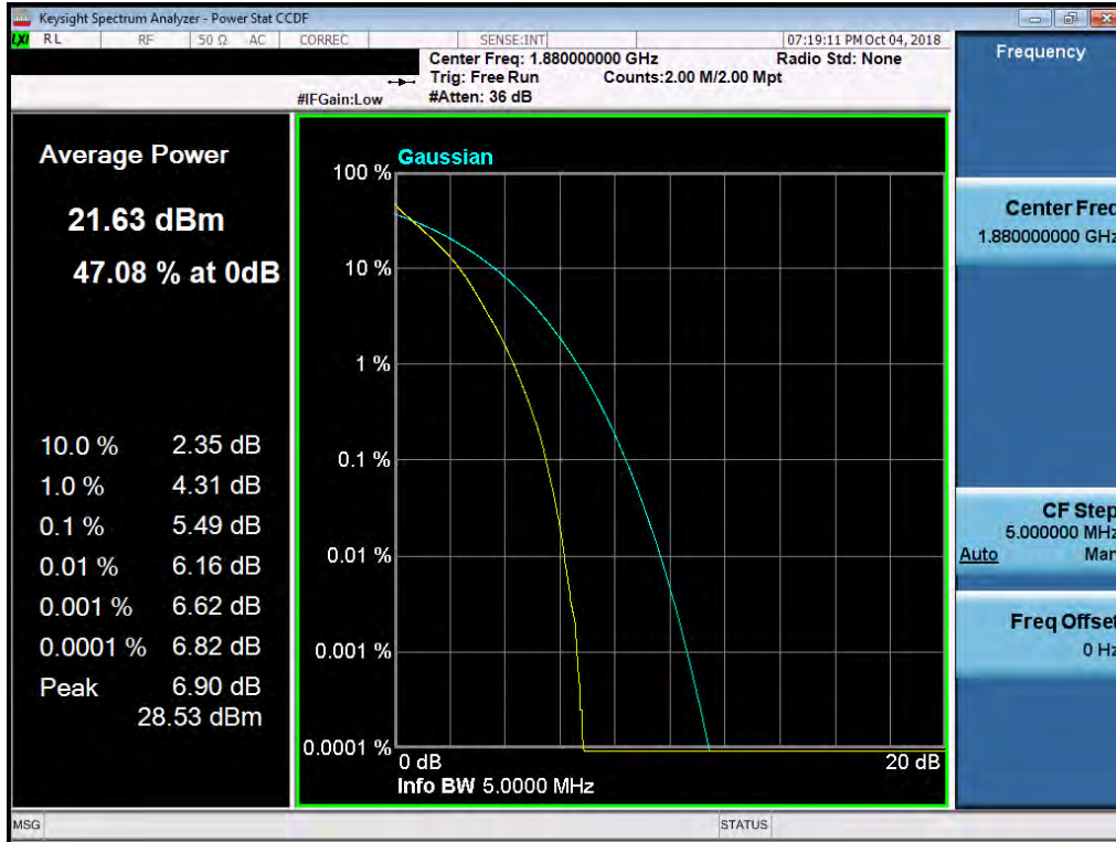
Plot 7-209. PAR Plot (Band 2 - 5.0MHz QPSK - Full RB Configuration)
