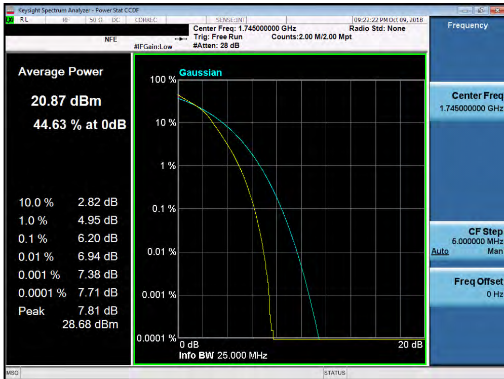
Plot 7-204. PAR Plot (Band 66/4 - 20.0MHz 16-QAM - Full RB Configuration)
