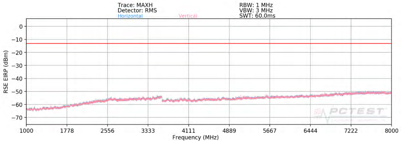
Plot 7-219. Radiated Spurious Plot above 1GHz (Band 13)
