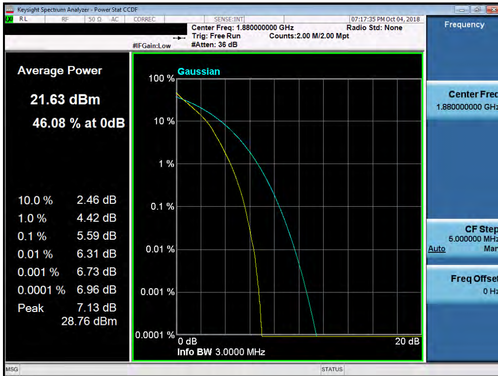
Plot 7-207. PAR Plot (Band 2 - 3.0MHz QPSK - Full RB Configuration)
