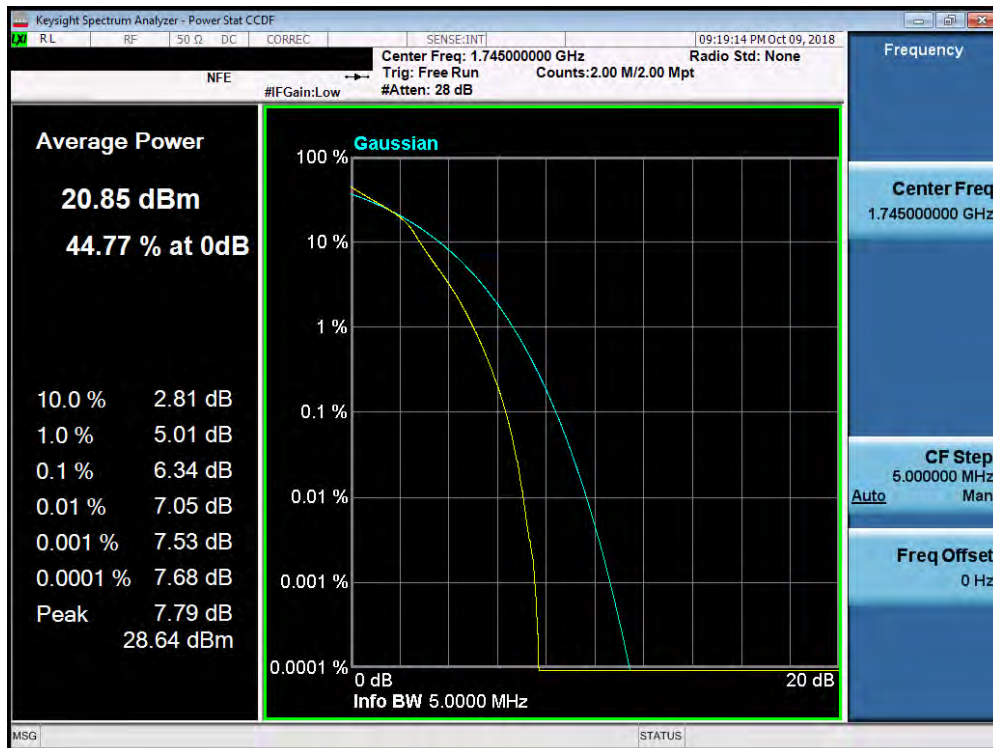
Plot 7-198. PAR Plot (Band 66/4 - 5.0MHz 16-QAM - Full RB Configuration)
