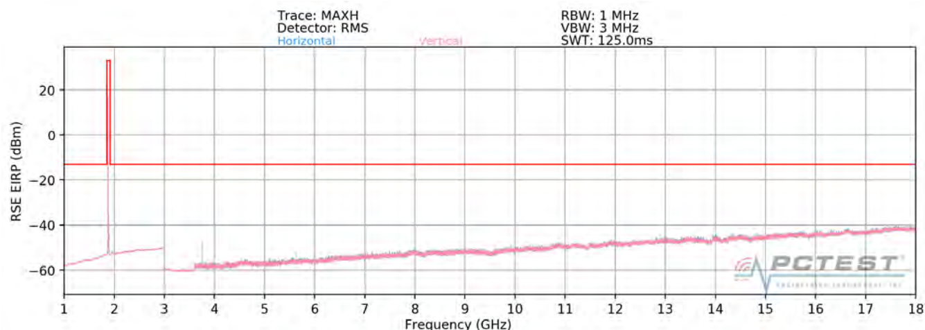
Plot 7-222. Radiated Spurious Plot above 1GHz (Band 2)
