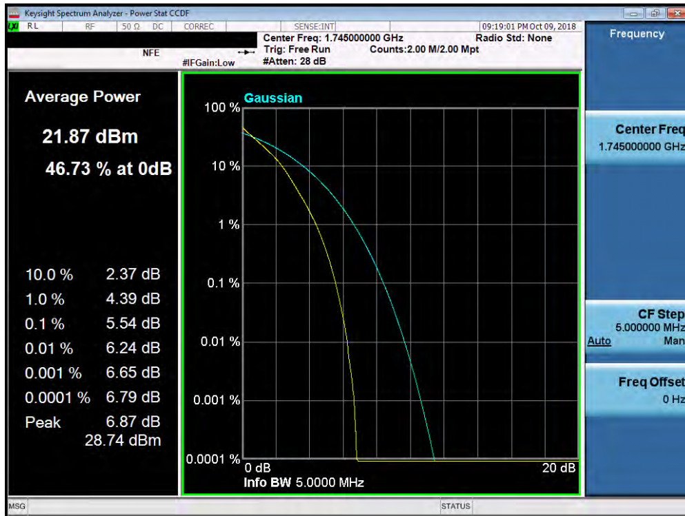
Plot 7-197. PAR Plot (Band 66/4 - 5.0MHz QPSK - Full RB Configuration)
