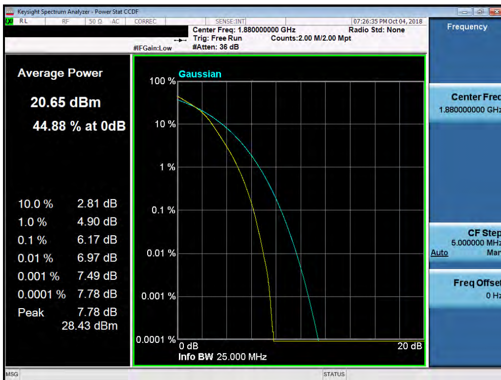
Plot 7-216. PAR Plot (Band 2 - 20.0MHz 16-QAM - Full RB Configuration)
