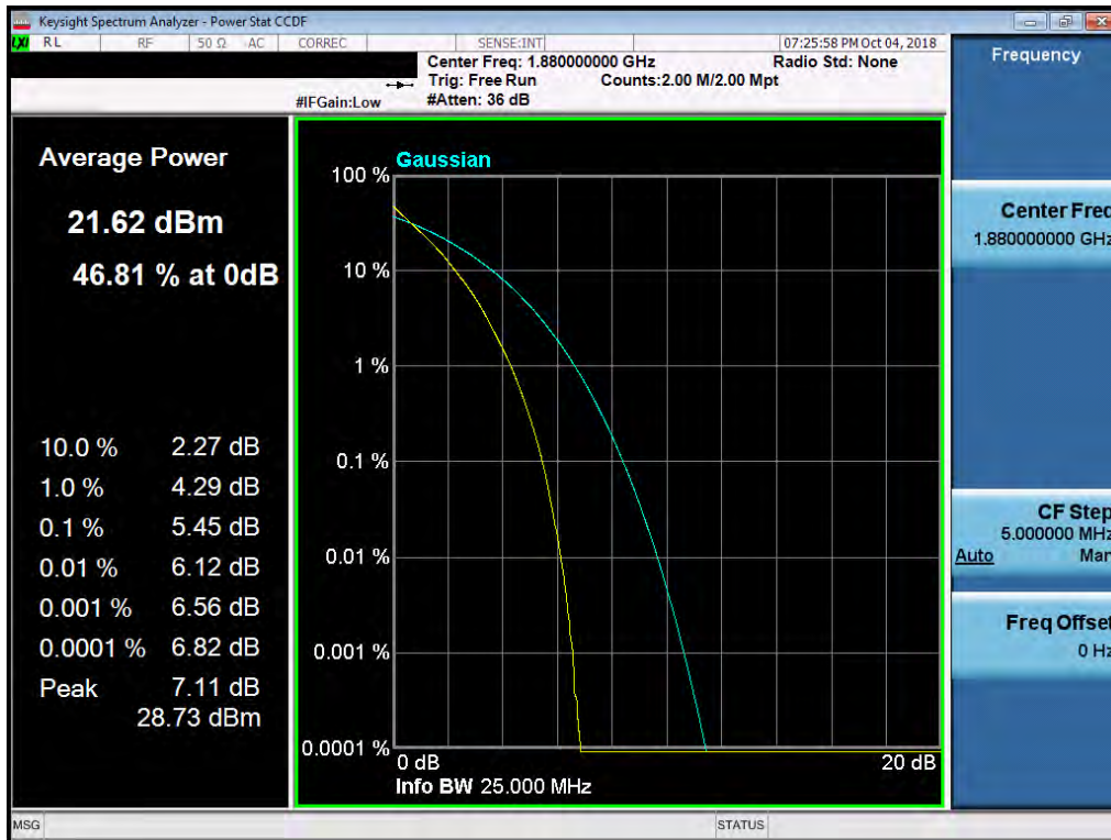
Plot 7-215. PAR Plot (Band 2 - 20.0MHz QPSK - Full RB Configuration)
