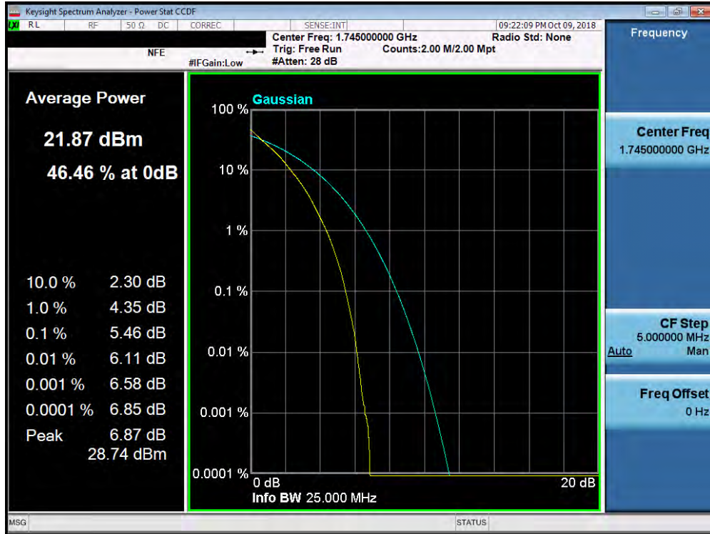
Plot 7-203. PAR Plot (Band 66/4 - 20.0MHz QPSK - Full RB Configuration)
