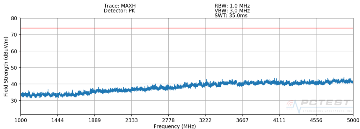
Plot 7-2. Radiated Spurious Plot above 1GHz (Ant. H)
