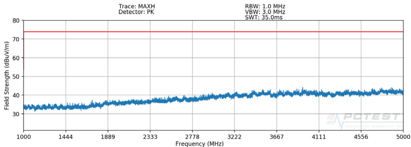
Plot 7-3. Radiated Spurious Plot above 1GHz (Ant. V)
