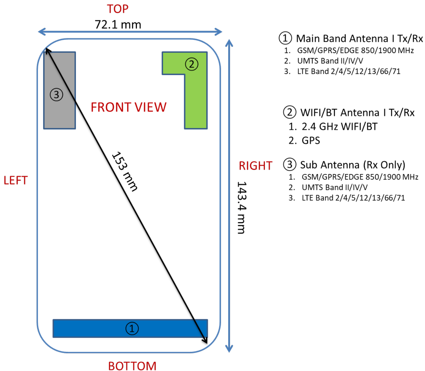
Figure F-1 DUT Antenna Locations
