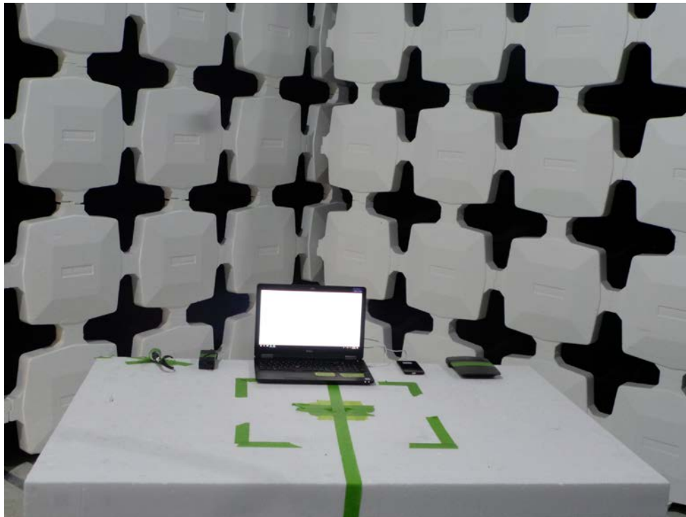
Radiated Measurement (Configuration 1- Front)
