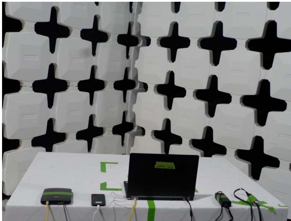
Radiated Measurement (Configuration 1- Back)
