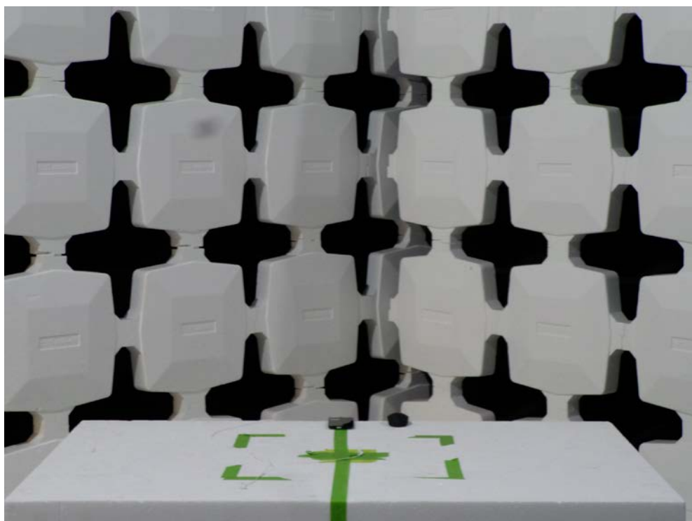
Radiated Measurement (Configuration 3)
