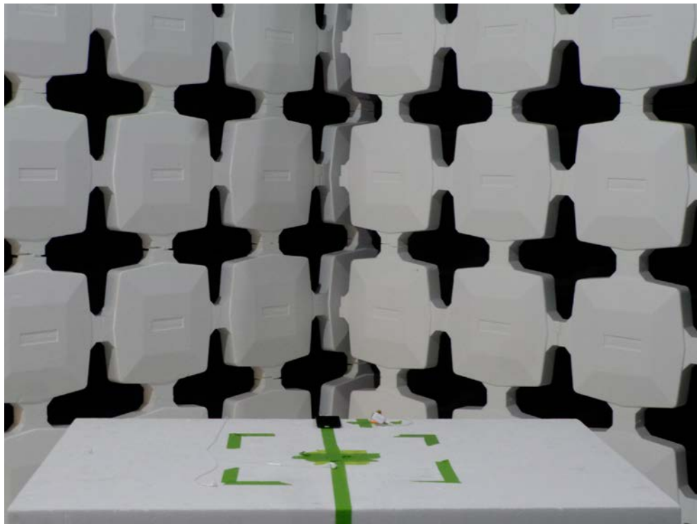
Radiated Measurement (Configuration 2)
