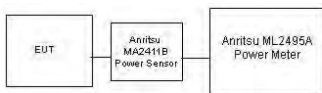
Figure 9-2 Power Measurement Setup
