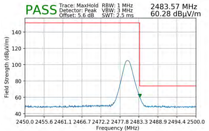
Plot 7-94. Radiated Restricted Upper Band Edge Measurement with WCP (Peak) – ANT1
