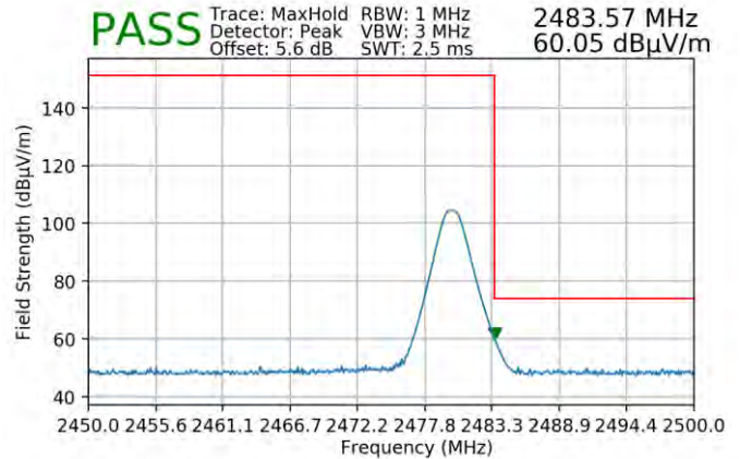
Plot 7-92. Radiated Restricted Upper Band Edge Measurement (Peak) – ANT1
