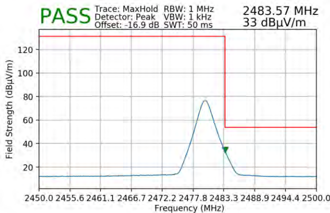
Plot 7-97. Radiated Restricted Upper Band Edge Measurement with WCP (Average) – ANT2
