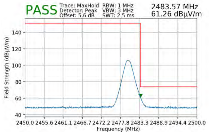
Plot 7-98. Radiated Restricted Upper Band Edge Measurement with WCP (Peak) – ANT2
