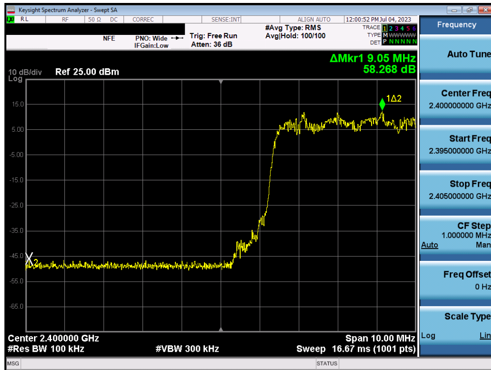
Plot 7-57. Band Edge Plot (Bluetooth with Hopping Enabled, 3 Mbps – Ch. 0) – ANT1
