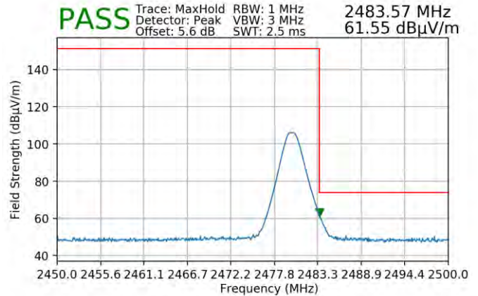
Plot 7-96. Radiated Restricted Upper Band Edge Measurement (Peak) – ANT2
