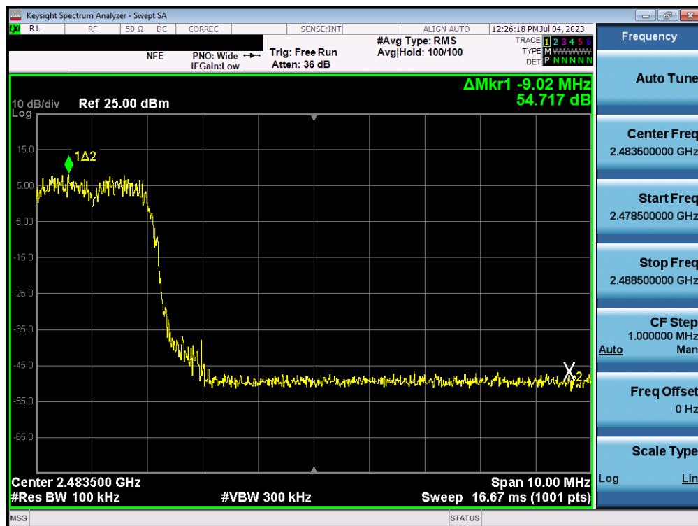
Plot 7-62. Band Edge Plot (Bluetooth with Hopping Enabled, 3 Mbps – Ch. 78) – ANT2
