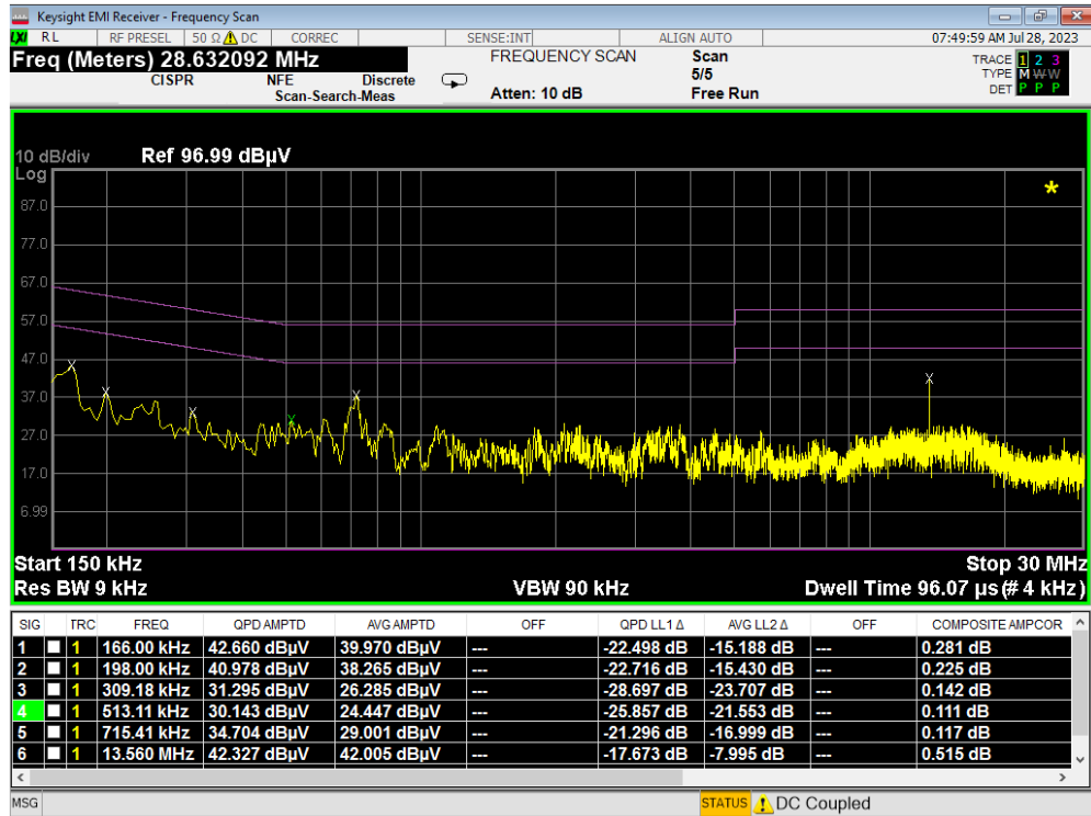
Plot 7-5. Line-Conducted Test Plot (L1) - Device to Device – 150kHz to 30MHz
