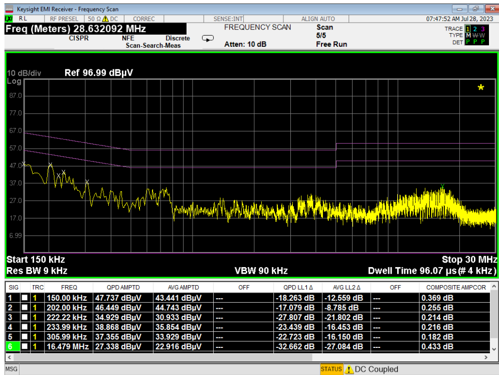
Plot 7-6. Line-Conducted Test Plot (N) - Device to Device – 150kHz to 30MHz
