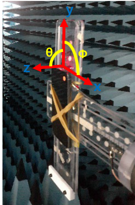
Figure 1: Geometry for SM-S711B for Radiation patterns.
