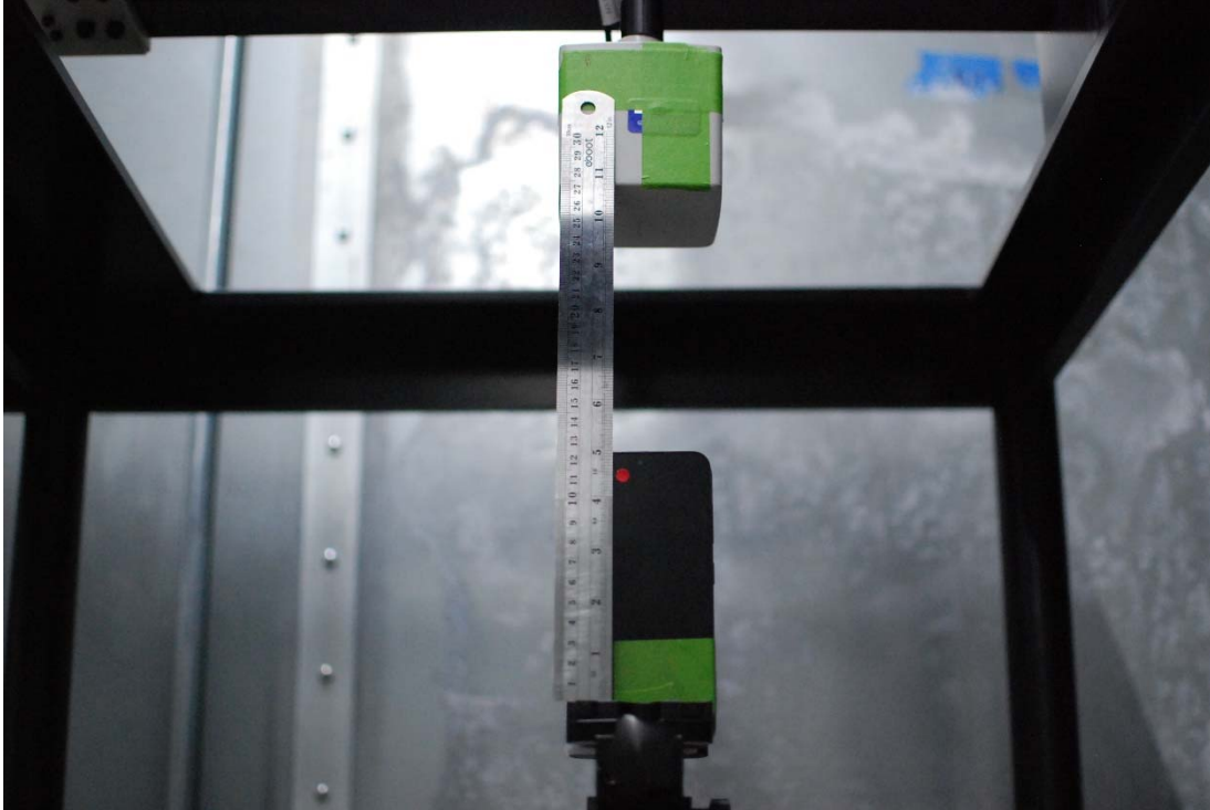
Test Setup Photo 9 H-field, Top edge, 15cm
