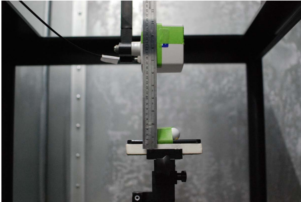
Test Setup Photo 15 E-field, Back side, 15cm
