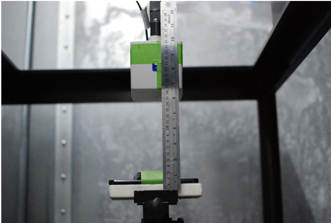
Test Setup Photo 14 H-field, Back side, 15cm
