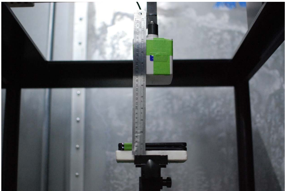
Test Setup Photo 8 H-field, Front side, 15cm
