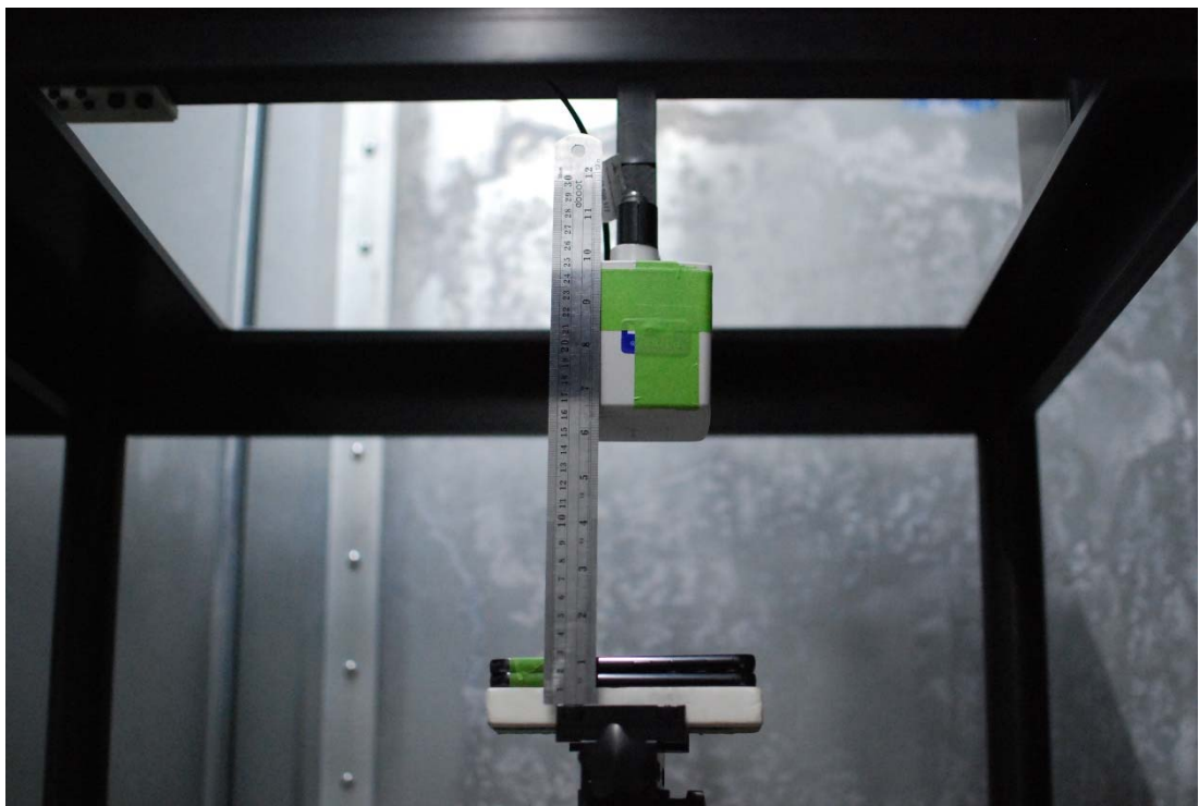
Test Setup Photo 7 H-field, Back side, 15cm
