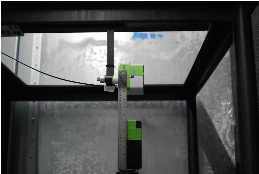
Test Setup Photo 4 E-field, Bottom edge, 15cm
