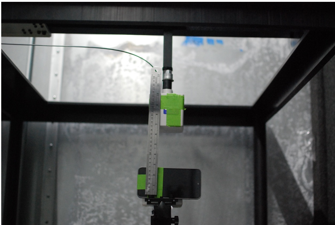
Test Setup Photo 12 H-field, Left edge, 15cm
