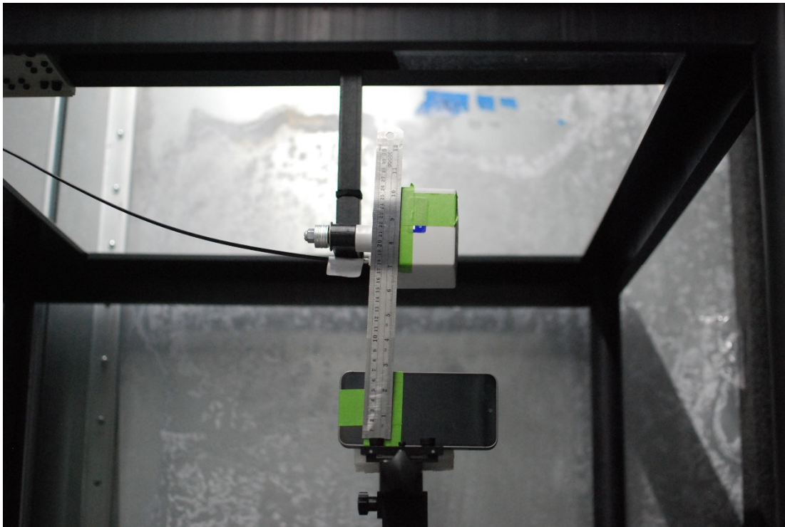
Test Setup Photo 6 E-field, Left edge, 15cm
