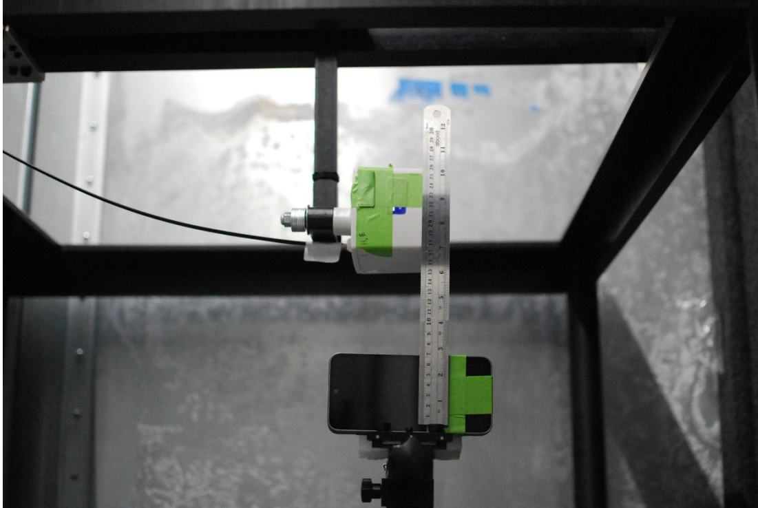
Test Setup Photo 5 E-field, Right edge, 15cm
