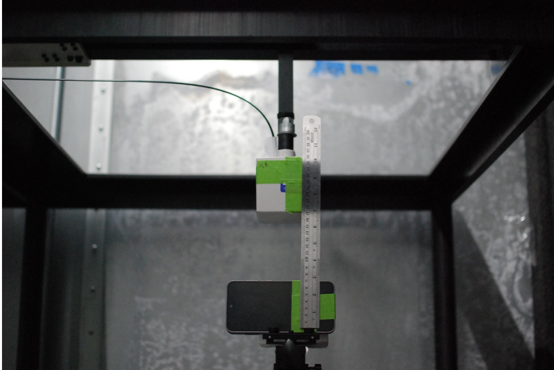
Test Setup Photo 11 H-field, Right edge, 15cm
