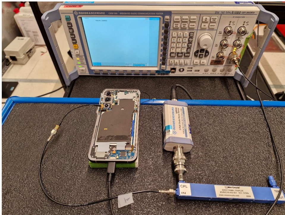
Test Setup Photo 10 – Conducted Test Setup (Figure 7-2)
