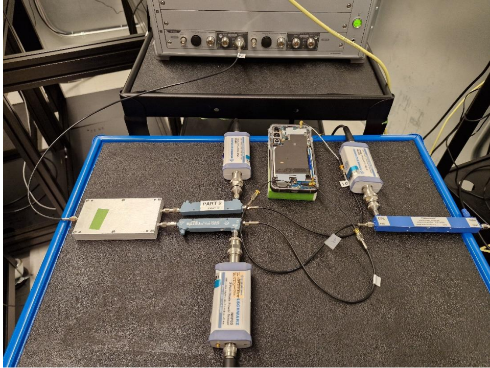
Test Setup Photo 9 – Conducted Test Setup (Figure 7-1d)
