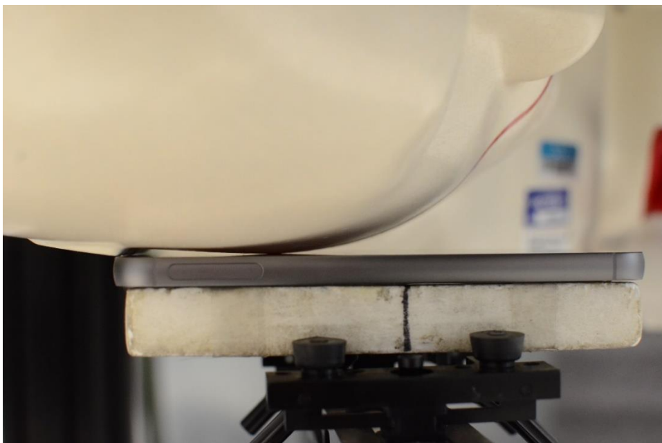
Test Setup Photo 14 – Head, Right, Cheek (Figure 7-6)
