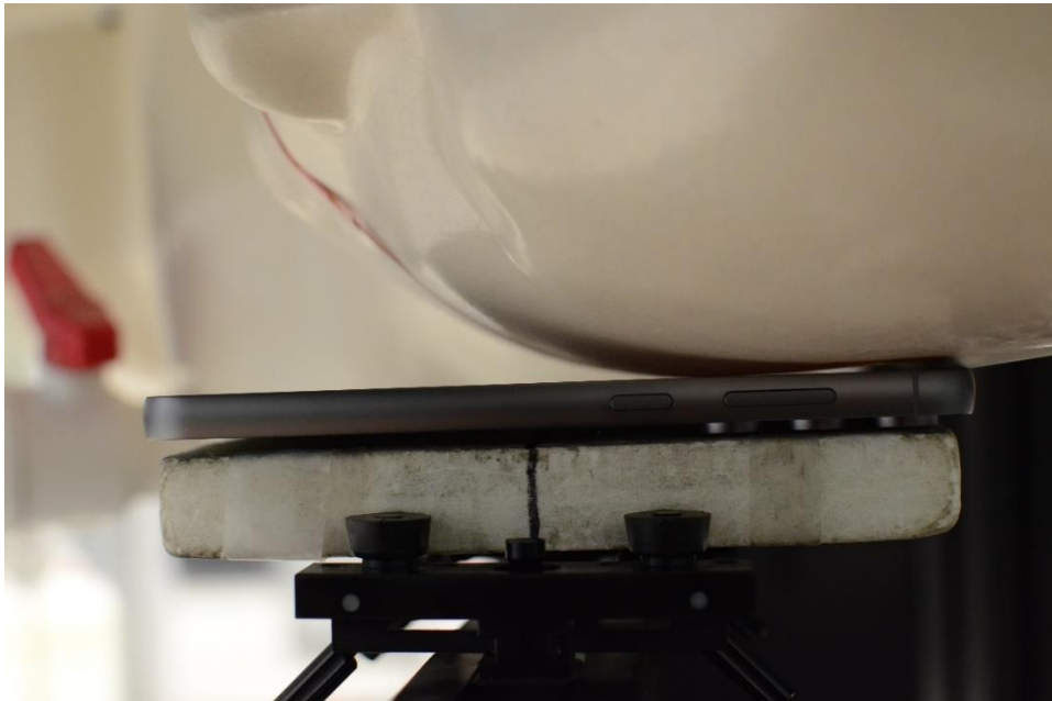
Test Setup Photo 13 – Head, Left, Cheek (Figure 7-6)
