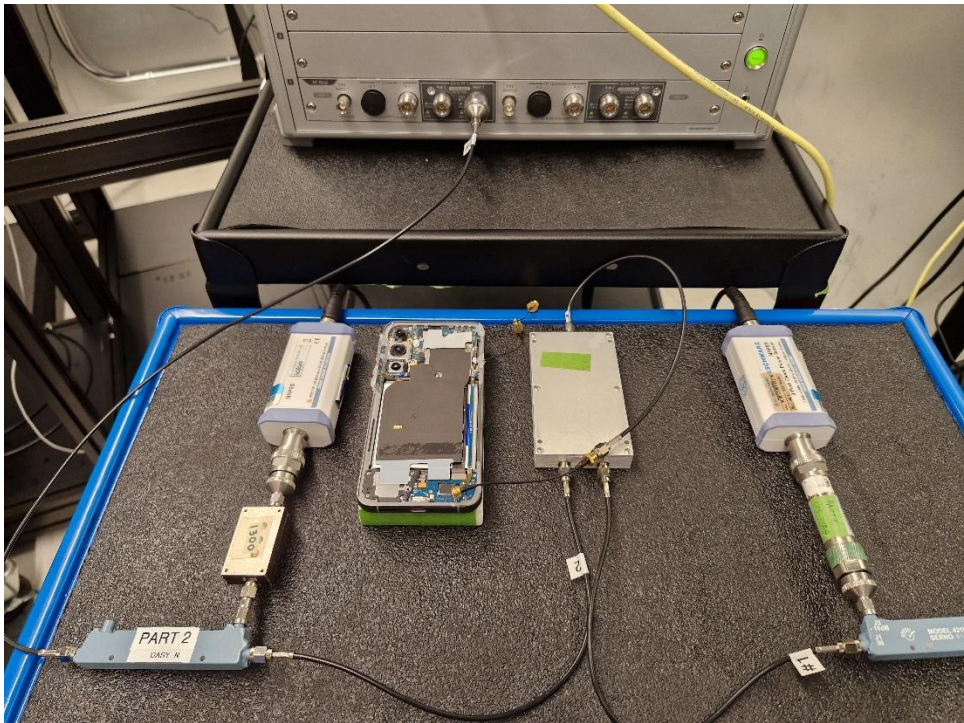
Test Setup Photo 6 – Conducted Test Setup (Figure 7-1c)
