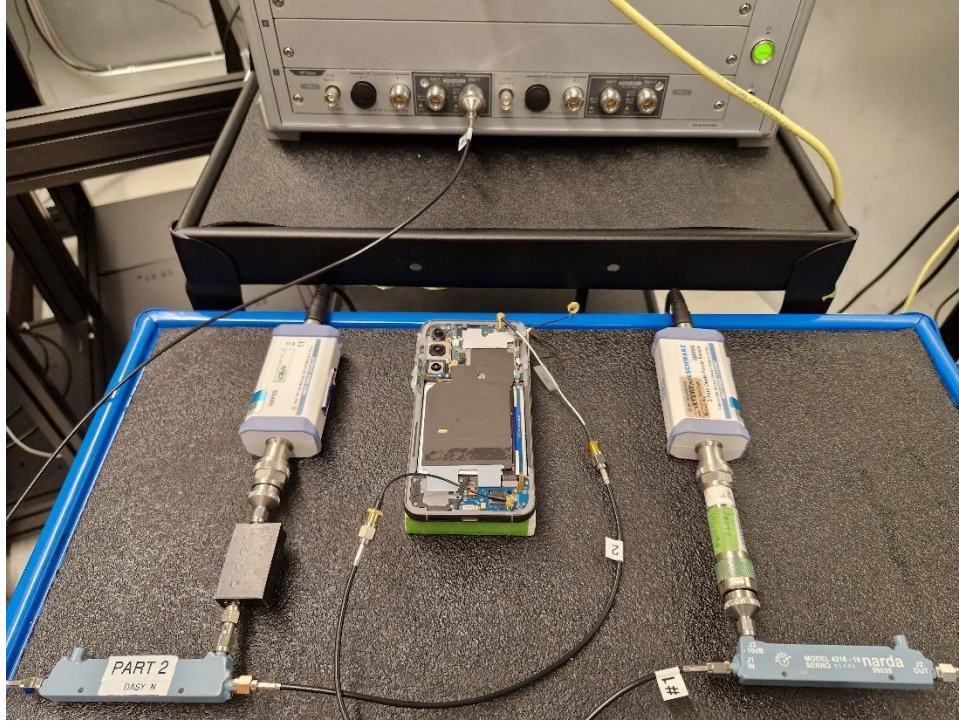
Test Setup Photo 7 – Conducted Test Setup (Figure 7-1d)
