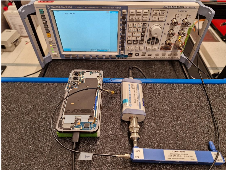
Test Setup Photo 11 – Conducted Test Setup (Figure 7-4)
