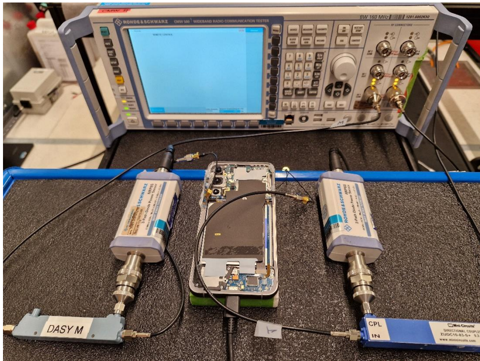
Test Setup Photo 12 – Conducted Test Setup (Figure 7-5)
