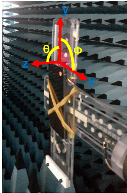
Figure 1: Geometry for SM-S711U for Radiation patterns.
