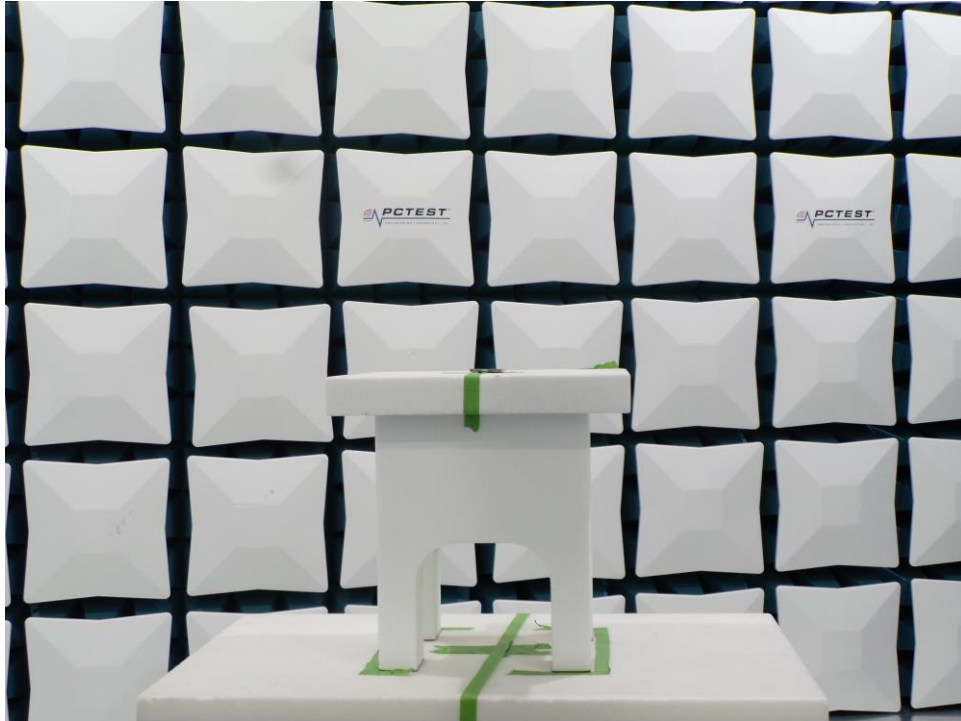
Figure 5. Test Setup – X Position – 1GHz-18GHz
