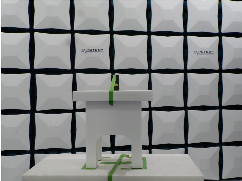
Figure 7. Test Setup – Z Position – 1GHz-18GHz
