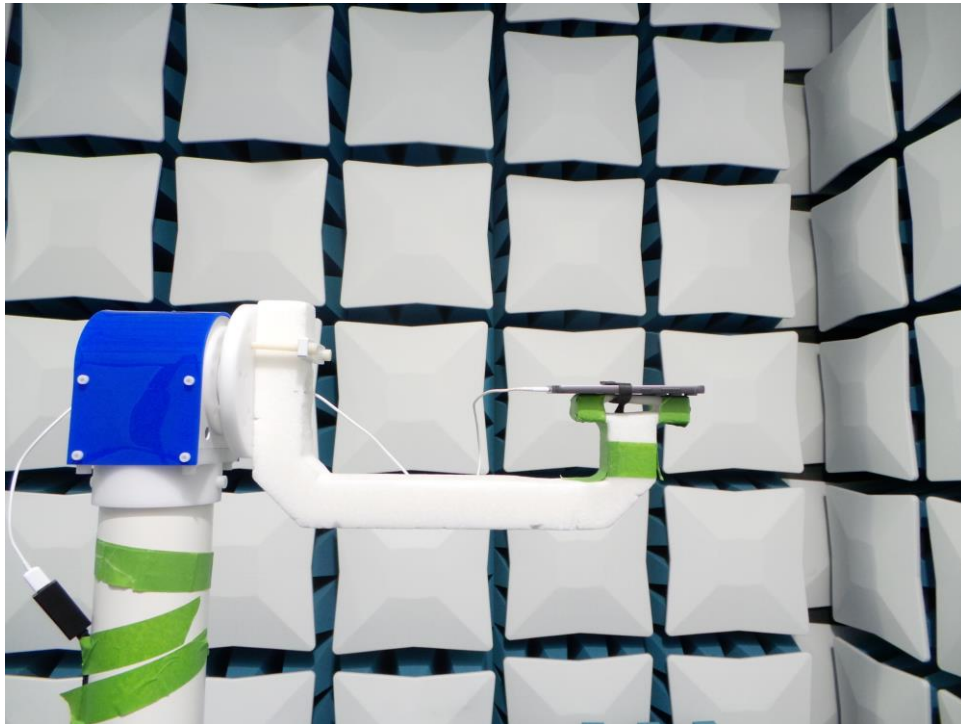
Figure 1. Test Setup – X Position – >18GHz
