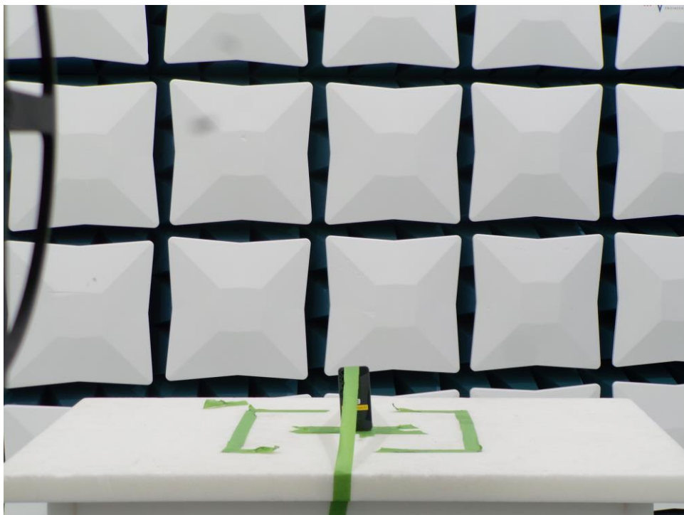
Figure 10. Test Setup – Z Position – 30MHz-1GHz
