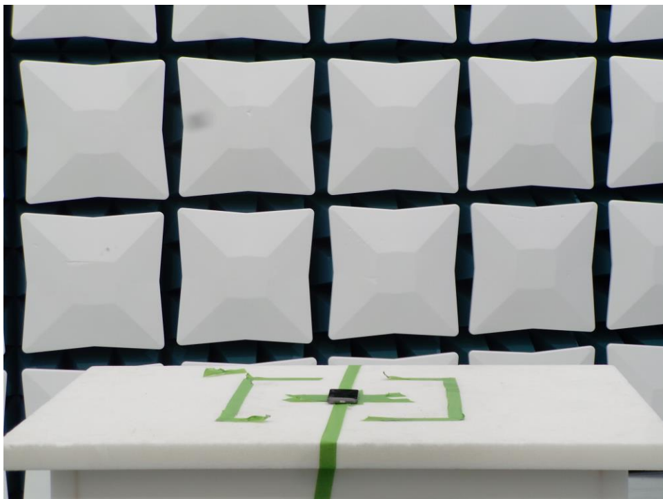
Figure 8. Test Setup – X Position – 30MHz-1GHz
