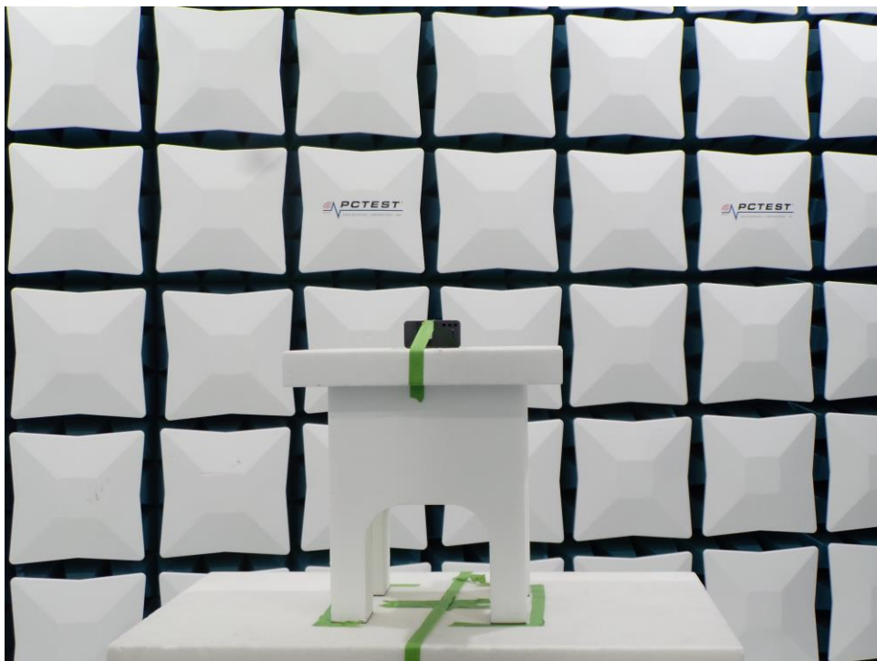
Figure 6. Test Setup – Y Position – 1GHz-18GHz
