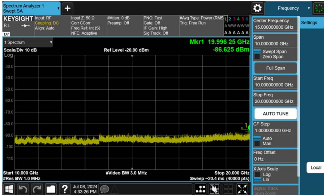
Sub6 n25(2)_15 M_Conducted Spurious(Above10 G)_Mid_BPSK_FullRB
