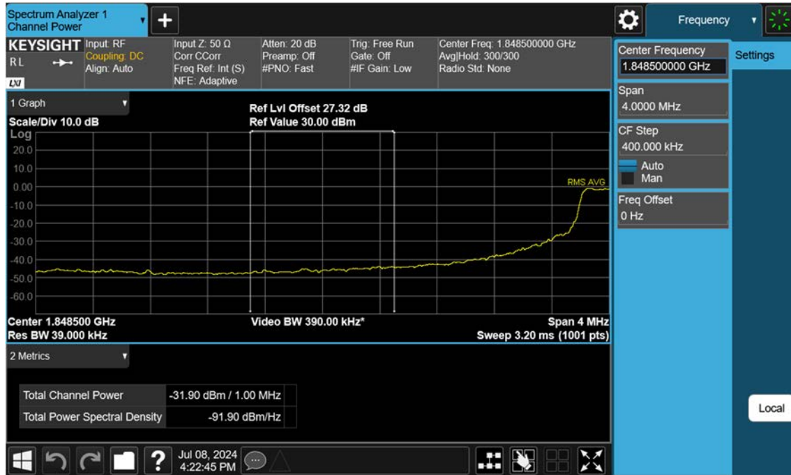
Sub6 n25(2)_10 M_Extended Band Edge_Low_BPSK_FullIRB
