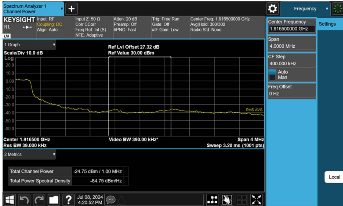
Sub6 n25(2)_5 M_Extended Band Edge_High_BPSK_FullIRB
