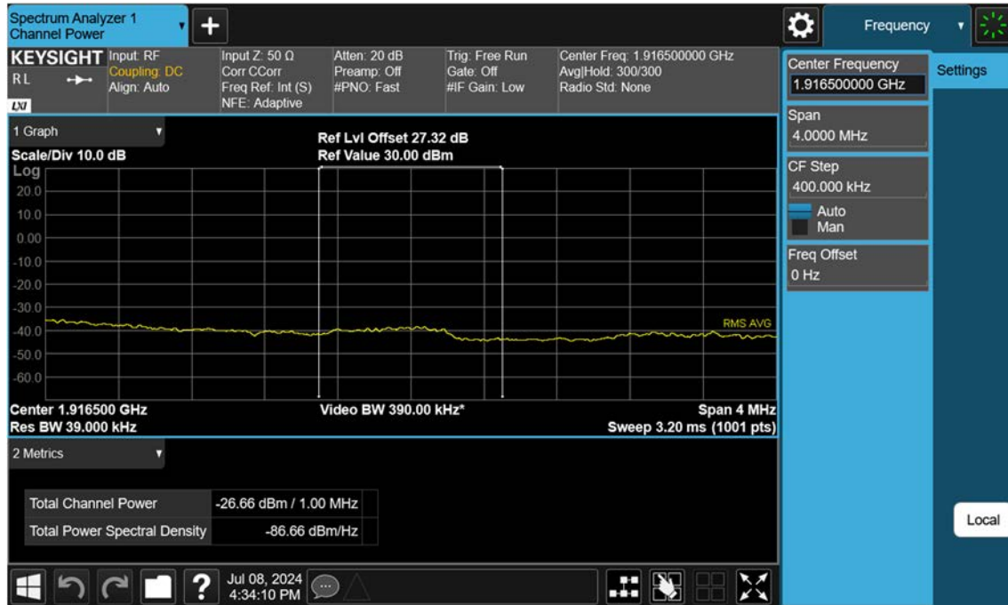
Sub6 n25(2)_15 M_Extended Band Edge_High_BPSK_FullIRB
