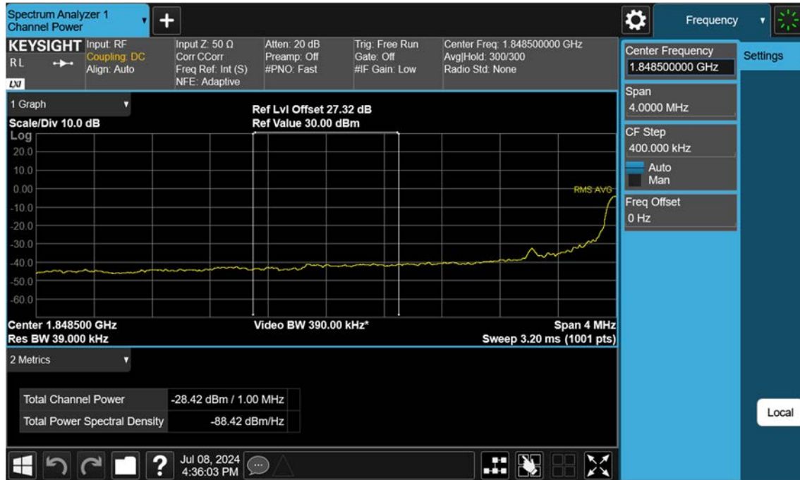
Sub6 n25(2)_20 M_Extended Band Edge_Low_BPSK_FullIRB
