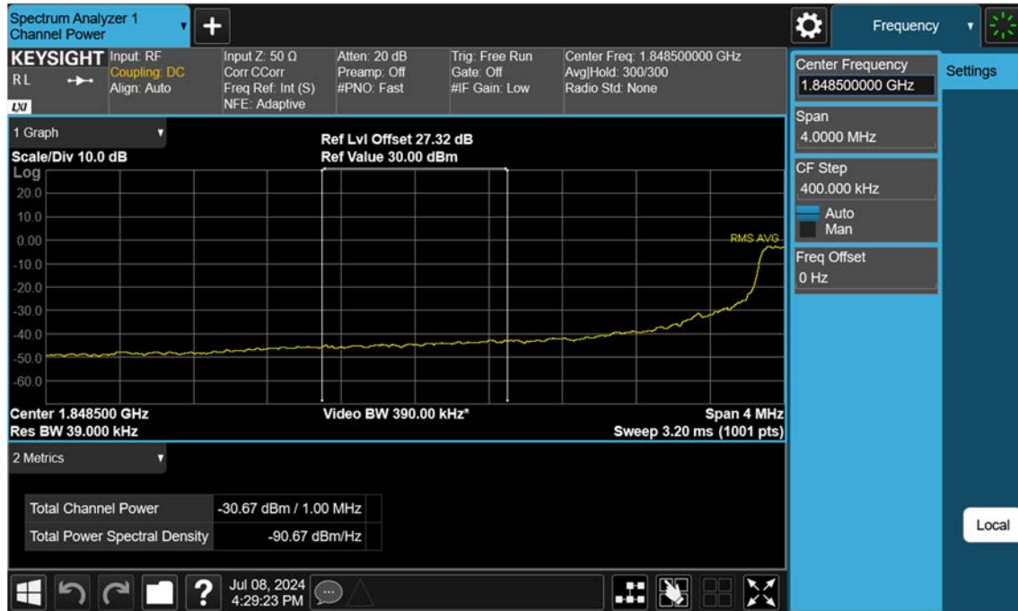
Sub6 n25(2)_15 M_Extended Band Edge_Low_BPSK_FullRB
