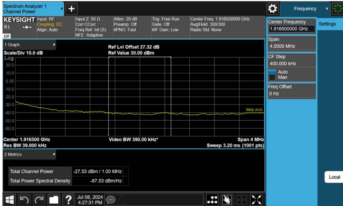
Sub6 n25(2)_10 M_Extended Band Edge_High_BPSK_FullIRB
