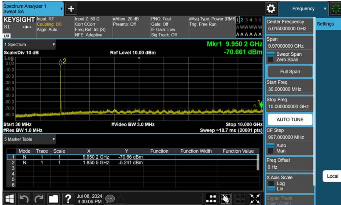
Sub6 n25(2)_15 M_Conducted Spurious(30 M-10 G)_Low_BPSK_1RB
