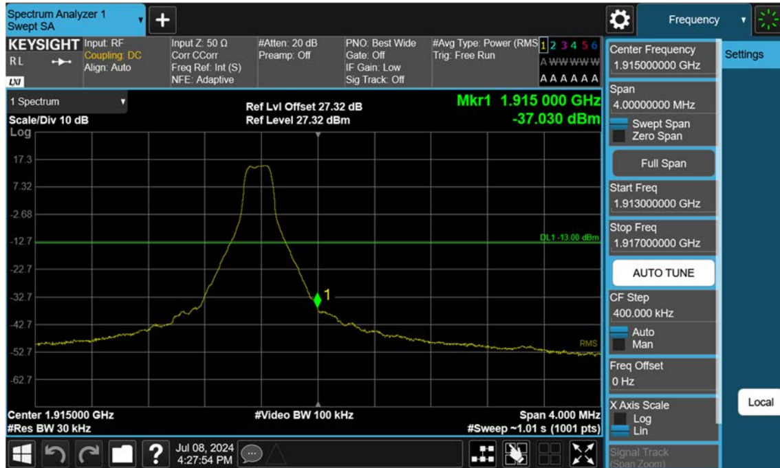
Sub6 n25(2)_10 M_Band Edge_High_BPSK_1RB
