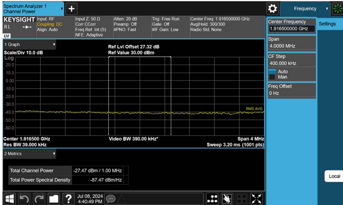
Sub6 n25(2)_20 M_Extended Band Edge_High_BPSK_FullIRB
