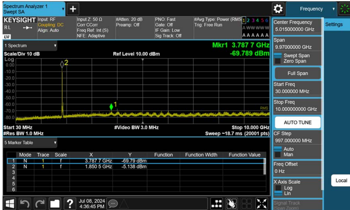
Sub6 n25(2)_20 M_Conducted Spurious(30 M-10 G)_Low_BPSK_1RB
