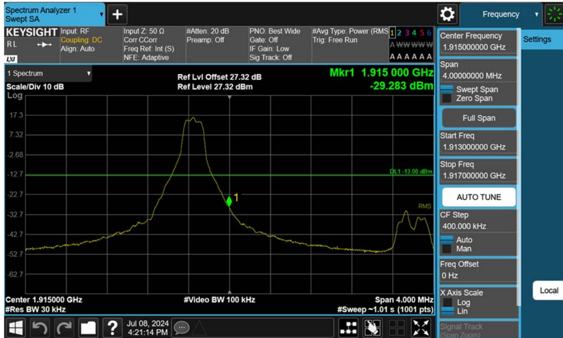
Sub6 n25(2)_5 M_Band Edge_High_BPSK_1RB
