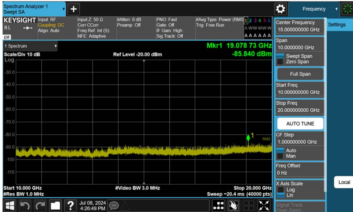
Sub6 n25(2)_10 M_Conducted Spurious(Above10 G)_Mid_BPSK_FullRB
