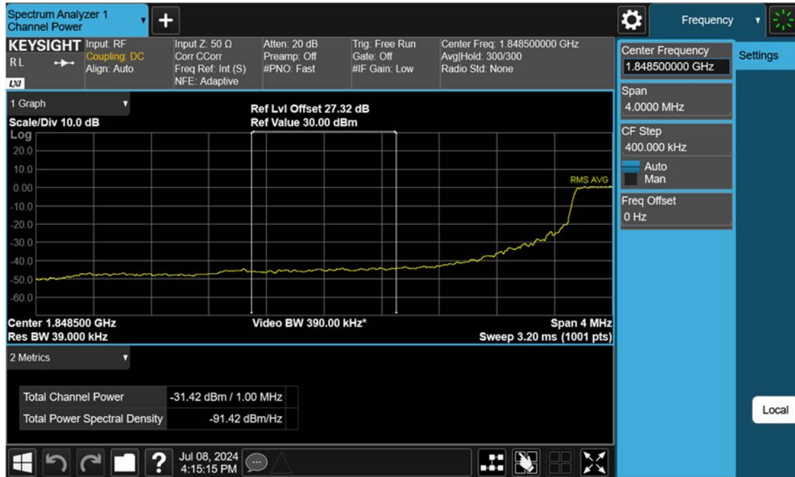
Sub6 n25(2)_5 M_Extended Band Edge_Low_BPSK_FullRB
