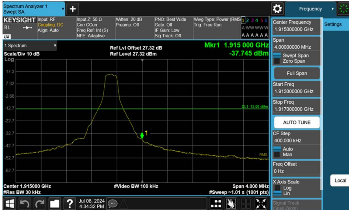
Sub6 n25(2)_15 M_Band Edge_High_BPSK_1RB
