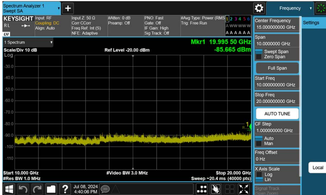
Sub6 n25(2)_20 M_Conducted Spurious(Above10 G)_Mid_BPSK_FullRB
