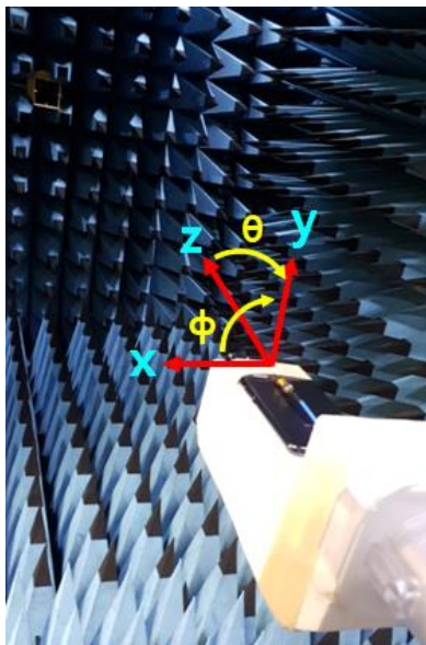
Figure 1: Geometry for SM-S721B/DS for Radiation patterns.
