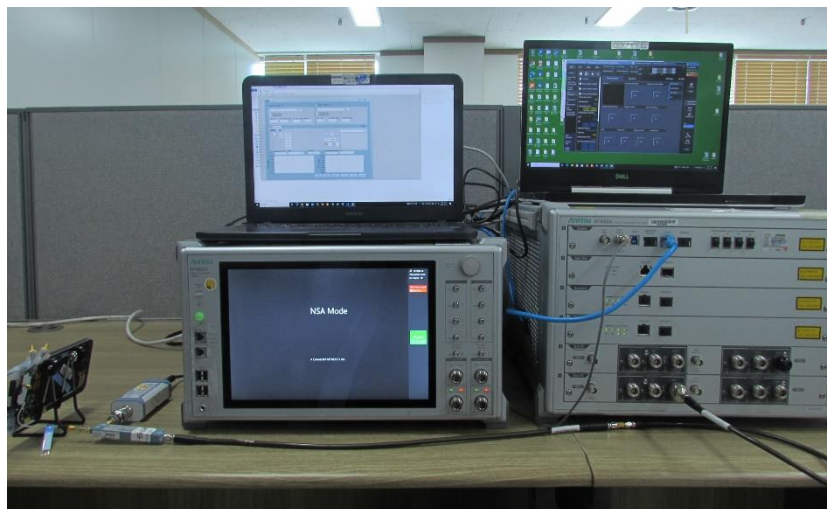
Test setup photo-2 TC02,06,14
