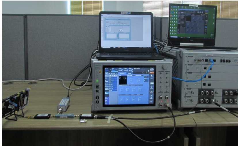
Test setup photo-3 TC11
