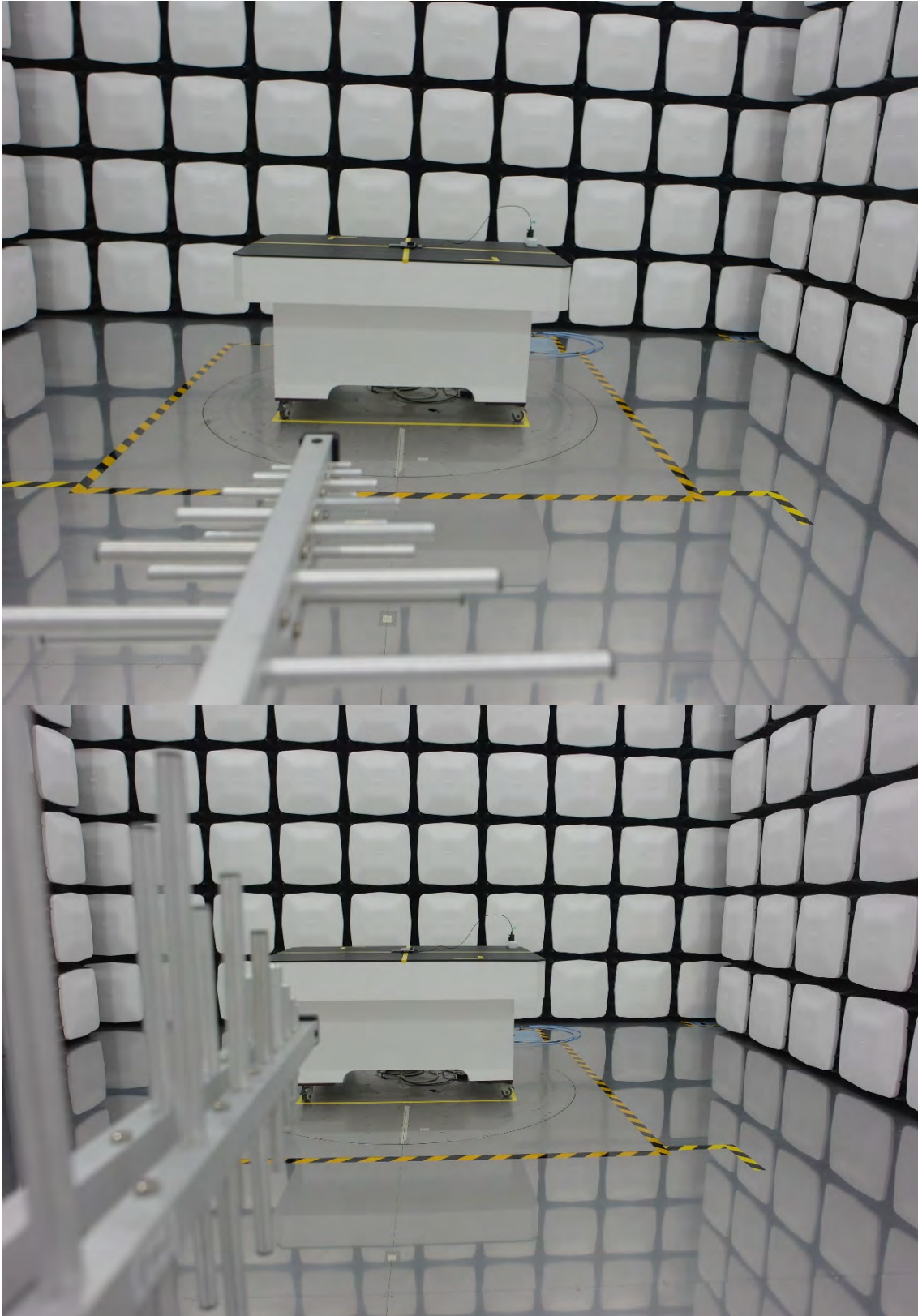
WPT Radiated Test Setup Photo for 30 MHz ~ 1 GHz :
