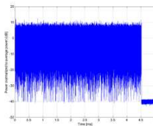
Time Domain
