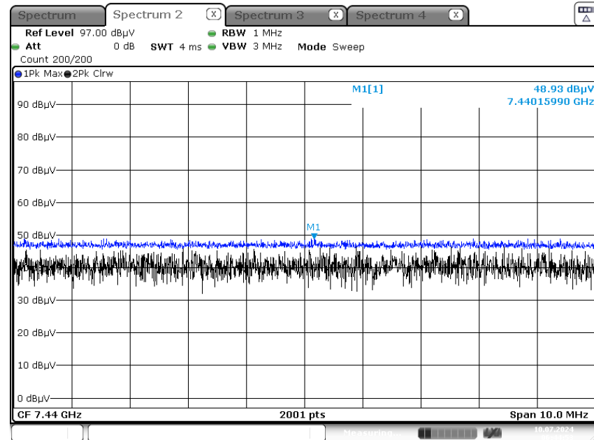
Radiated Spurious Emissions plot – Peak & Average Result (3rd Harmonic, Z-H)
