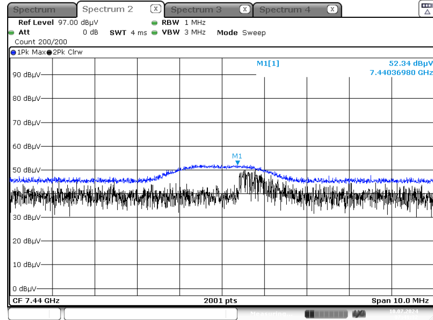
Radiated Spurious Emissions plot – Peak & Average Result (3rd Harmonic, Y-V)
