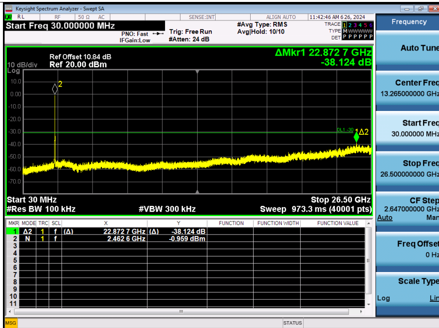
[ANT. 2] 802.11n (HT20)_Ch.11_MCS0
