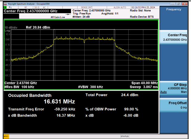
802.11ac_VHT20-CH 6
