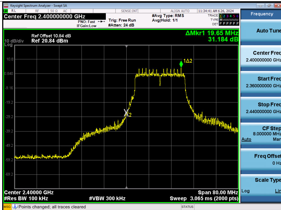
[ANT. 2] 802.11n_HT20-CH 1
