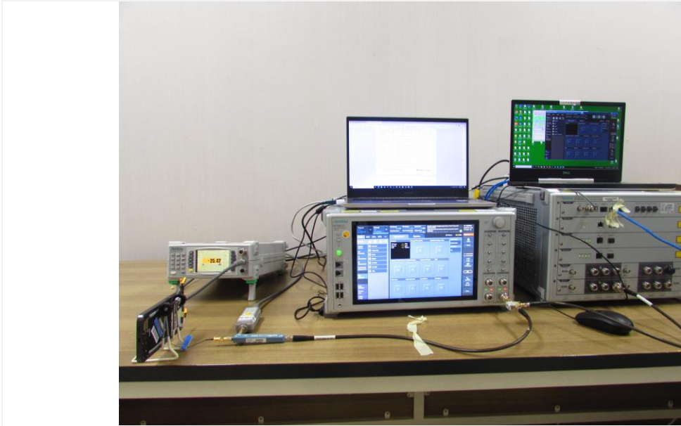
Test setup photo-3 TC11
