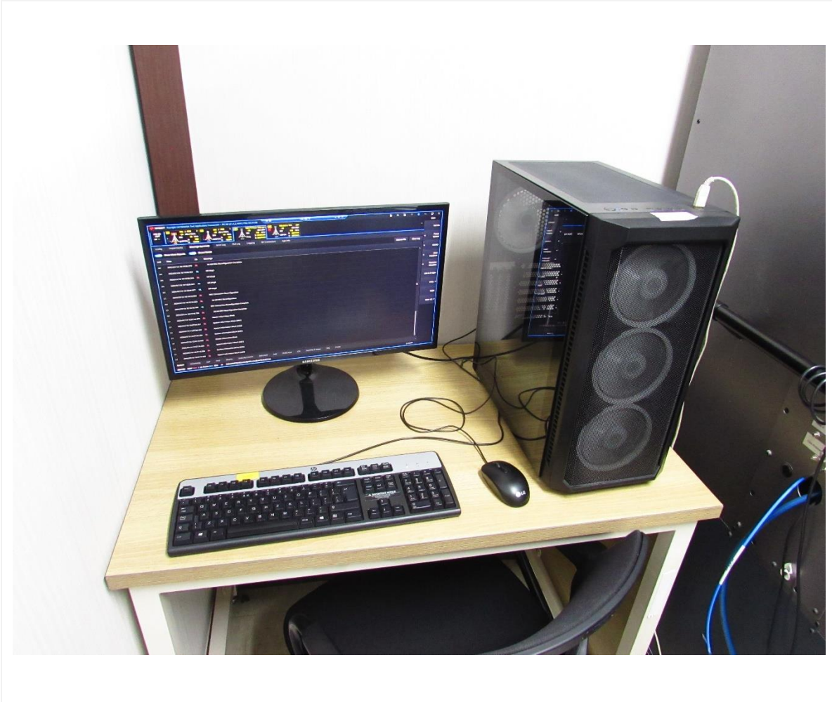
Test setup photo 6-2 mmW NR radiated power measurement
