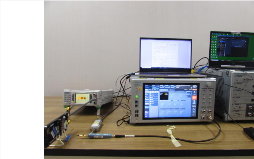
Test setup photo-1 TC01,03,04,05,07,08,09,10,15
