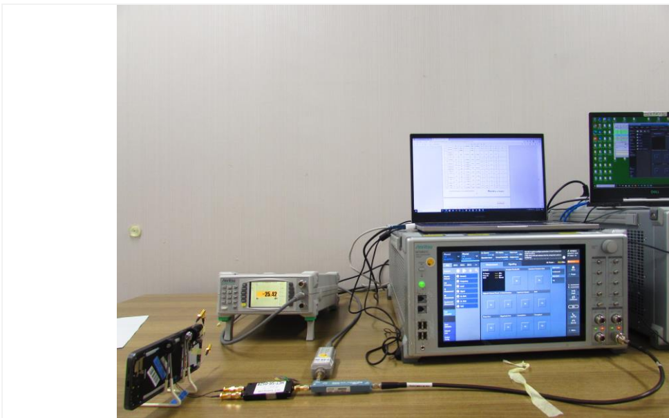
Test setup photo-4 TC12
