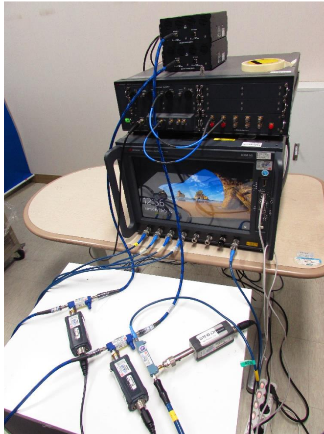
Test setup photo 6-1 mmW NR radiated power measurement
