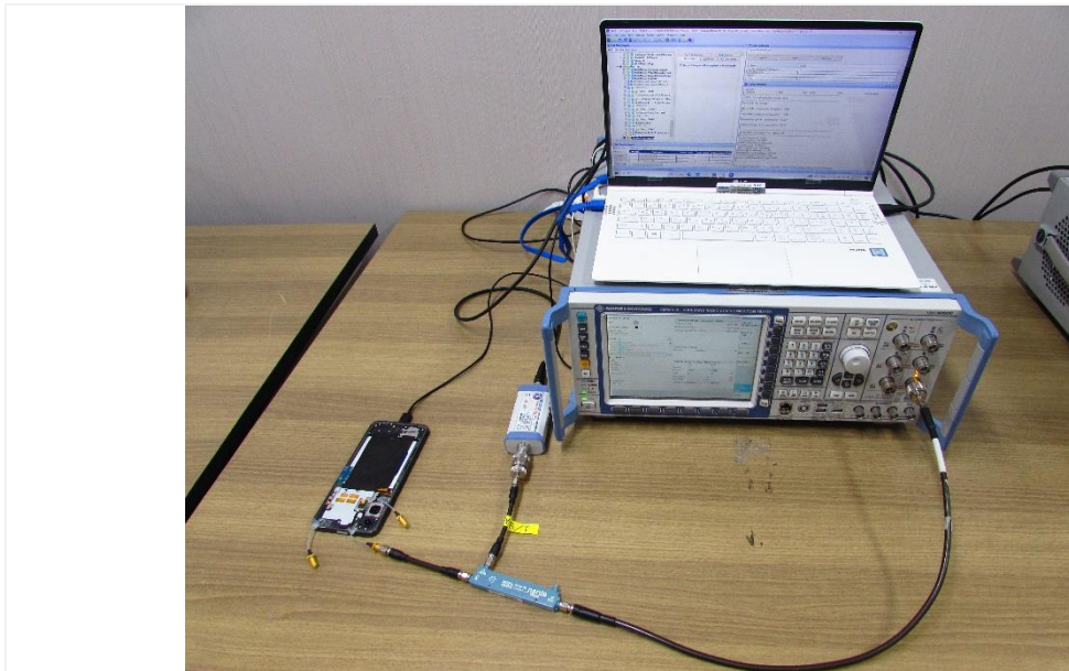
Test setup photo-1 (7-1(a) WLAN Time-varying Tx Power Transmission, Change in Call, Change in DSI)
