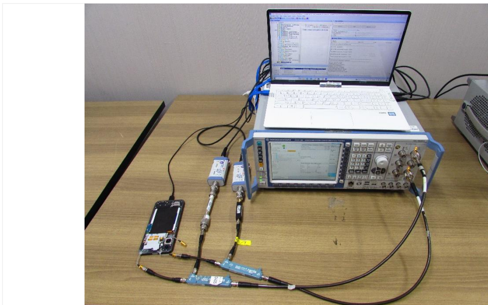
Test setup photo-2 (7-1(b) WLAN SAR1 vs SAR2 (DBS)/ WLAN Ant Switch)
