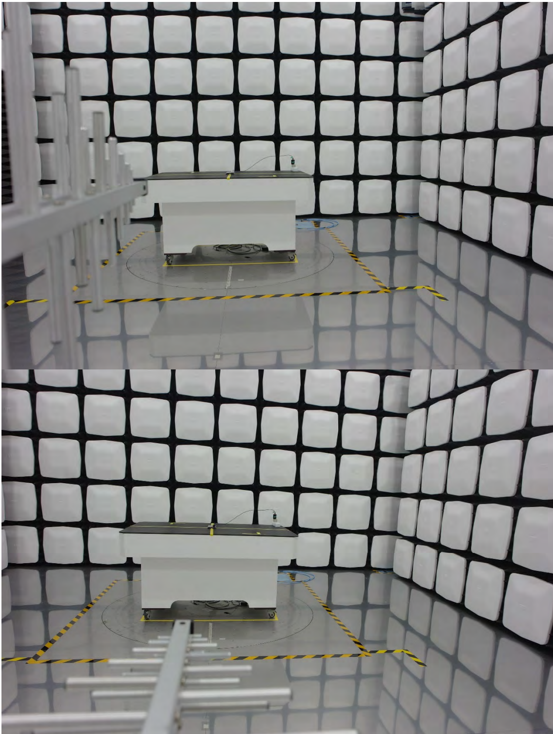
WPT Radiated Test Setup Photo for 30 MHz ~ 1 GHz :
