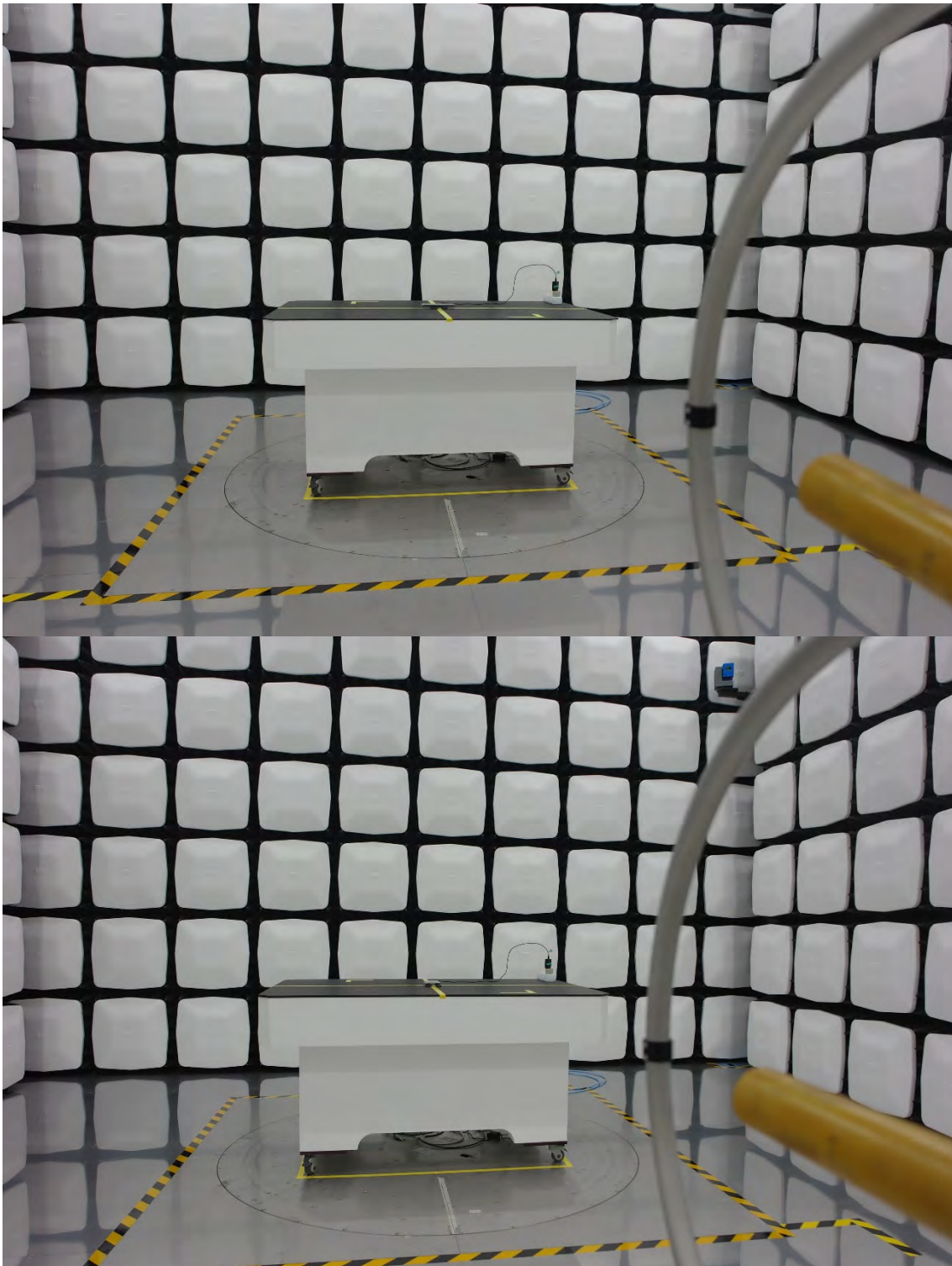
WPT Radiated Test Setup Photo for below 30 MHz:
