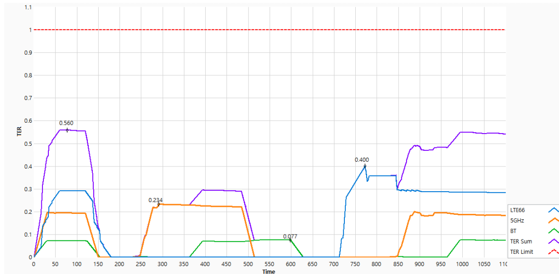
Figure 11.10-3 Total Exposure Ratio in C-TC01
