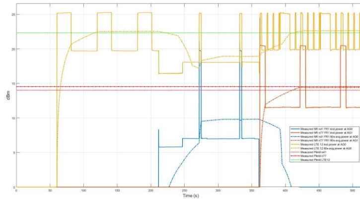
Figure 11.9-1 Conducted Transmitted power for LTE B12(AG0) and NR n41(AG0), n77(AG1) in Test TC14
