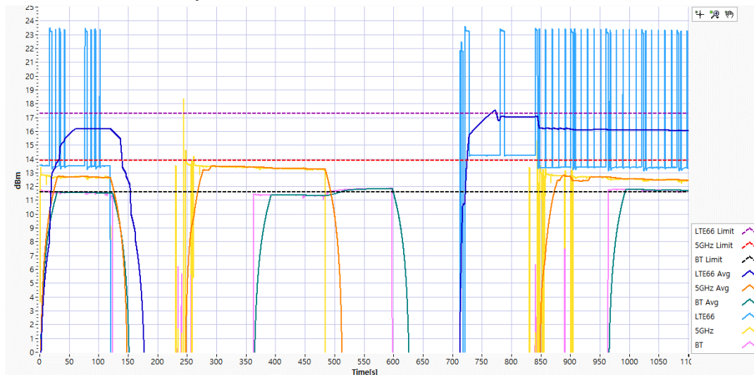
Figure 11.10-1 Conducted Tx power in LTE /WLAN 5G/Bluetooth in test C-TC 01
