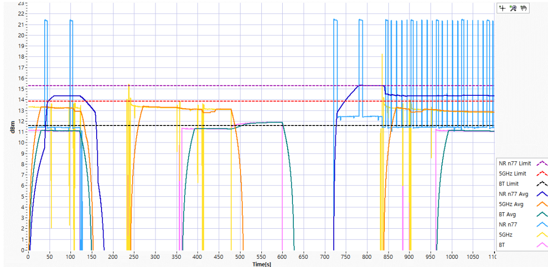
Figure 11.10-4 Conducted Tx power in NR/WLAN 5G/Bluetooth in test C-TC02
