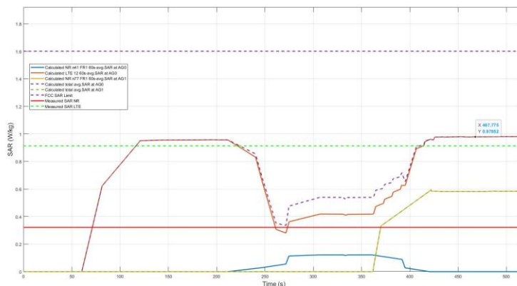
Figure 11.9-2 Total time-averaged SAR in TC14
