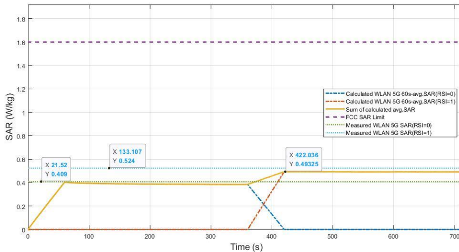
Figure 11.3-20 Total time-averaged SAR in WTC01
