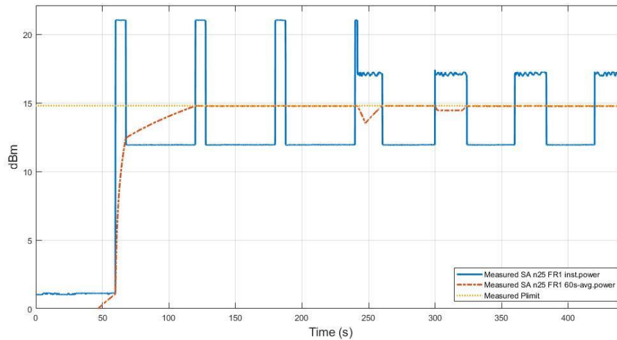
Figure 11.3-3 Time average conducted power of NR n25 in TC02
