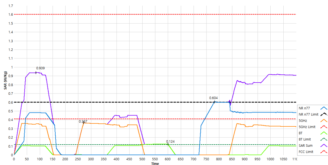
Figure 11.10-5 Time-averaged SAR in C-TC02
