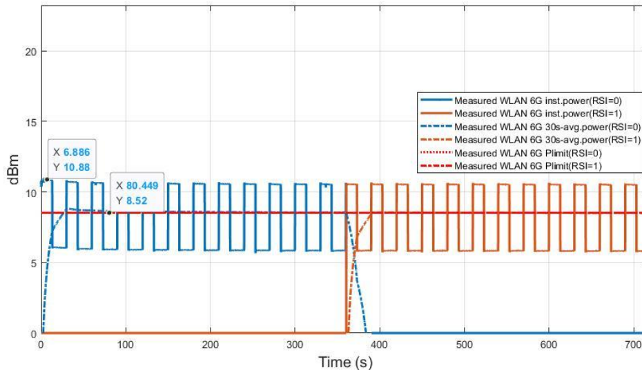
Figure 11.3-21 Conducted Tx power for WLAN 6GHz in WTC03
