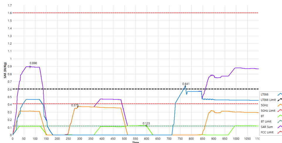
Figure 11.10-2 Time-averaged SAR in C-TC01
