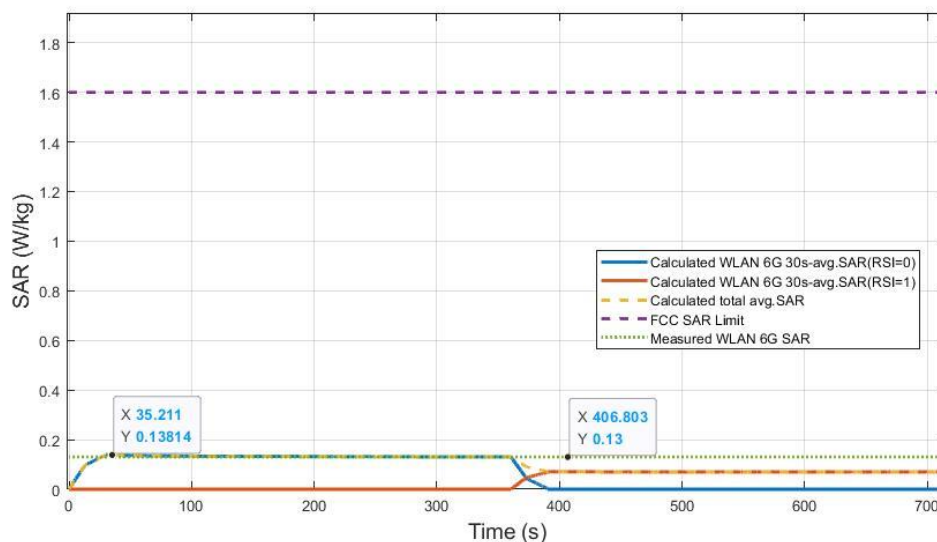
Figure 11.3-22 Total time-averaged SAR in WTC01
