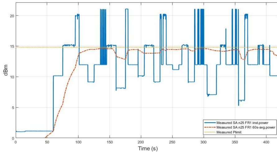
Figure 11.3-11 Conducted Tx power of NR n25 in TC06
