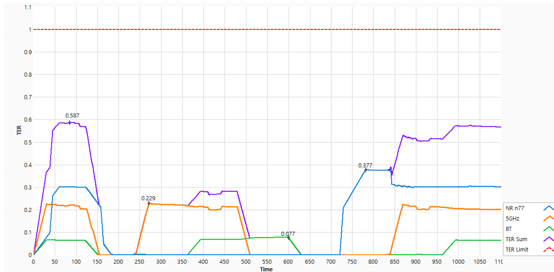
Figure 11.10-6 Total Exposure Ratio in C-TC02
