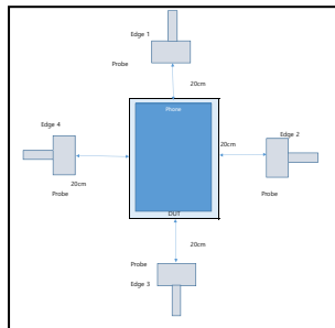
DUT to phone test Configuration 1 & 2
