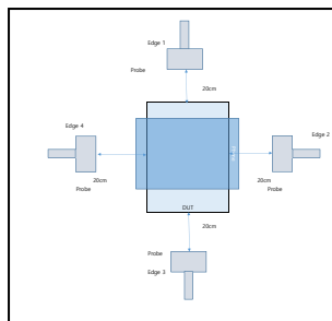
DUT to phone test Configuration 3 & 4
