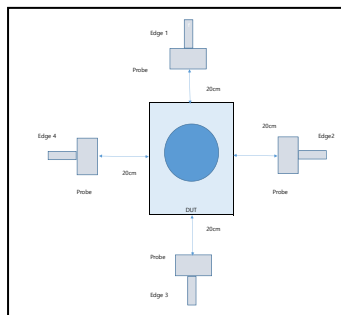
DUT to Watch/Ear buds test Configuration 5 & 6 and 7 & 8
