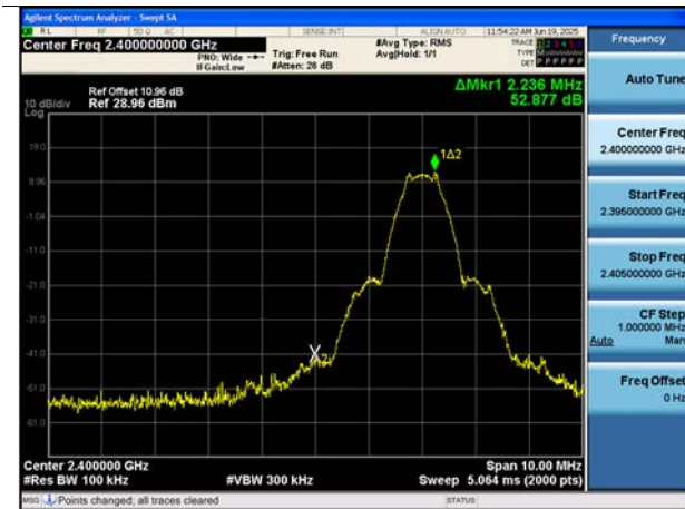
Dual Ant.1, 1 MBit/s 255 Byte (Low-CH 37)
