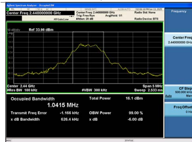
125k Bit/s 255 Byte (Low-CH 17)
