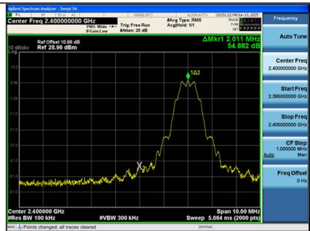
Dual Ant.2, 1 MBit/s 255 Byte (Low-CH 37)
