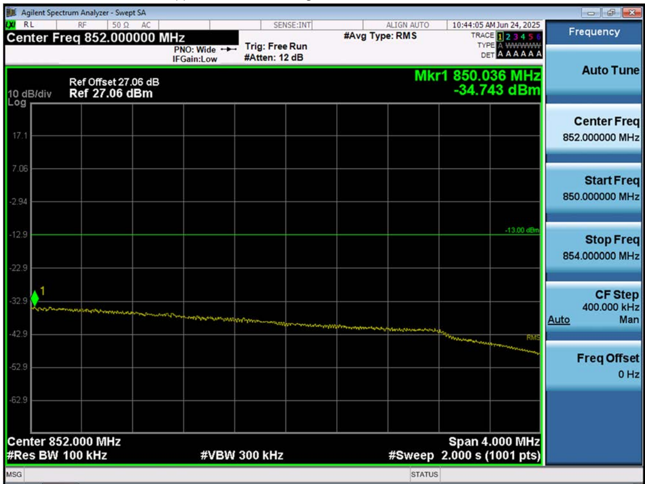
LTE B26_Upper Extended Band Edge Plot (5 M BW Ch.27015 QPSK_RB25_0)
