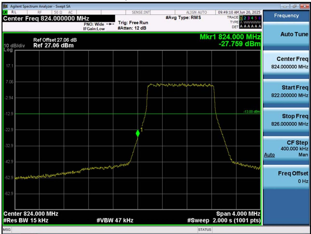
LTE B26_Lower Band Edge Plot (1.4 M BW Ch.26797 QPSK_RB6_Offset 0)
