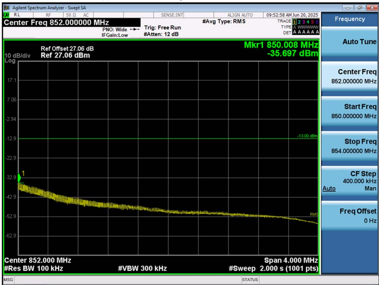
LTE B26_Upper Extended Band Edge Plot (1.4 M BW Ch.27033 QPSK_RB6_0)
