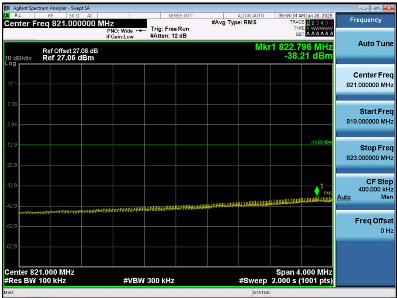
LTE B26_Lower Extended Band Edge Plot (3 M BW Ch.26805 QPSK_RB15_0)
