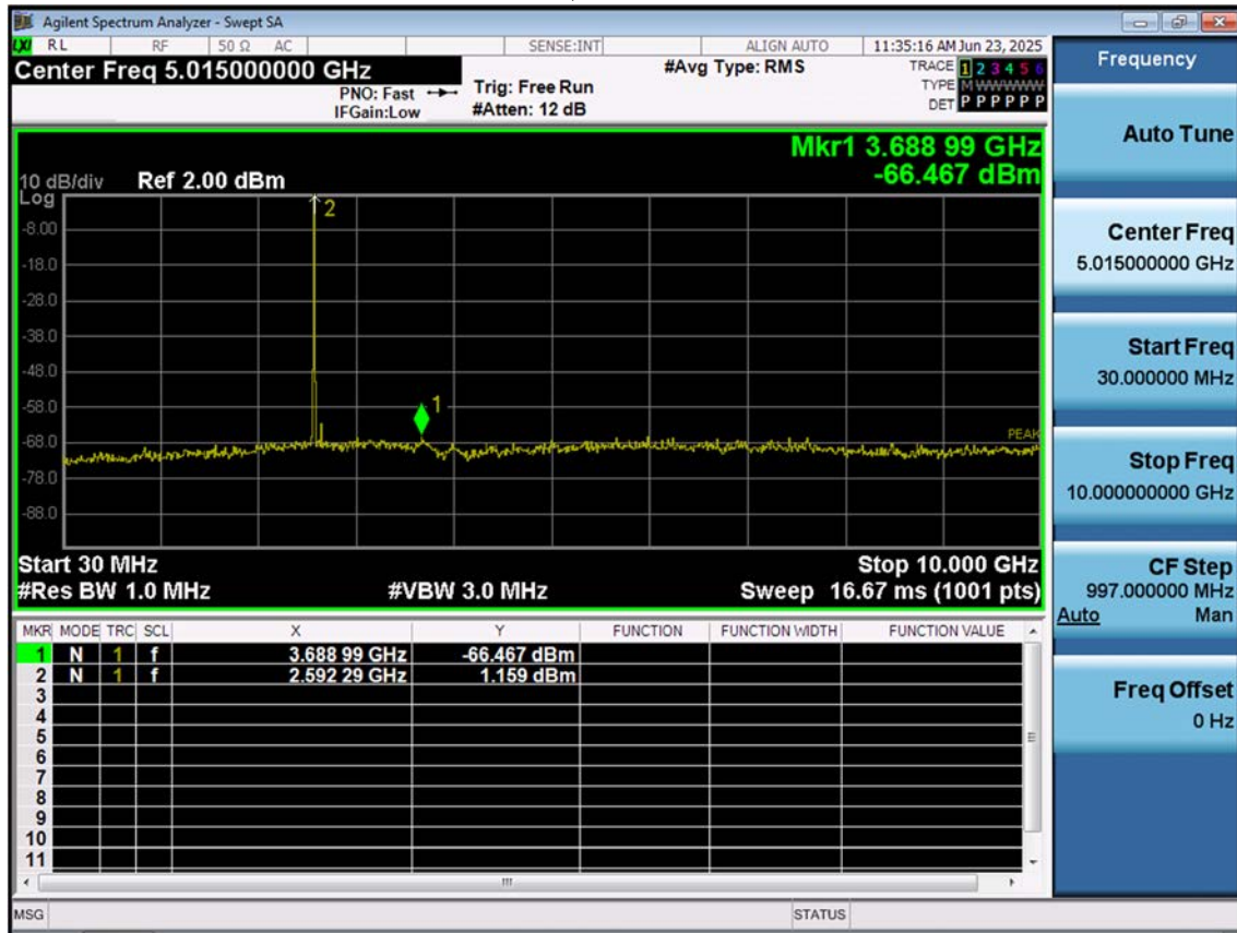
LTE B41_5 M_Conducted Spurious(30 M-10 G)_Mid_QPSK_1RB
