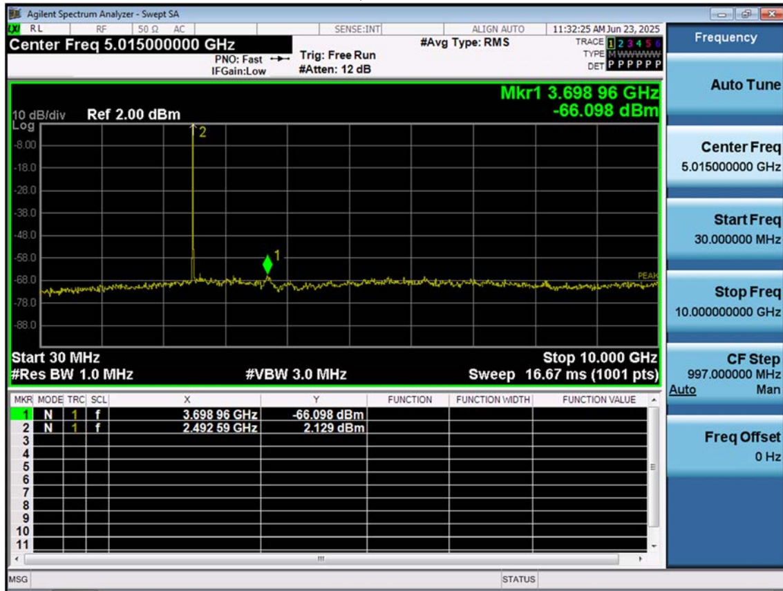
LTE B41_5 M_Conducted Spurious(30 M-10 G)_Low_QPSK_1RB
