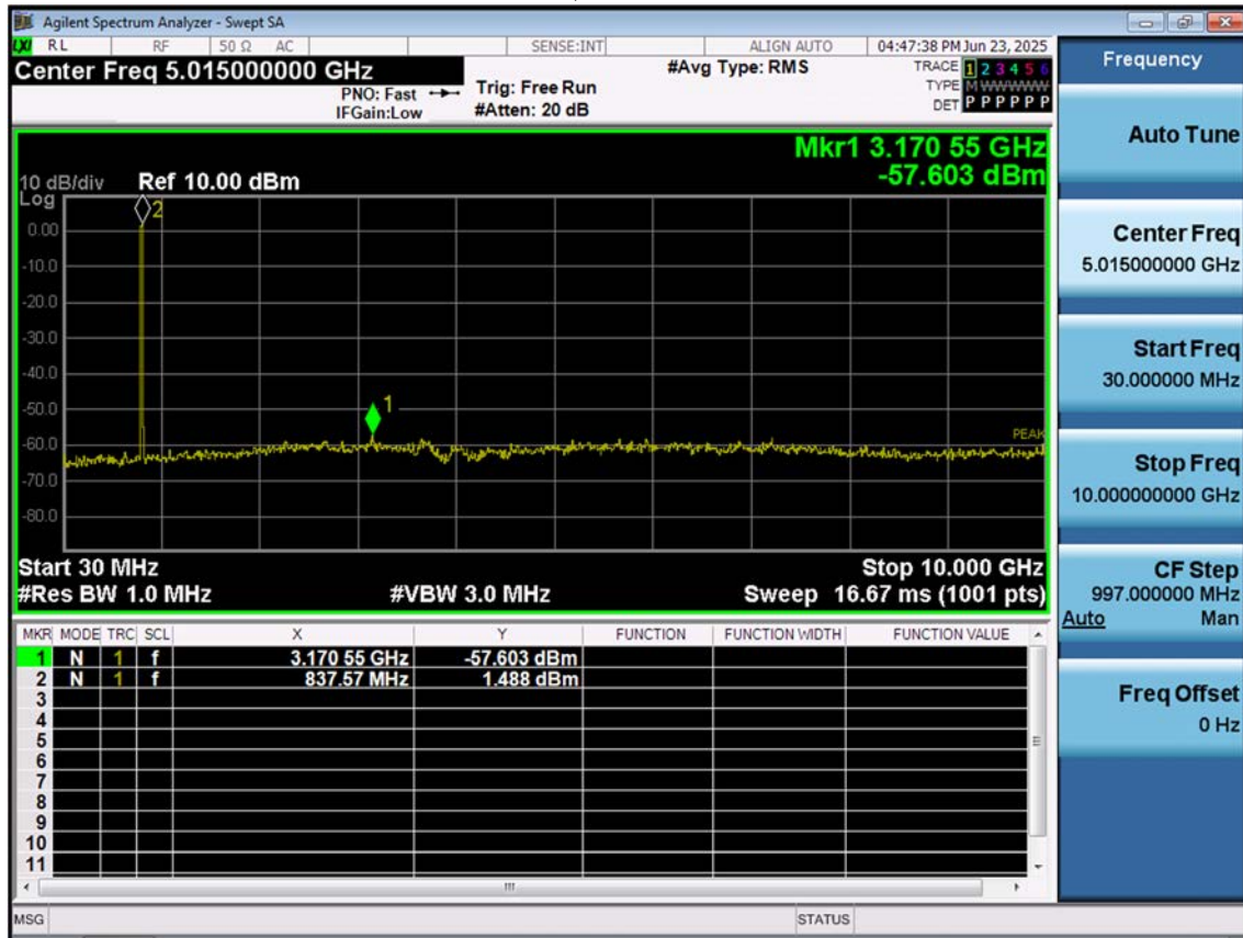
LTE B5_10 M_Conducted Spurious(30 M-10 G)_Mid_QPSK_1RB
