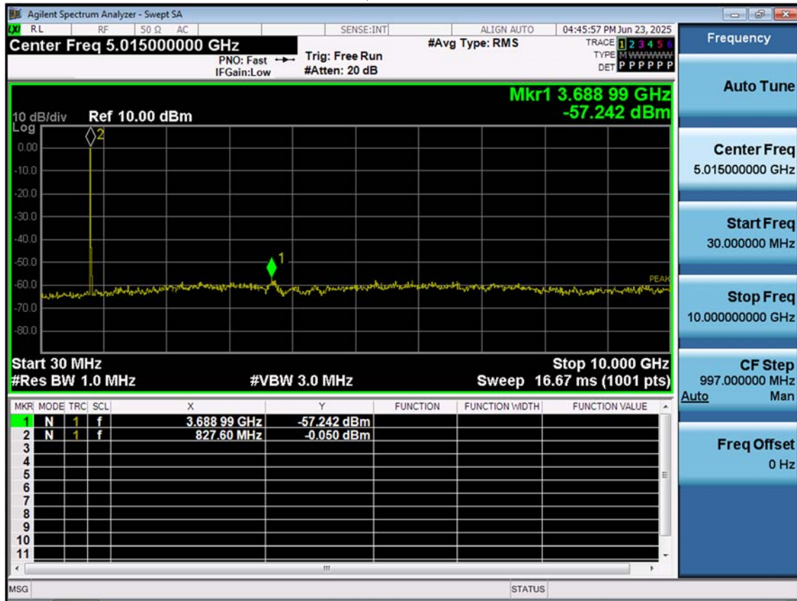
LTE B5_10 M_Conducted Spurious(30 M-10 G)_Low_QPSK_1RB
