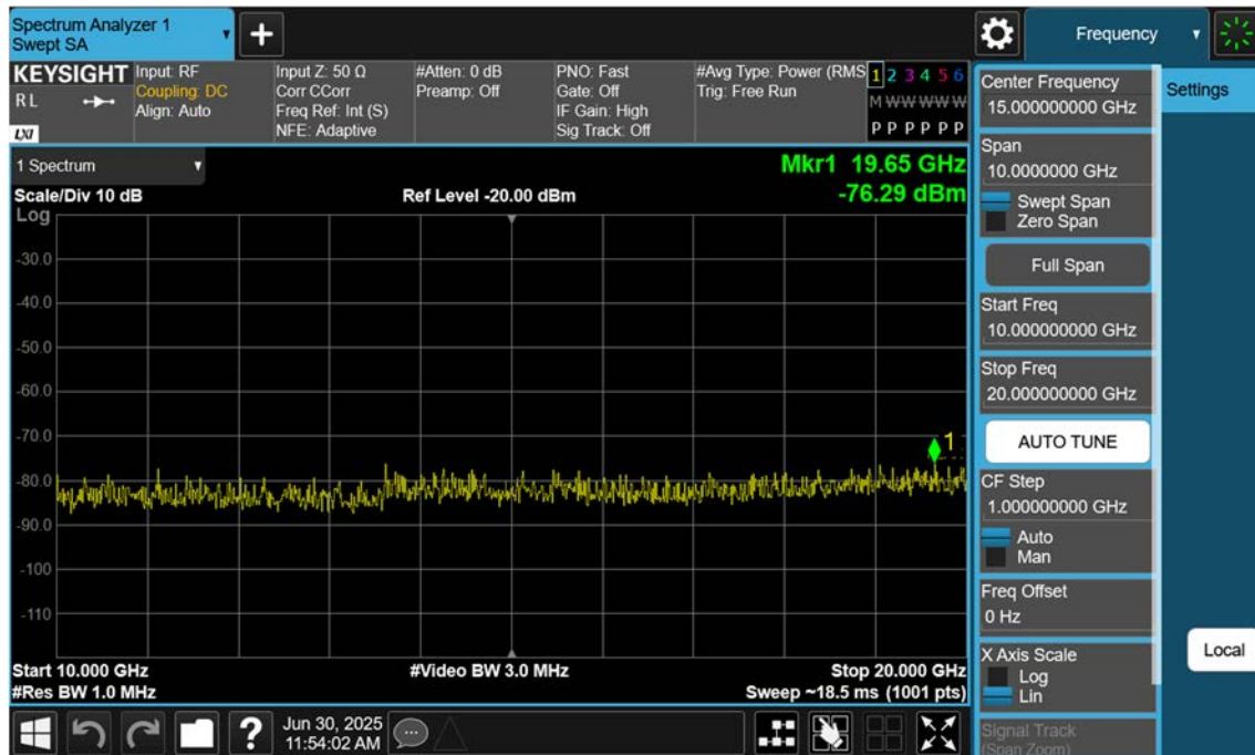
NR25_15 M_Conducted Spurious(Above10 G)_Mid_BPSK_1RB
