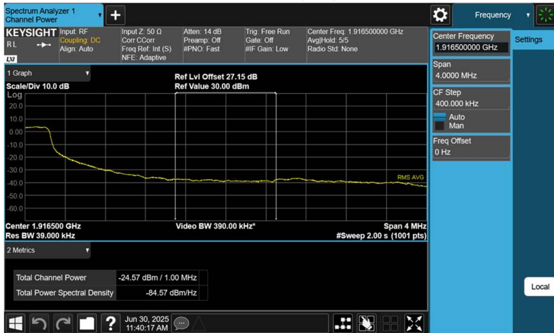
NR25_5 M_Extended Band Edge_High_BPSK_FullRB
