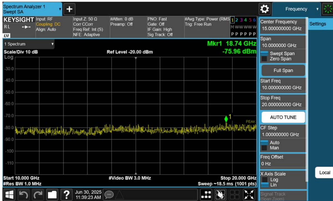
NR25_5 M_Conducted Spurious(Above10 G)_Mid_BPSK_1RB
