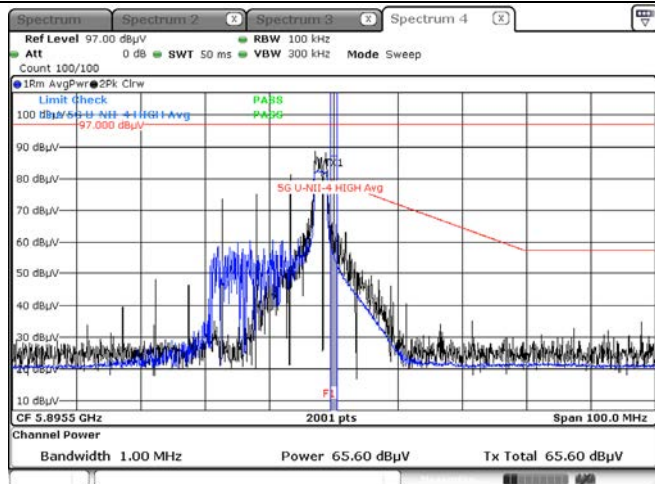
Average result (802.11ax(HE20) Ch.177, 106T RU 54)
