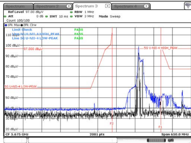
Peak result (802.11ax(HE80) Ch.171, 106T RU 53)
