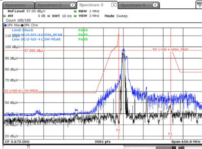
Peak result (802.11ax(HE160_80L) Ch.163, 484T RU 65)
