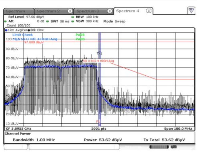
Average result (802.11ax(HE40) Ch.175, SU)
