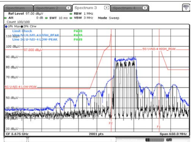
Peak result (802.11ax(HE160_80L) Ch.163, 996T RU 67)
