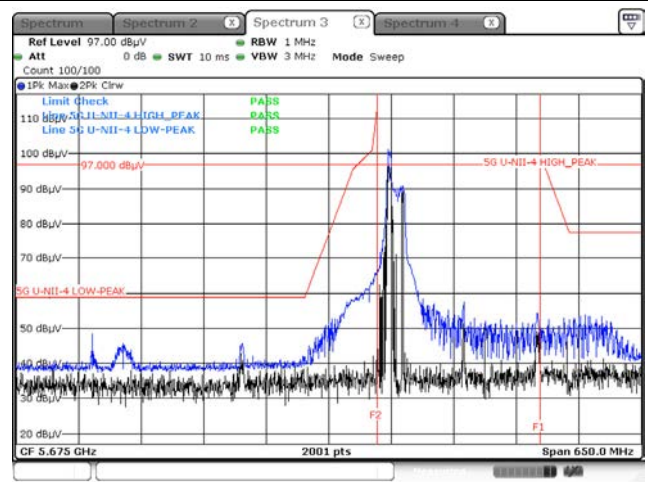
Peak result (802.11ax(HE160_80L) Ch.163, 242T RU 61)
