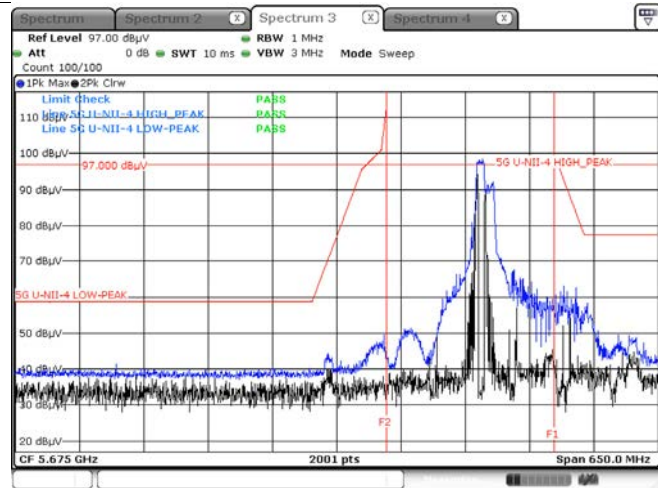
Peak result (802.11ax(HE80) Ch.171, 484T RU 65)
