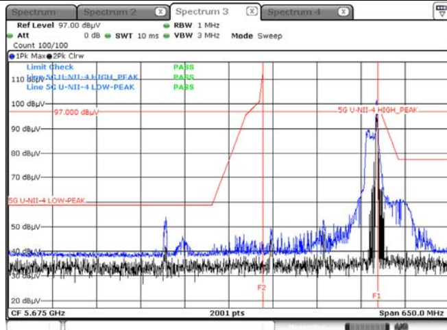
Peak result (802.11ax(HE160_80U) Ch.163, 106T RU 60)
