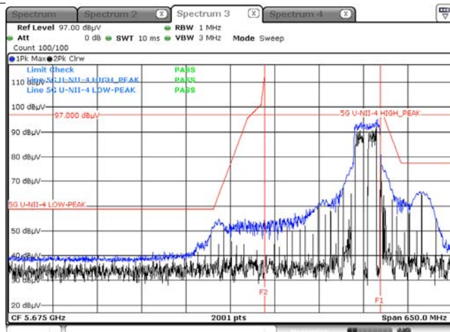
Peak result (802.11ax(HE160_80U) Ch.163, 484T RU 66)
