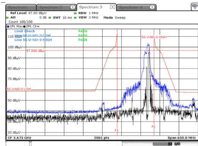
Peak result (802.11ax(HE20) Ch.165, SU)
