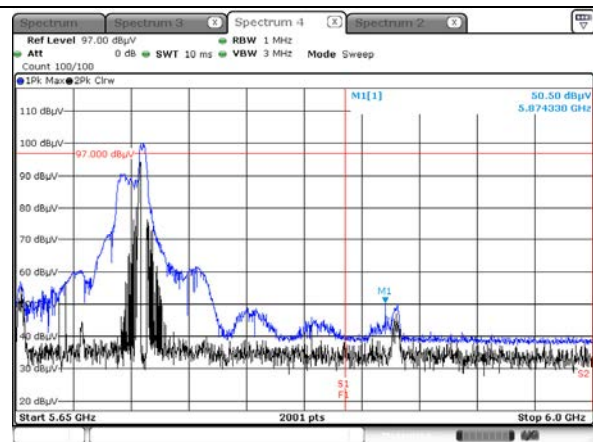
Peak result (802.11ax(HE80) Ch.138, 242T RU 64)
