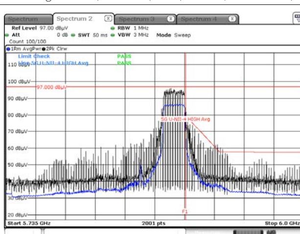
Average result (802.11ax(HE80) Ch.171, 242T RU 64)
