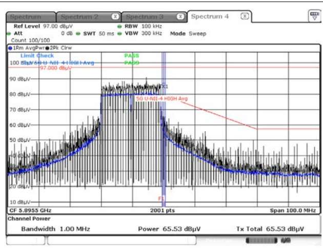
Average result (802.11ax(HE20) Ch.177, 242T RU 61)
