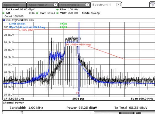
Average result (802.11ax(HE20) Ch.177, SU)
