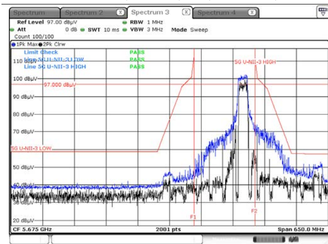
Peak result (802.11ax(HE20) Ch.165, SU)
