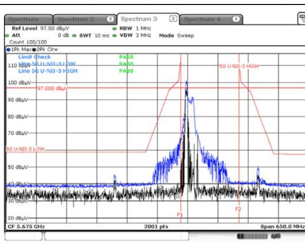
Peak result (802.11ax(HE20) Ch.149, 242T RU 61)
