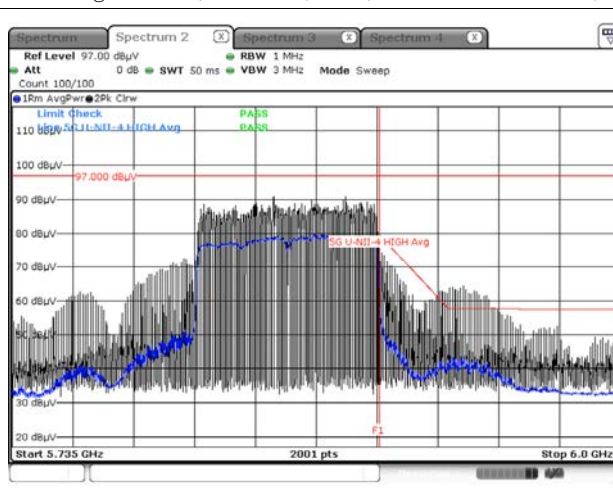
Average result (802.11ax(HE80) Ch.171, 996T RU 67)
