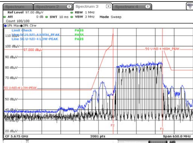
Peak result (802.11ax(HE160) Ch.163, 2x996T RU 68)
