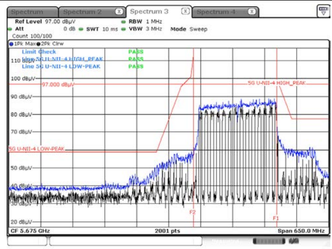
Peak result (802.11ax(HE160) Ch.163, SU)
