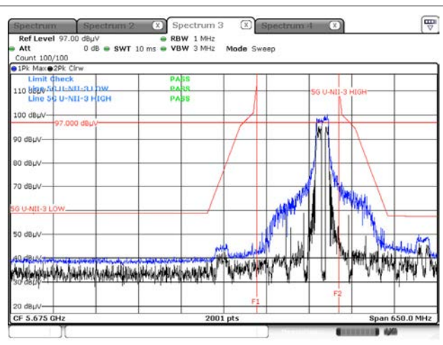
Peak result (802.11ax(HE20) Ch.165, 242T RU 61)
