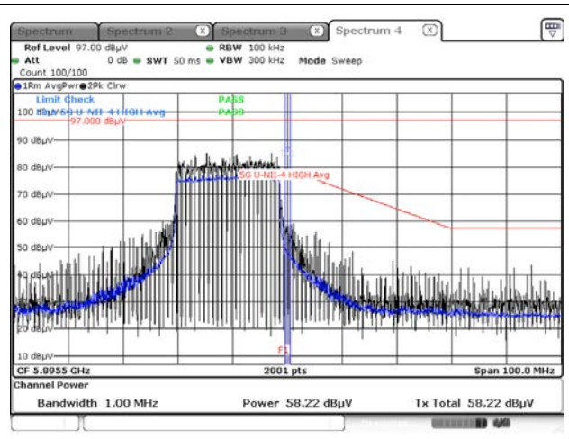
Average result (802.11ax(HE40) Ch.175, 242T RU 62)
