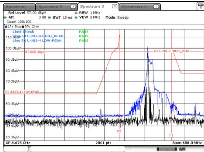
Peak result (802.11ax(HE40) Ch.167, 106T RU 53)
