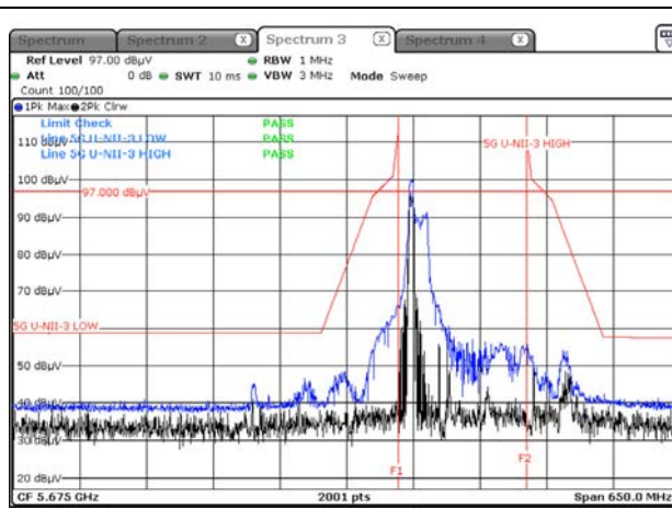
Peak result (802.11ax(HE80) Ch.155, 52T RU 37)
