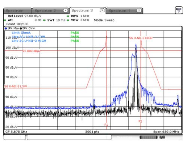
Peak result (802.11ax(HE20) Ch.165, 52T RU 40)
