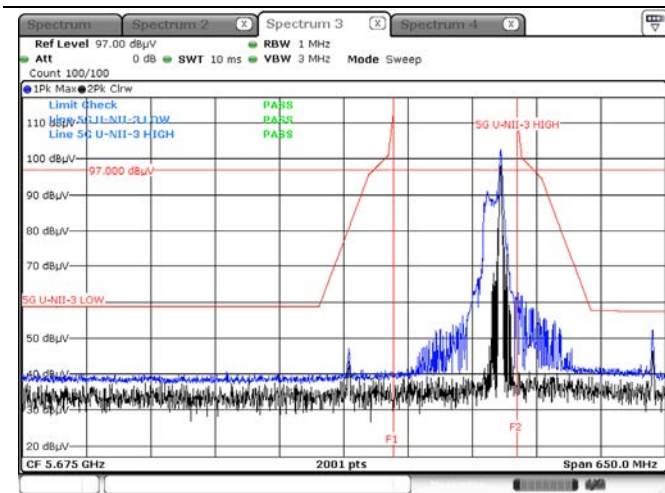
Peak result (802.11ax(HE20) Ch.165, 26T RU 8)
