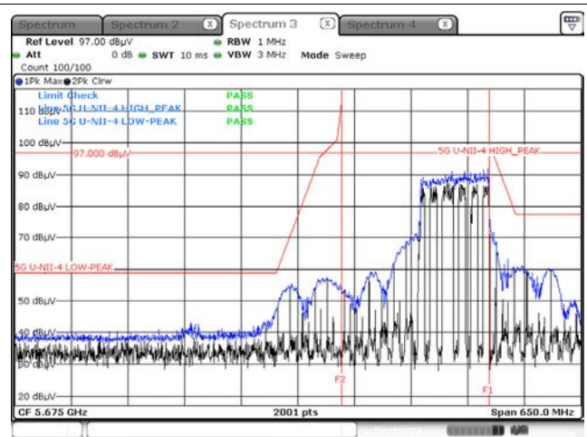
Peak result (802.11ax(HE160_80U) Ch.163, 996T RU 67)
