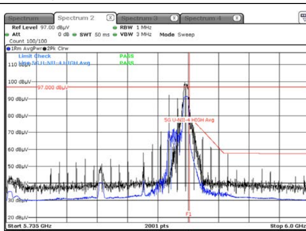
Average result (802.11ax(HE80) Ch.171, 52T RU 52)
