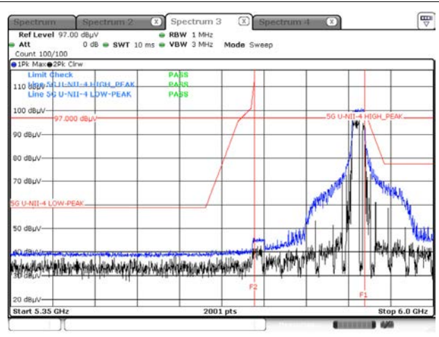
Peak result (802.11ax(HE20) Ch.177, 242T RU 61)
