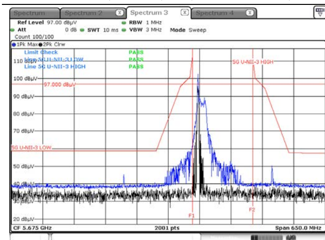
Peak result (802.11ax(HE20) Ch.149, 106T RU 53)
