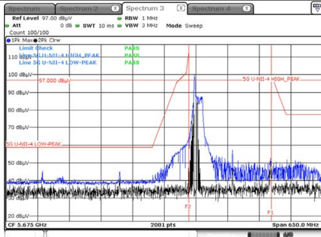
Peak result (802.11ax(HE160_80L) Ch.163, 106T RU 53)
