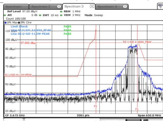
Peak result (802.11ax(HE40) Ch.175, 484T RU 65)
