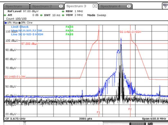
Peak result (802.11ax(HE40) Ch.159, 106T RU 56)
