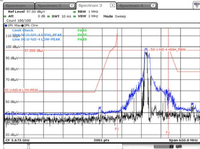
Peak result (802.11ax(HE40) Ch.167, 484T RU 65)
