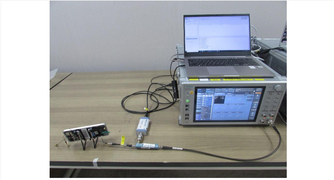
Test setup photo-1 TC01,03,04,05,07,08,09
