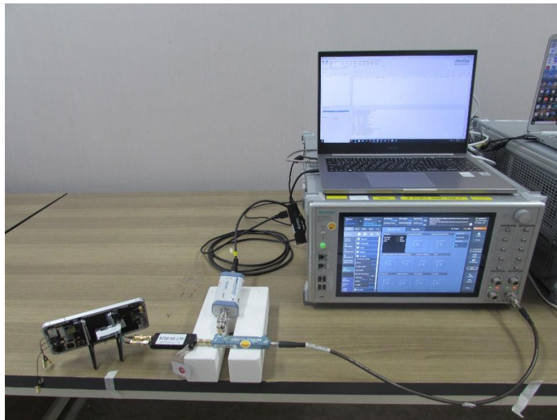
Test setup photo-4 TC11
