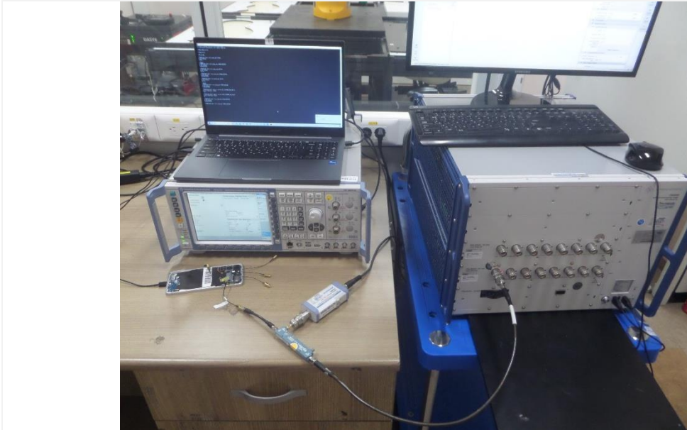
Test setup photo-7 W_TC 01,02,03
