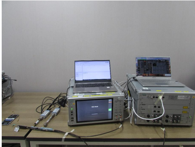
Test setup photo-5 TC12
