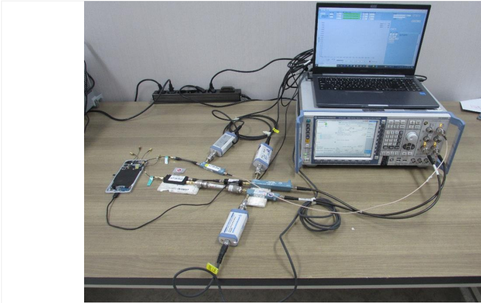
Test setup photo-8 C-TC01
