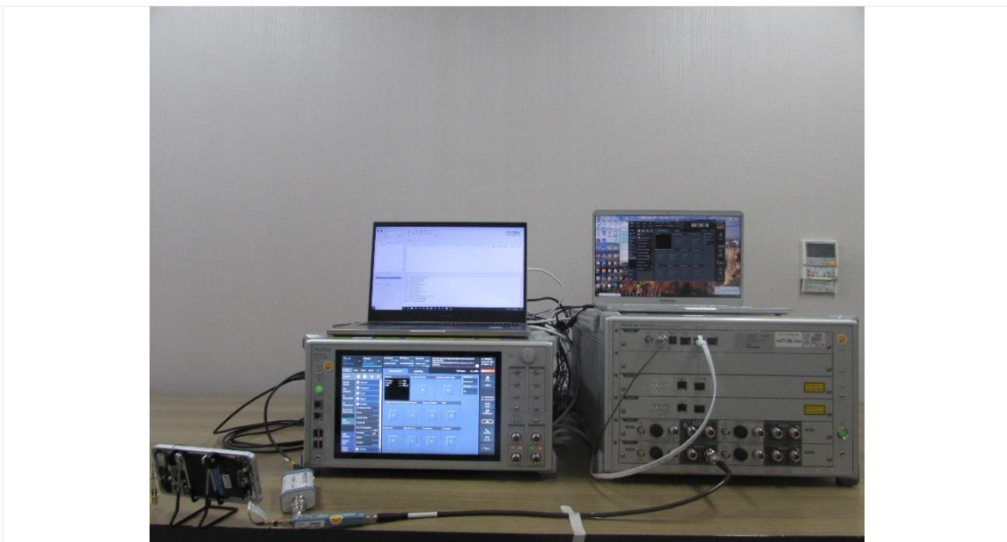
Test setup photo-2 TC02,06,13
