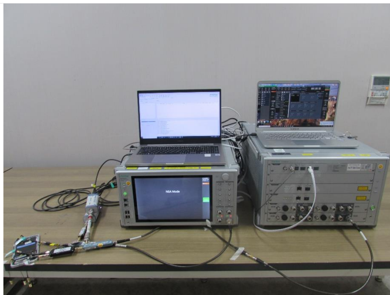
Test setup photo-6 TC14
