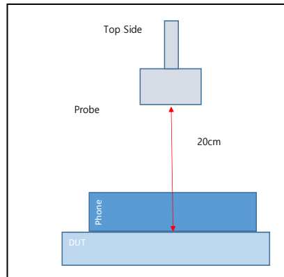
DUT to phone test Configuration 1 & 2
