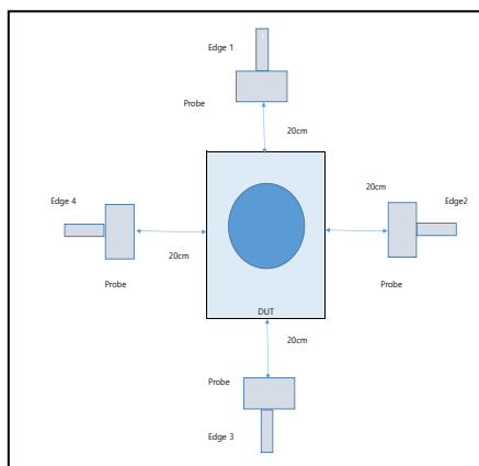
DUT to Watch/Ear buds test Configuration 5 & 6 and 7 & 8
