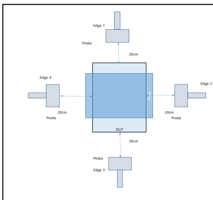
DUT to phone test Configuration 3 & 4
