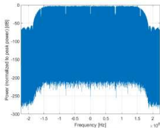
Frequency Domain
