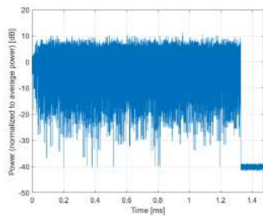
Time Domain
