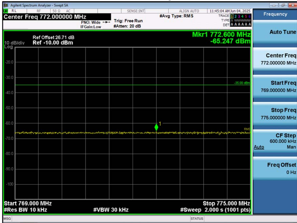
LTE B14_5 M_Extended Band Edge_Low_QPSK_1RB
